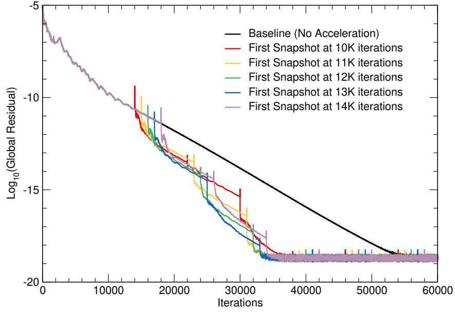
Figure 43: Comparison of the convergence history of the primal harmonic balance solver accelerated with the reduced-order model-base acceleration technique.
