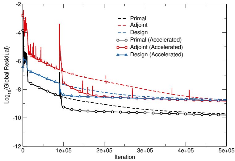
Figure 89: Convergence history of the primal, adjoint, and design equations solved via a one-shot optimizer with a single application of the reduced-order model acceleration technique.
