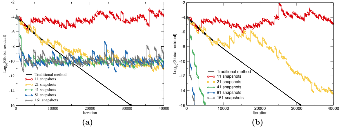
Figure 48: Multiple applications of the convergence acceleration technique (a) using double precision reaches an artificial convergence limit but (b) using quadruple precision eliminates this limit.
