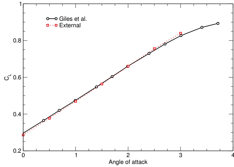
Figure 27: Lift coefficient for varying angles of attack over RAE 2822 at M = 0.725 and Re = 6.5 \times 10^6
