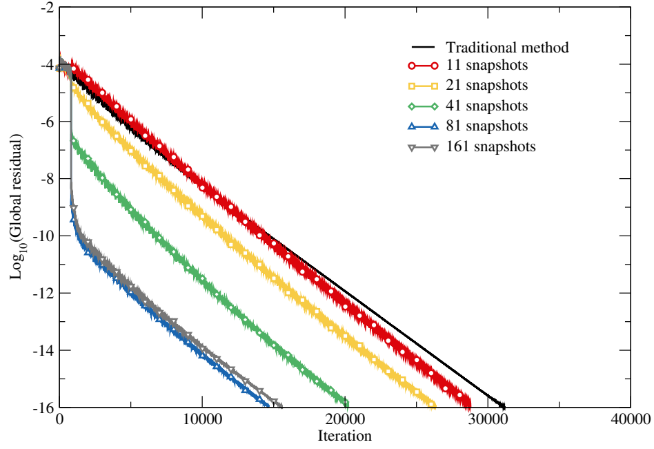
Figure 45: Convergence history achieved by varying snapshot count: increased snapshot quantities improve convergence acceleration
