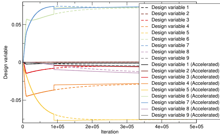
Figure 90: Design variable history for the one-shot optimizer with a single application of the reduced-order model acceleration technique.
