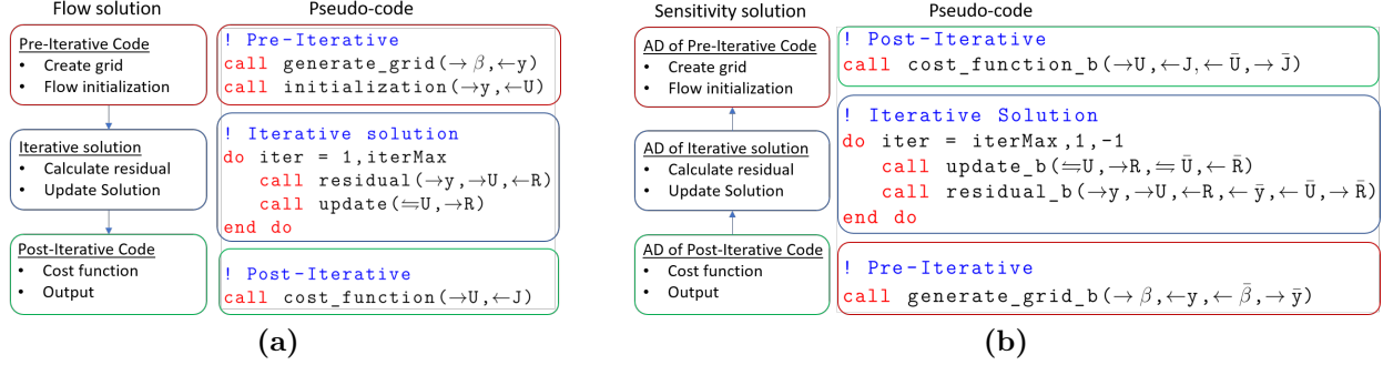
Figure 18: (a) Pseudo-code for the forward pass and (b) Pseudo-code for the reverse pass using brute force AD. Adapted from Christakopoulos et al. [27].
