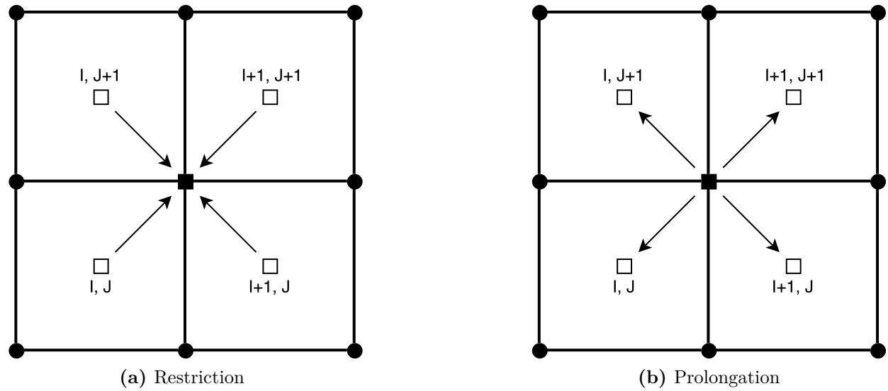
Figure 9: Cell-centered multigrid (a) Restriction and (b) Prolongation. Here \square are the centers of the fine grid and \blacksquare is the center of the coarse grid.
