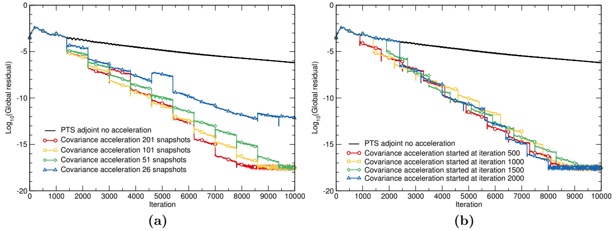
Figure 70: Comparison of the convergence history of the primal time-stepping adjoint accelerated with reduced-order models built using: (a) different snapshot quantities, and (b) varied initial snapshot collection iterations.
