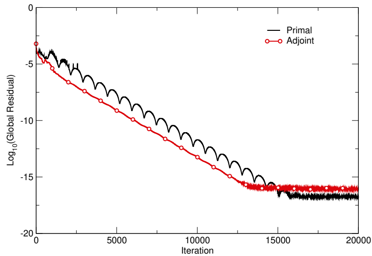
Figure 83: Convergence history of the primal, brute-force adjoint, and time-stepping adjoint sensitivity approach for the initial nozzle design.
