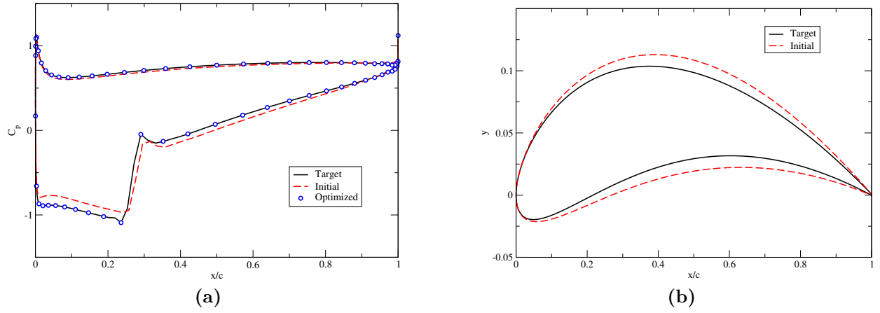
Figure 61: The initial, target and optimized (a) surface pressure distribution and (b) blade shape
