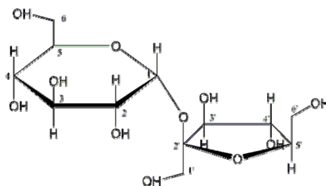
Sucrose: \beta -D-fructofuranosyl- \alpha -D-glucopyranoside
