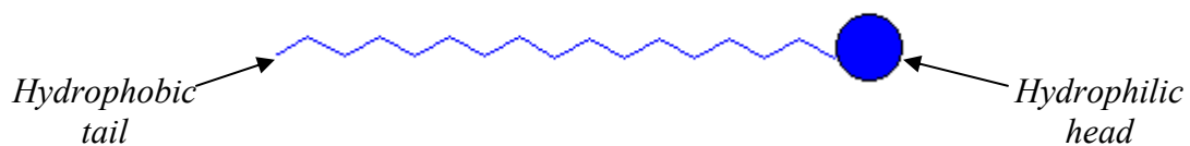
Figure 1.1: Structure of a surfactant
