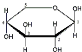
Xylose: \beta -D-xylopyranose
