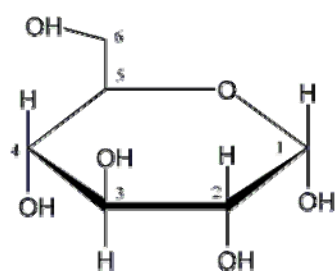
Glucose: \alpha -D-glycopyranose (most abundant form for crystalline reagent; in water, present at 33%, with 67% \beta -D-glucopyranoside)
