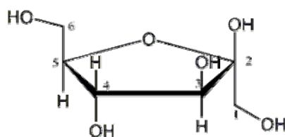
Fructose: \beta -D-fructofuranose (typical form when part of disaccharide or polymer; 33% in water)
