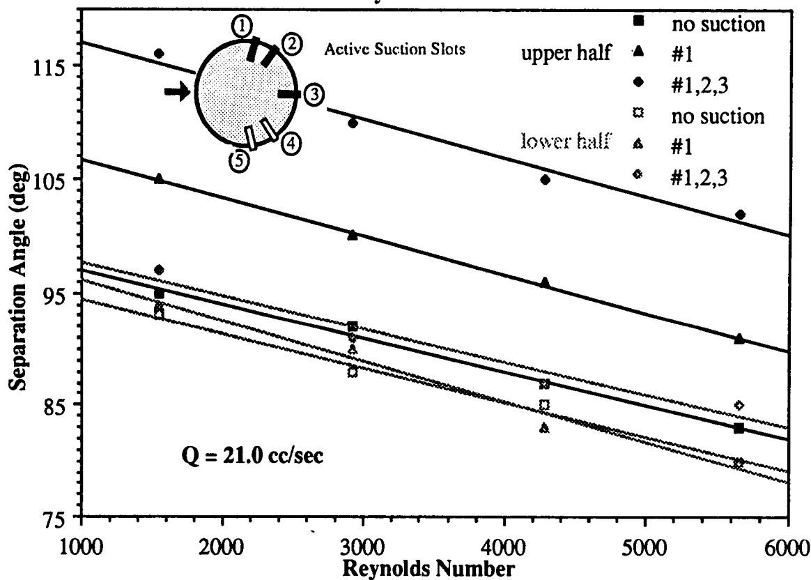
Figure 3.8 \theta vs. Re_D for suction through slots #1 and 1, 2, 3 at Q = 10.5 \text{ cc/sec} and 21.0 \text{ cc/sec}
