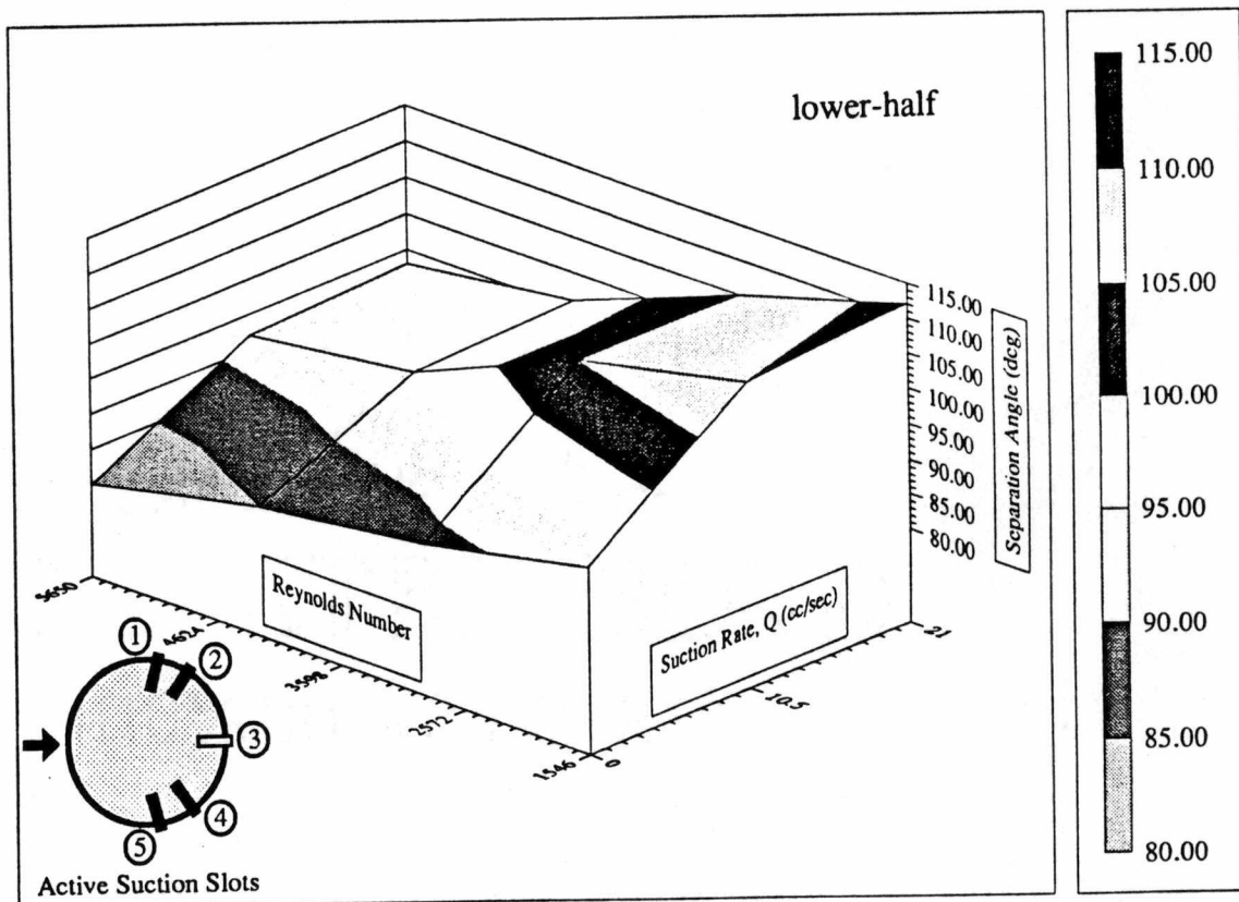
Figure 3.5 \theta vs. Re_D and Q : suction through slots #1, 2, 4, 5
