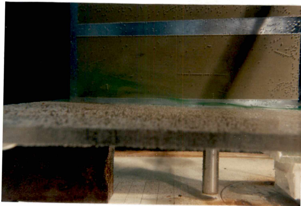
Figure 3.20 Top and bottom views of the flowfield with no suction applied for \beta = 6^\circ ( V_\infty = 8.91 cm/sec, Re = 16060 )
