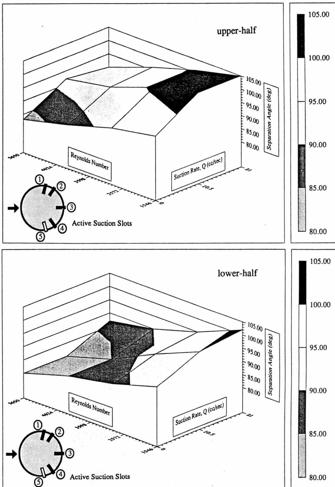
Figure 3.3 \theta vs. Re_D and Q : suction through slots #1, 2, 3, 4
