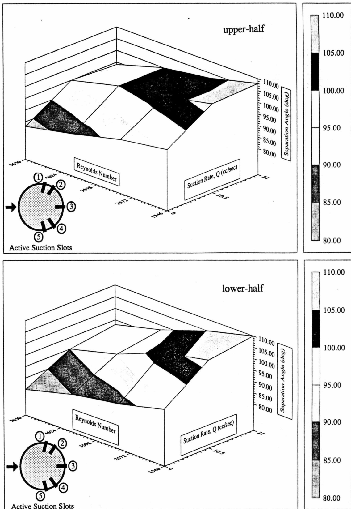
Figure 3.4 \theta vs. Re_D and Q : suction through slots #1, 2, 3, 4, 5
