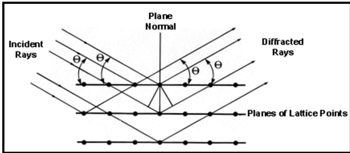
Figure 43. Figure showing the position for the incident and diffracted X-rays in XRD as well as the interaction angle of an ordered crystal
