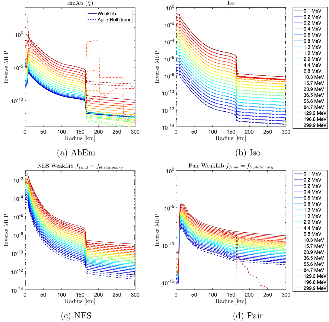
Figure 5.2.4: Opacity comparison between results obtained by WeakLib and Agile-Boltztran for Bruenn (1985) electron-neutrino interactions using the LS220 EOS and a 25 M_{\odot} 100 ms post-bounce profile.
