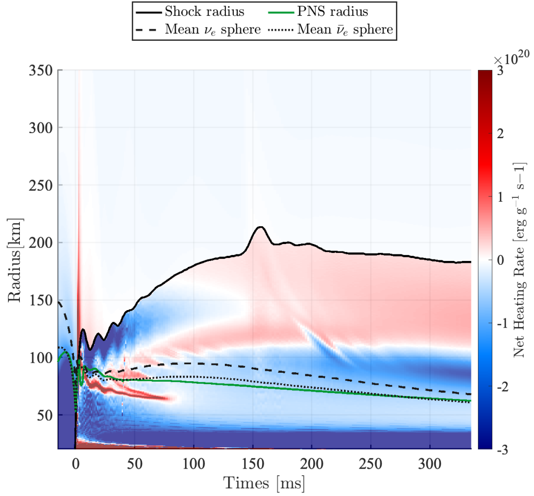
Figure 7.4.8: Net heating rates for model S10 as a function of radius and time. The black line tracks the shock position. The green line marks the PNS radius. The dashed black line and the dotted black line represent the mean electron-neutrino sphere and the mean electron-antineutrino sphere, respectively.
