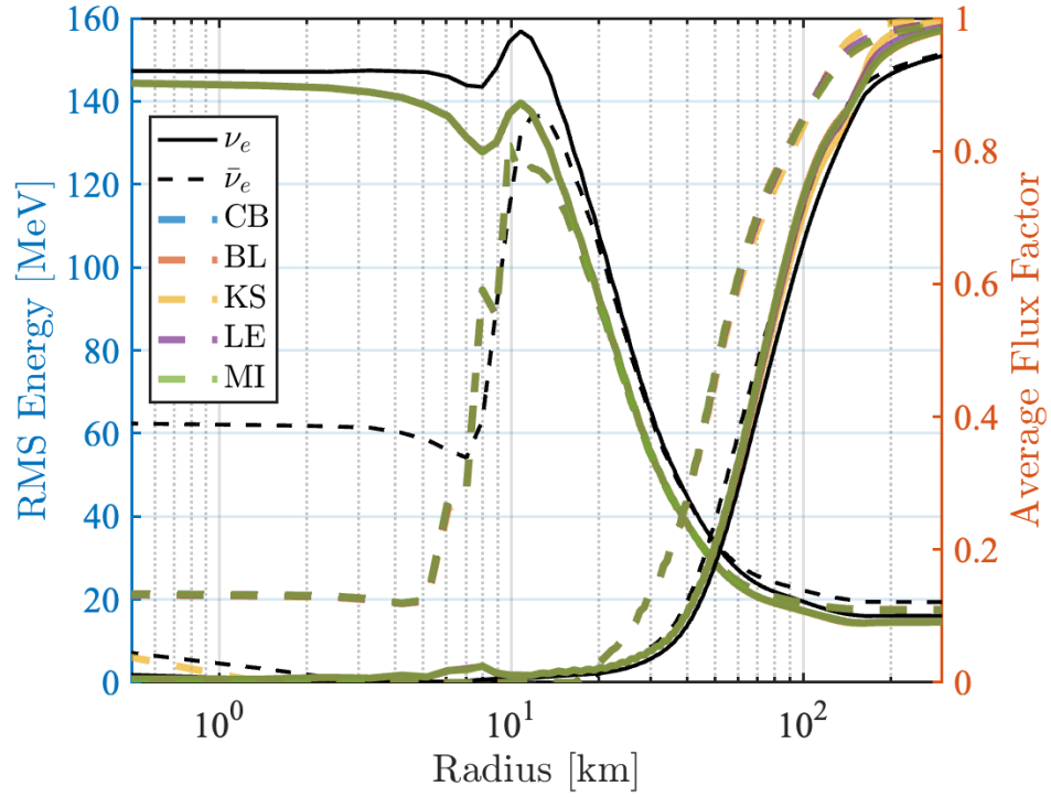
Figure 5.6.8: Steady radiation field with stationary fluid field in deleptonization problem for all closures. The black lines represent the initial (CHIMERA) state, and thornado results in color: the results of the CB closure are in blue, red for the BL closure, yellow for the KS closure, purple for the LE closure, and green for the MI closure.
