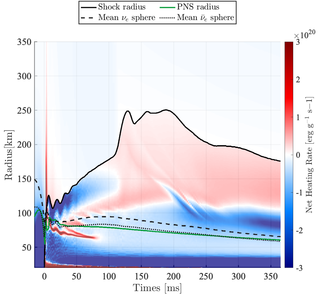
Figure 7.4.9: Net heating rates for model S11 as a function of radius and time. The black line tracks the shock position. The green line marks the PNS radius. The dashed black line and the dotted black line represent the mean electron-neutrino sphere and the mean electron-antineutrino sphere, respectively.
