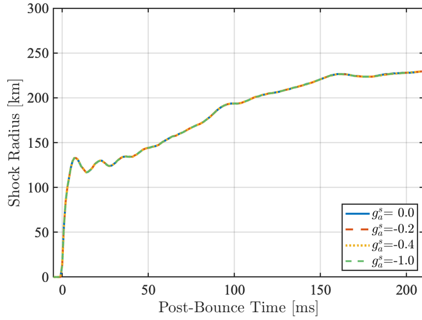
Figure 7.5.9: Comparison isoenergetic scattering opacity simulations in shock radii for model S9, with different g_a^s and g_a = 1.21 . The blue line marks the result for g_a^s = 0.0 , red for -0.2, yellow for -0.4, and green for -1.0.
