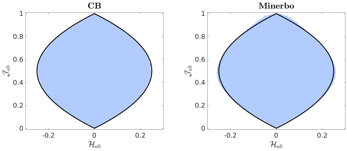
Figure 2.5.3: Illustration of \mathcal{M}_{ab} , as defined in Equation (2.117), computed with algebraic maximum entropy closures of Cernohorsky & Bludman (left) and Minerbo (right). In each panel, \mathcal{M}_{ab} was computed using the respective closure, using 10^6 random pairs (\mathcal{M}_a, \mathcal{M}_b \in \mathcal{R}) , and plotted as a light-blue point. The solid black lines mark the boundary of \mathcal{R} : \gamma(\mathcal{M}) = 0 . Published in Chu et al. (2019a) .
