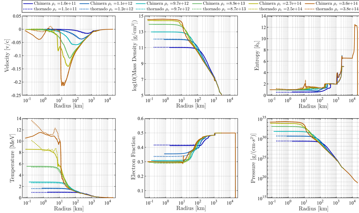
Figure 6.3.2: Comparison with CHIMERA in fluid quantities versus radius at certain snapshots during collapse, as the legend indicates. CHIMERA results are plotted with solid lines, while Flash-X + thornado results are plotted with dotted lines. Line color indicates different collapse times, as indicated by the central density.
