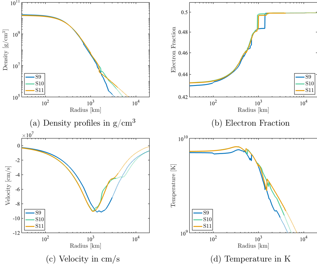
Figure 7.2.1: Initial conditions for the three low-mass progenitor models from Sukhbold et al. (2016). We used 3000 km with \Delta r = 0.73 km for S9, 3700 km with \Delta r = 0.72 km for S10, and 4000 km with \Delta r = 0.74 km for S11. The solid lines represent the initial condition in the computation domain, while the dotted lines are for the available data from Sukhbold et al. (2016).
