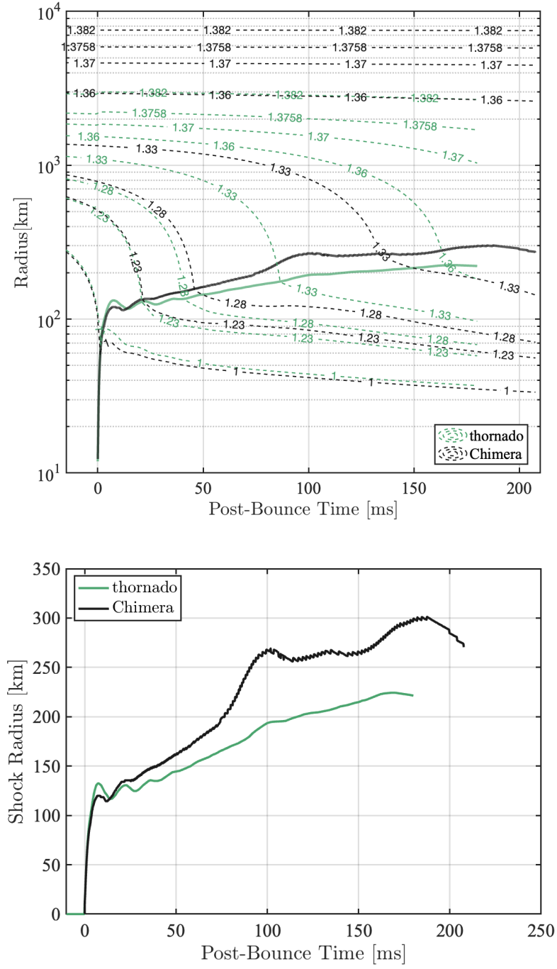
Figure 6.3.6: Comparison of CHIMERA and Flash-X + thornado shock radii (both panels) and mass shell trajectories (upper panel) as a function of time after bounce.
