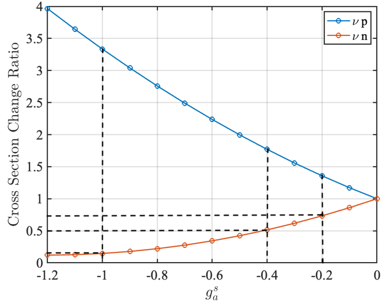
Figure 7.5.8: Following the definition in Melson et al. (2015b) , plots the ratio change in the total transport cross section Equation (7.6) versus g_a^s with g_a = 1.21 . Blue line marks the change in \nu p cross section, and red line for \nu n cross section. g_a^s = 0.0, -0.2, -0.4 , and -1.0 , corresponding to that \nu n decreasing ratio (defined by Equation (7.7) with -g_a ) be 1.0(no change), \sim 0.73 , \sim 0.51 , and \sim 0.15 , respectively.
