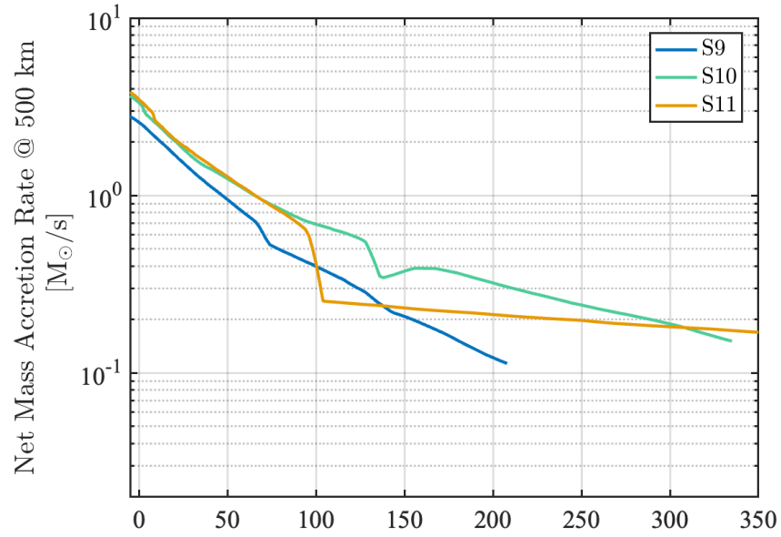
Figure 7.4.2: Accretion rates for three models considered here. Blue line marks result for S9, while green line for S10, and yellow line for S11.
