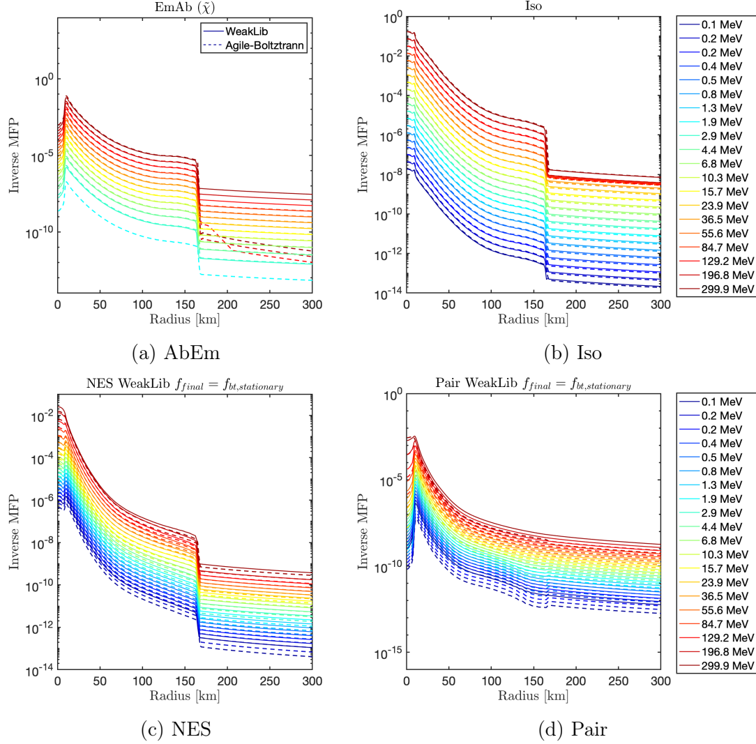
Figure 5.2.5: Opacity comparison between results obtained by WeakLib and Agile-Boltztrann for Bruenn (1985) electron-antineutrinos interactions using the LS220 EOS and a 25 M_{\odot} 100 ms post-bounce profile. Same as Figure 5.2.4 but for electron-antineutrinos.
