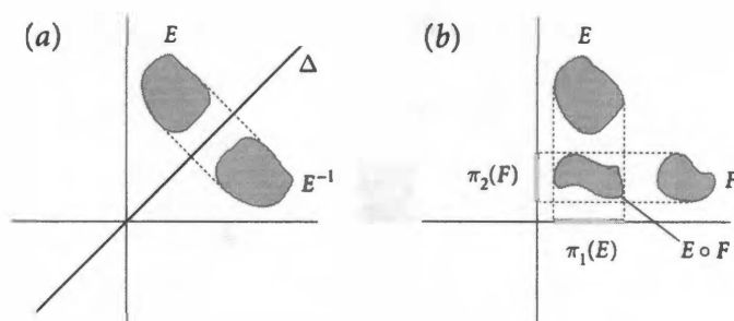
Figure 2.2: Inverses and products of subsets of X \times X . (a) The inverse E^{-1} of a subset E of X \times X . (b) The product E \circ F is a subset of projections of E and F .
