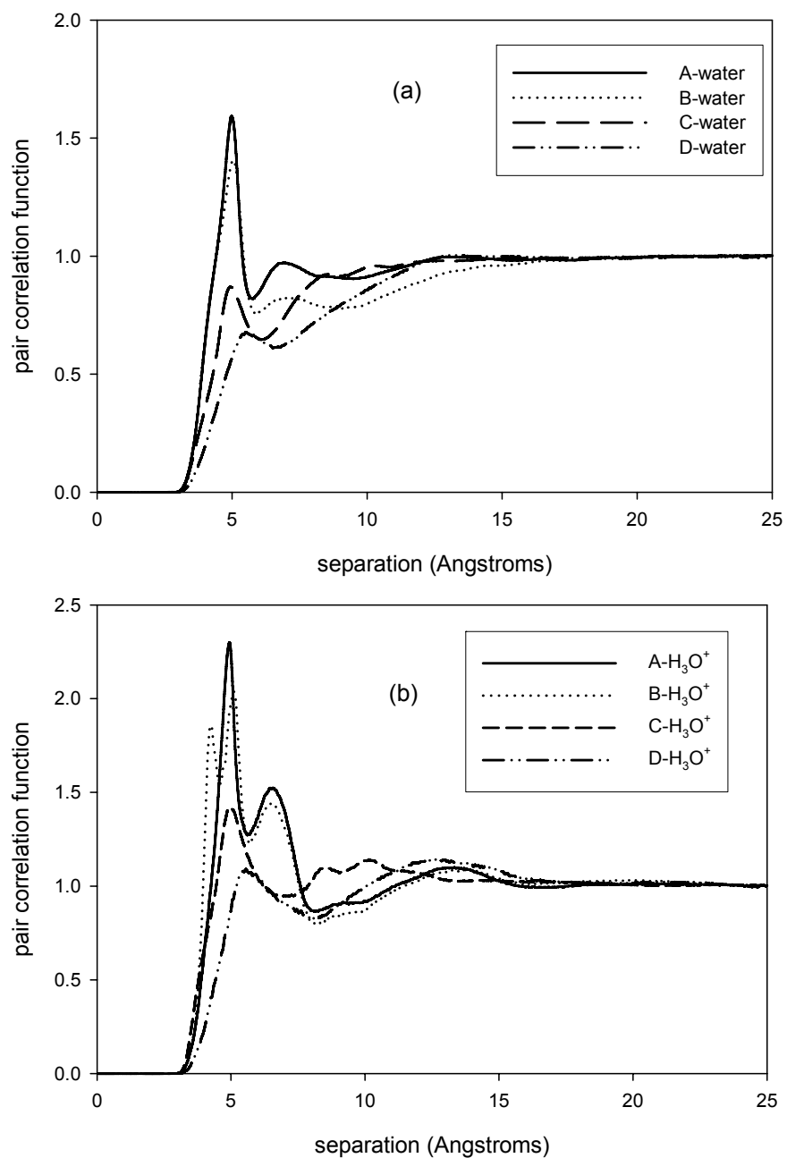
Figure 7.4. PCFs for CG beads involved in (a): polymer-water interactions and (b): polymer- \text{H}_3\text{O}^+ interactions.
