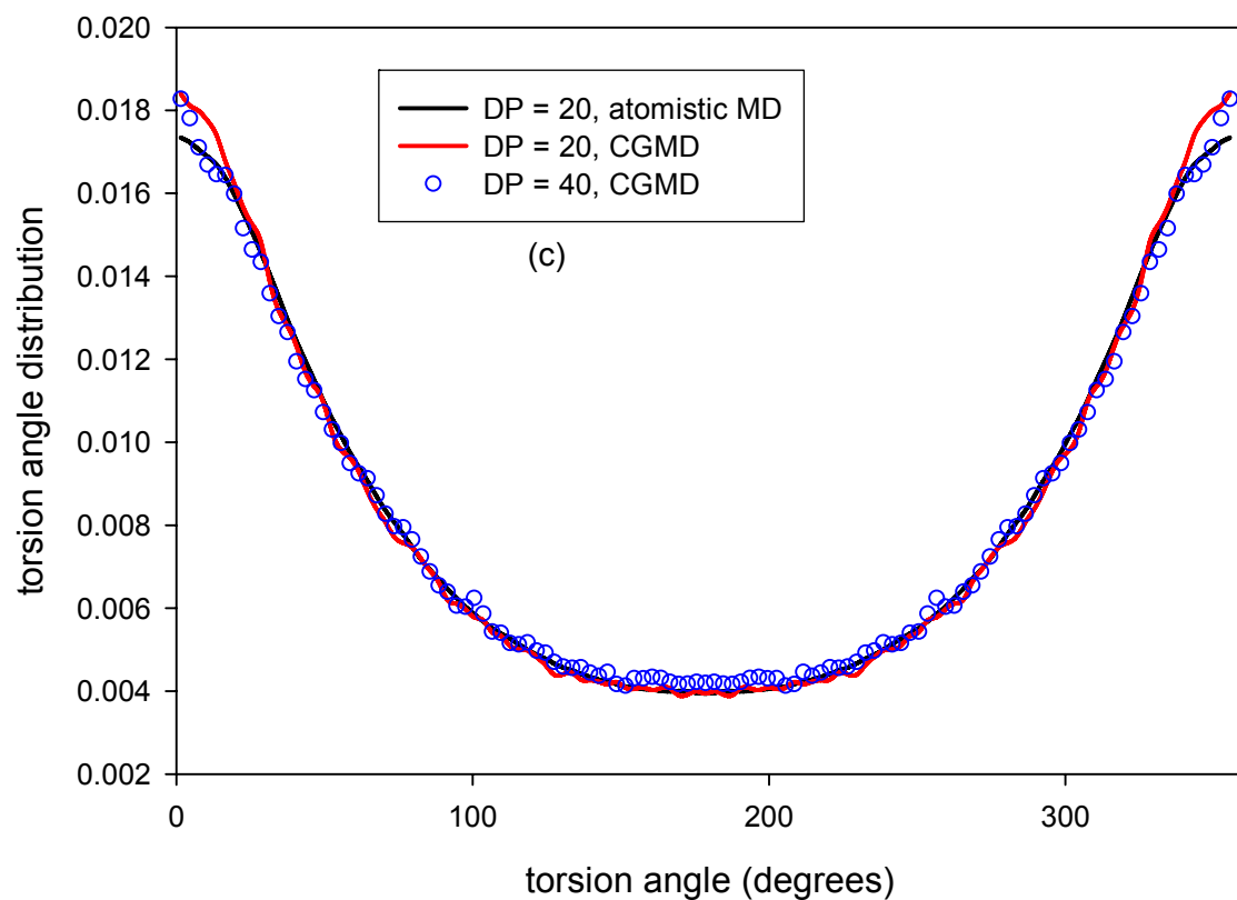
Figure 5.2. Bonded probability distribution functions for CG beads of PEG from atomistic MD simulations (DP=20) and CGMD simulations (DP=20 and 40). (c) Torsion. The GCMD simulations used the potentials from the OZPY -1 +IBI method.
