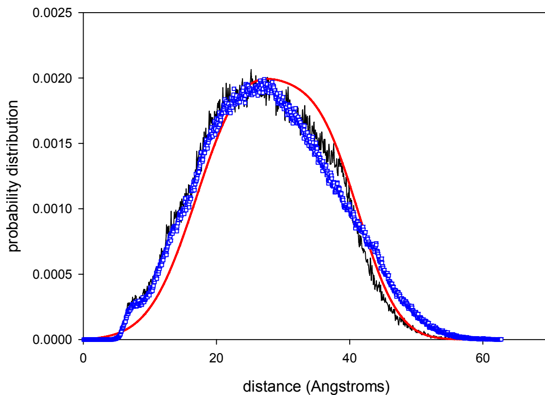
Figure 6.8. Comparisons of the chain end-to-end distance probability distributions for sxPCHD systems from atomistic MD (two chains cross-linked system: red line) and CGMD (two chains cross-linked system: black line, three chains cross-linked system: data points) simulations.
