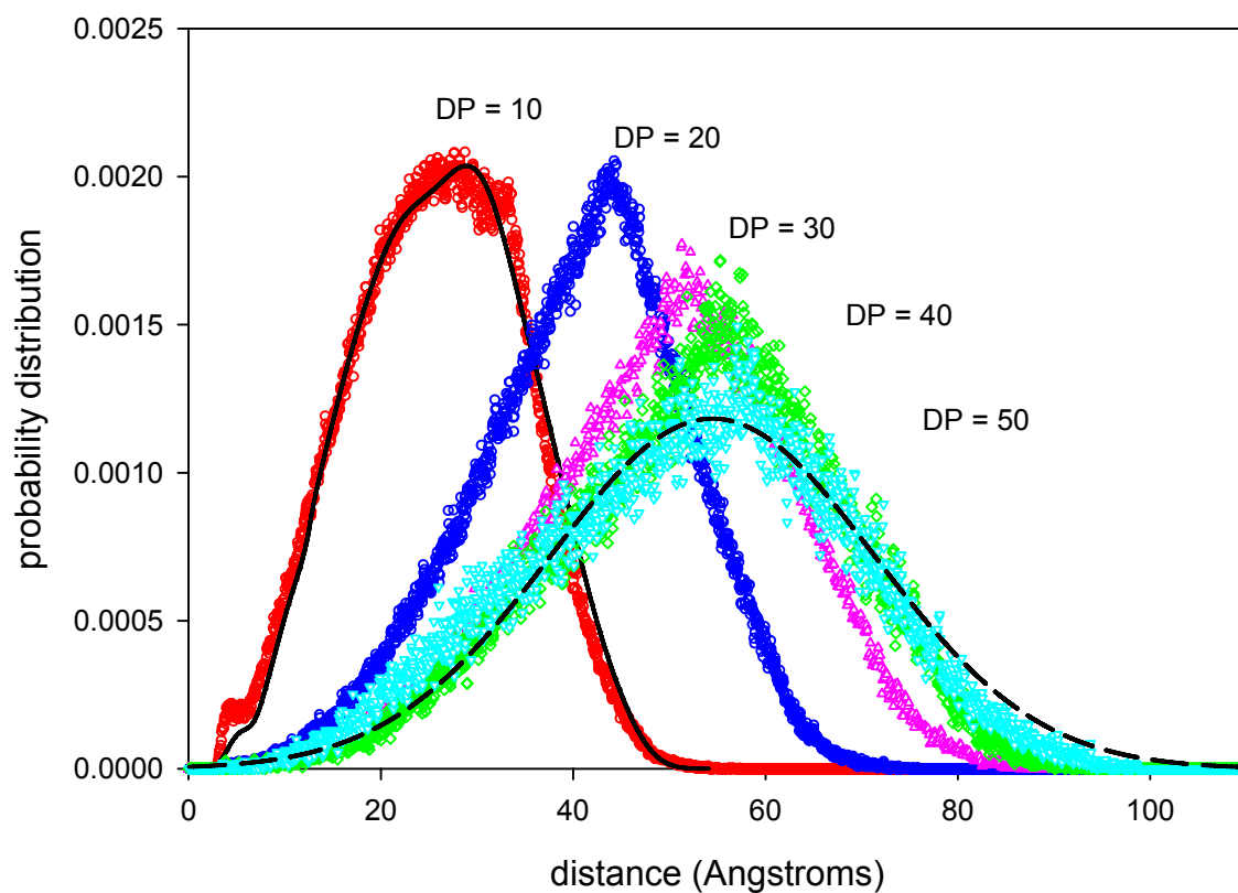
Figure 4.7. Comparisons of the chain end-to-end distance probability distributions for DP = 10, 20, 30, 40 and 50 from CGMD. For DP = 10, the solid line represents the distribution from atomistic MD simulation; For DP = 50, the dash line represents the distribution predicted by Gaussian function.
