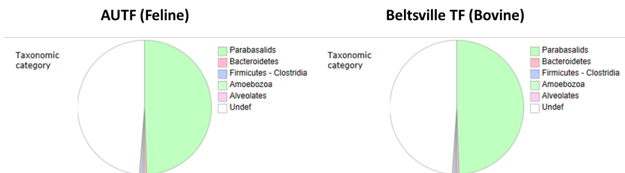
Figure 15. Taxonomic Information for Best BLAST hits for Two T. foetus Genomes. The top 5 sources of best BLASTp hits from taxa were chosen for this figure. After Parabasalids, Bacteroidetes (a phylum rich in pathogenic bacteria) was the next highest source of hits with close to 100 sequences represented.
