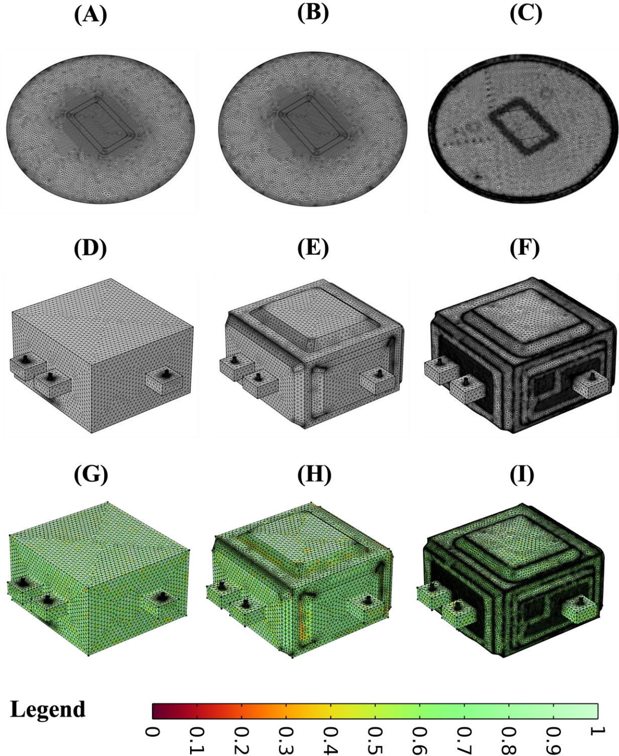
Figure 2.5 Modeling geometries and their corresponding mesh with three types of details: simple box (A & D), manually measured (B & E), and 3-D scanned (C & F) for turntable (A, B, & C) and oven (D, E, & F) and the mesh quality of the three different geometries (G, H, & I)
