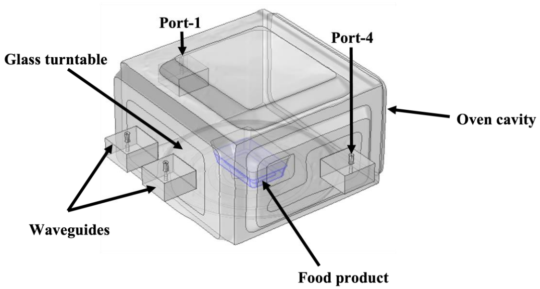
Figure 3.2 A detailed schematic diagram of the multiple-port microwave oven cavity.
