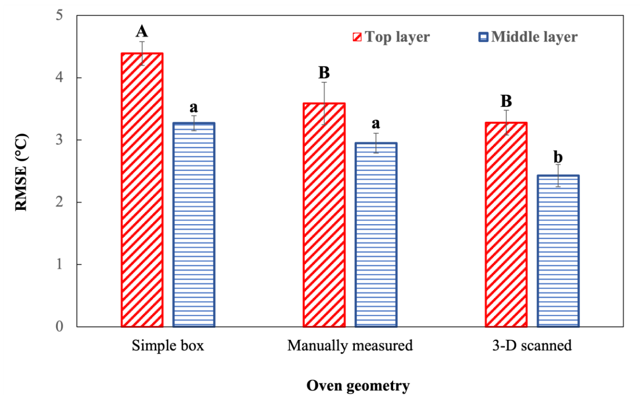
Figure 2.8 Comparison of the RMSE values* between the simulated temperature profiles of the different geometries with the experimental temperature profiles for the top and middle layer at 2.45 GHz using port 1.
