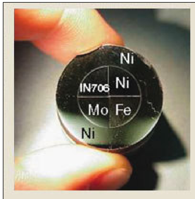
Figure 2 : Zhao's "diffusion multiple" of Ni, Fe, Mo, and Inconel-706
