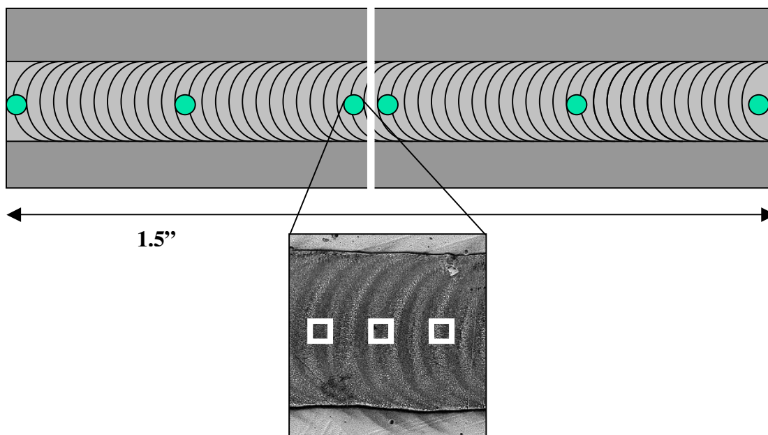
Figure 27 : Schematic showing EDS measurements for samples with Cr films on Ni substrates.
