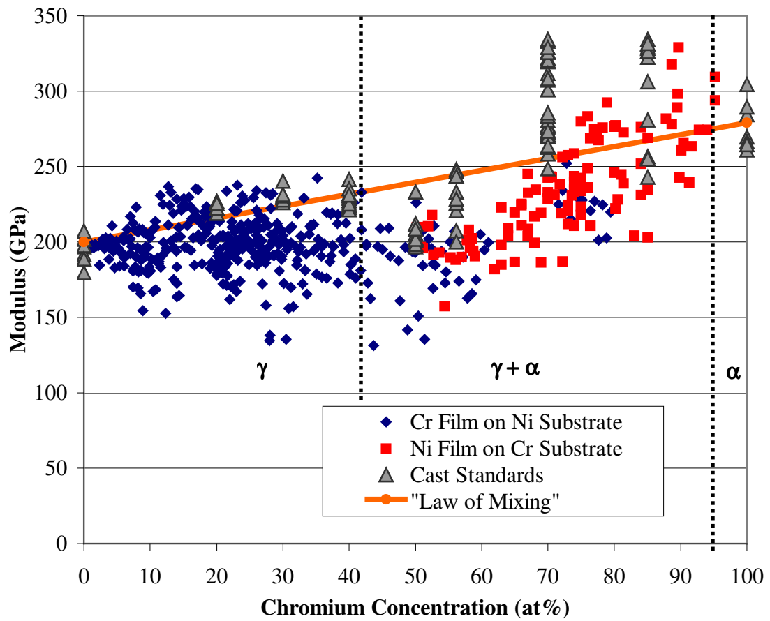
Figure 51: Modulus of all combinatorial EB welds.
