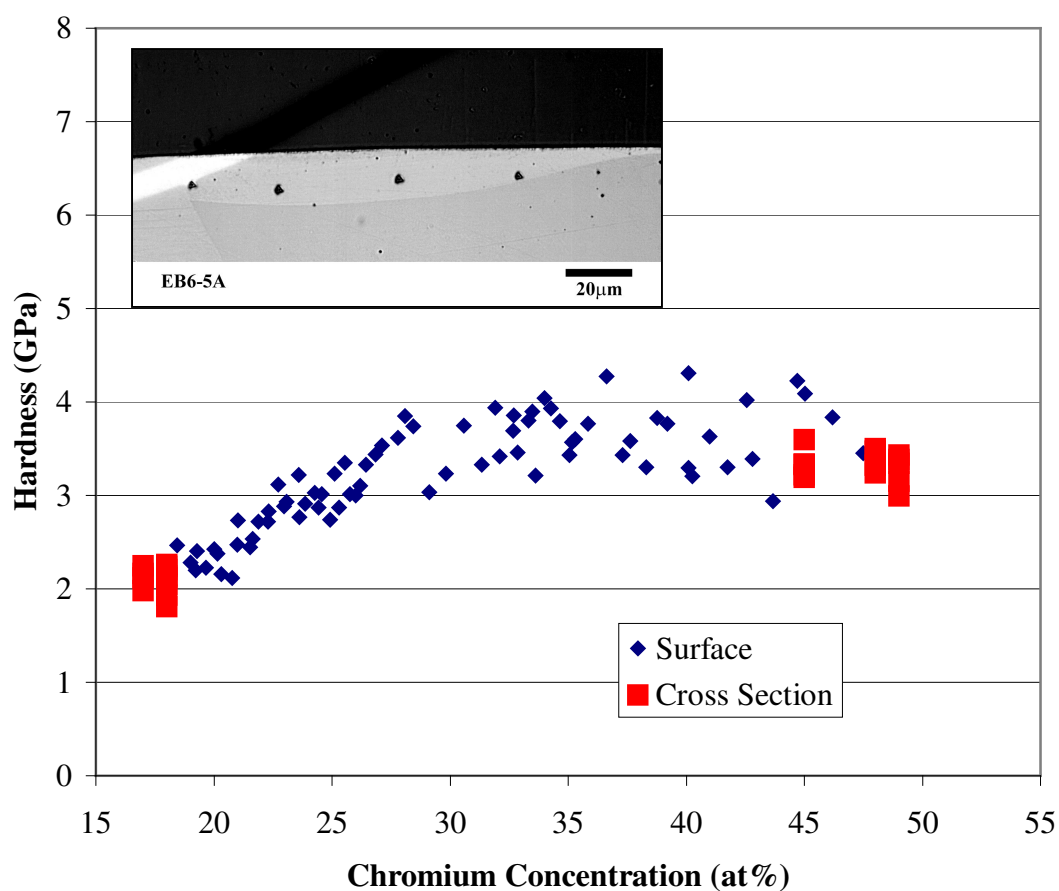
Figure 31: Hardness values for indents taken at surface compared to those taken from polished cross sections at either end.
