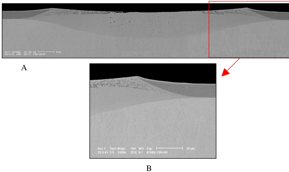
Figure 22: BSE images of a weld cross section; A) full weld pool, and B) edge of same weld at higher resolution (concentration of about 44 at% Cr).
