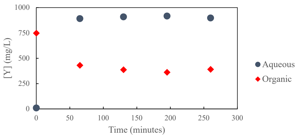
Figure 4B: Trial 12 – Yttrium Concentrations in Mixer-Settler Exit Streams vs Time ( E = 0.1\text{ M} , 60% Recycle)
