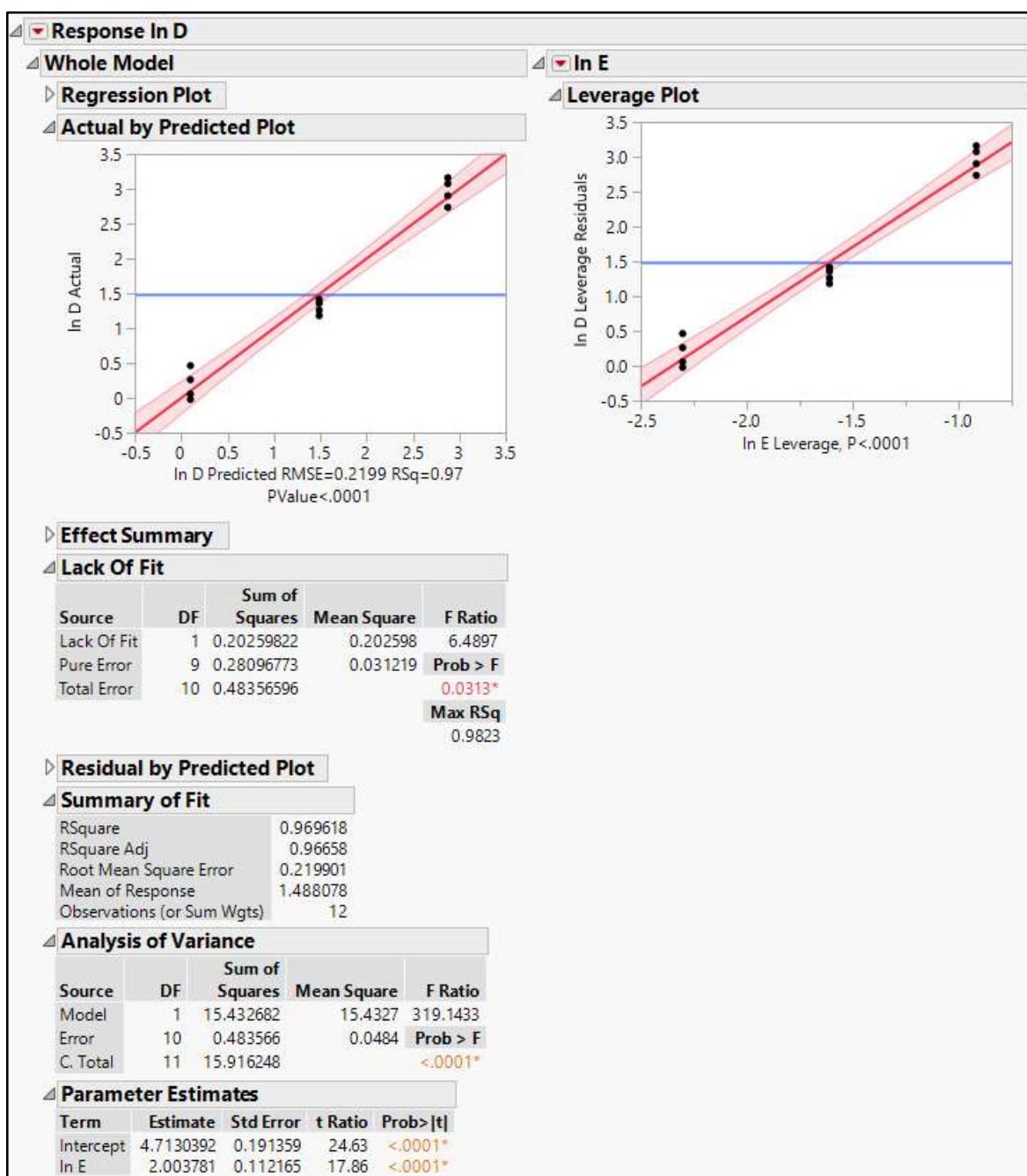
Figure 15: Model of Distribution Coefficient as Function of Extractant Concentration for Yttrium Extraction by DEHPA
