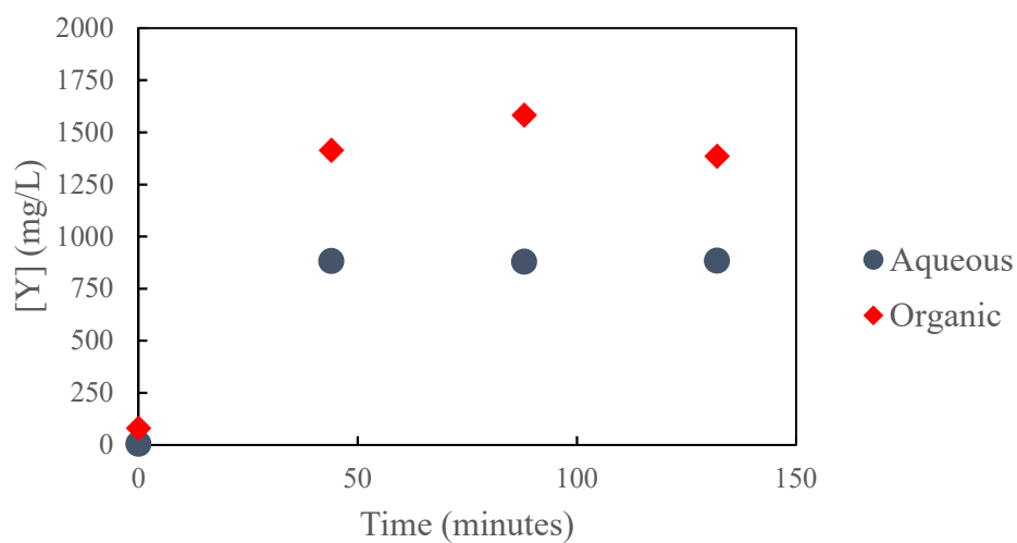
Figure 4A: Trial 4 – Yttrium Concentrations in Mixer-Settler Exit Streams vs Time ( E = 0.2\text{ M} , 0% Recycle)
