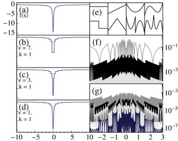
Figure 3.2: The function f to be approximated is in (a). Panels (b) - (d) show function refinement at k = 1 with successively smaller numerical thresholds ( \epsilon ). In (e) the first four scaling functions from Eq. 3.10 are shown above their corresponding wavelet from Eq. 3.11. The absolute value of the refinement error in is shown in (f) with k = 1 and \epsilon = 10^{-1}, 10^{-3}, 10^{-5} and in (g) with \epsilon = 10^{-5} and k = 1, 2, 3, 6 .
