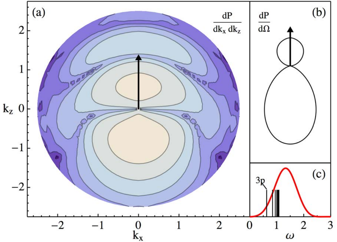
Figure 5.8: (Color online) (a) The fully differential photoionization momentum distribution of \text{Li}^{2+} and (b) angular distribution dP/d\Omega from Eq. 3.32 are shown against the laser polarization access (the arrow). (c) The transition energies from the initial 2s state are superimposed on the laser's power spectrum.
