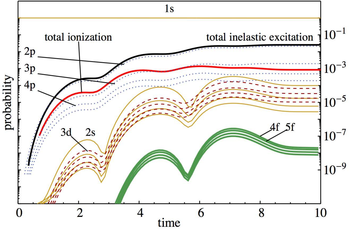
Figure 5.5: (Color online) The total ionization probability, total inelastic excitation probability Eq. (4.3), and selected bound state probabilities |\langle \psi_{n\ell 0} | \psi(t) \rangle|^2 of He + are plotted versus time. Due to azimuthal symmetry, m=0 .
