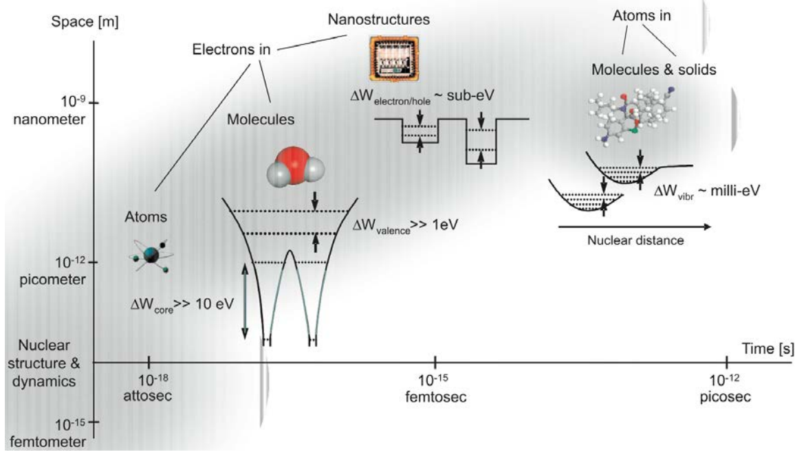
Figure 1.8: (from Krause and Ivanov [32]) Characteristic length and time scales in matter.
