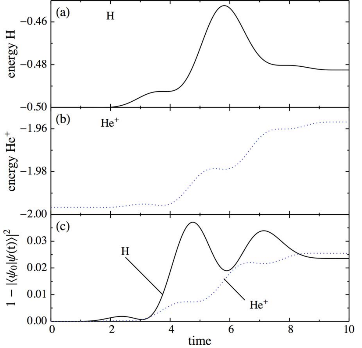
Figure 5.4: (Color online) The energy \langle \mathcal{H} \rangle from Eq. (2.21) and total inelastic excitation from Eq. (4.3) for He + and H are shown as a function of time.
