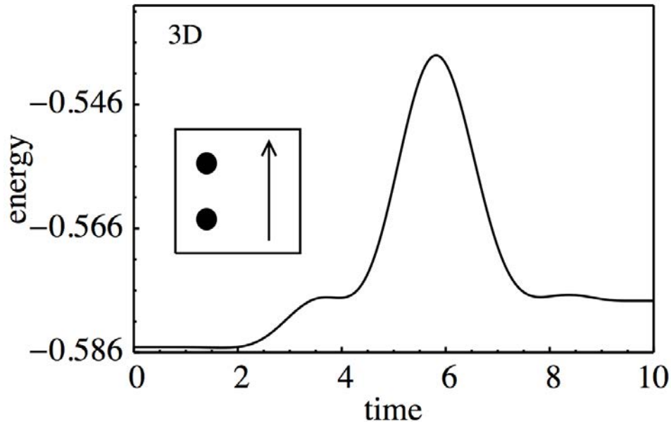
Figure 7.2: The energy \text{H}_2^+ whose internuclear axis is aligned parallel to the laser field polarization as shown by the inset.
