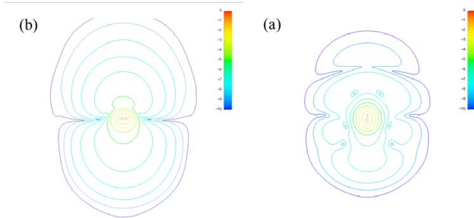
Figure 7.3: Isosurfaces of the probability density are shown at the end of the attosecond laser pulse for \text{H}_2^+ oriented (a) parallel and (b) perpendicular to the field polarization.
