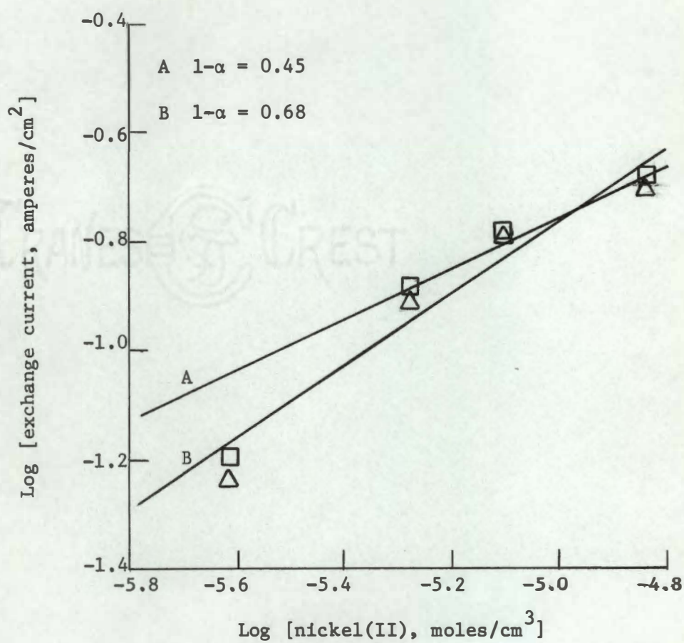
Figure 13. Plot of log [exchange current] versus log [nickel(II)].
