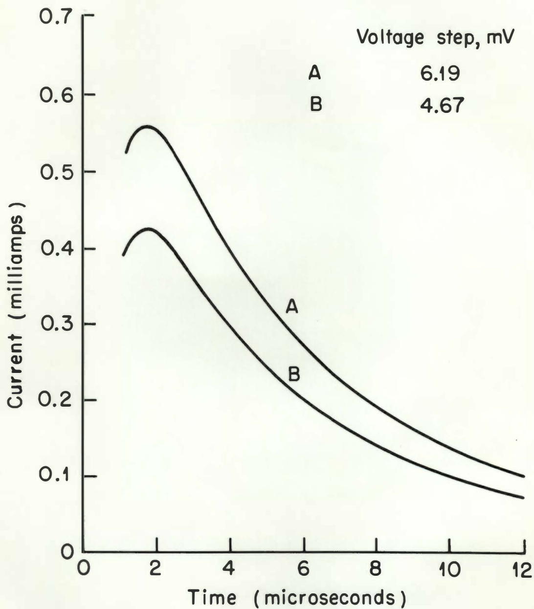
Figure 9. Charging current-time curves obtained by the voltage-step method in \text{LiF-BeF}_2\text{-ZrF}_4 at 500^\circ .
