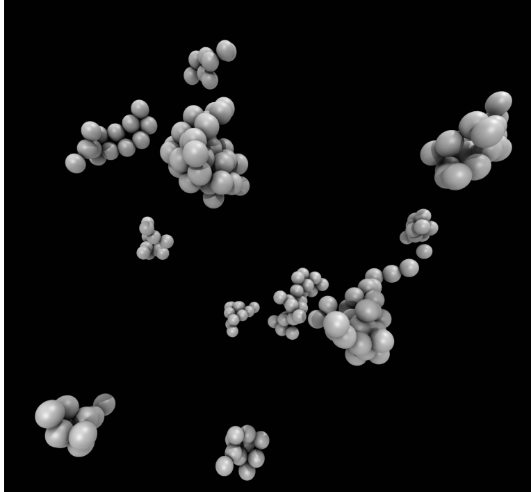
Figure 2.10: Loss of directionality upon introduction of random defects on structure formation for a = 5.5 nm and C_s = 1 mM. Values in the last row are surface charge density ( e/\text{nm}^2 ) and values in the first column are normalized magnitudes of polar vector.
