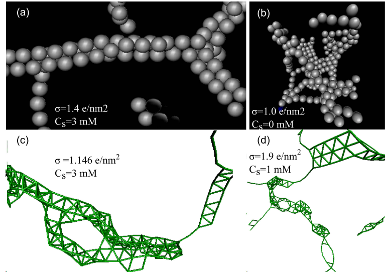
Figure 2.8: Formation of porous structures and elongated chain assemblies at higher concentrations (volume fraction is 0.1 for (b) and 0.01 for all other snapshots). a = 6.2 \text{ nm} , r_{sur.ch.} = 0.6 \text{ nm} for (b) and a = 5.5 \text{ nm} , r_{sur.ch.} = 2.5 \text{ \AA} for (a), (c) and (d).
