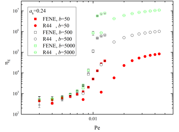
(f) FENE and R44, all b s, with HI and EV
