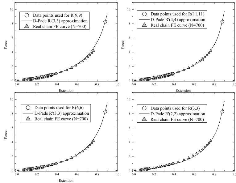
Figure 3.18: Various D-Pad  approximations. In general, accuracy increases with increasing initial polynomial order and sampling data points from all regions. The coefficient of each approximation is shown in Table 3.2.
