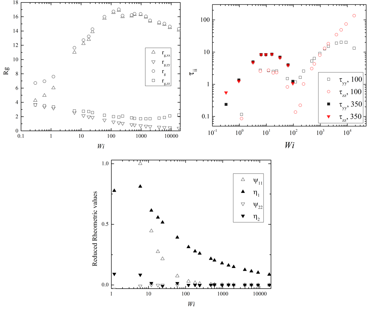
Figure 5.9: Diagonal components of the radius of gyration tensor (a) and the corresponding stress tensor components(b). Despite the growth of stress diagonal components in gradient and neutral direction, the second normal stress coefficient remains about zero.
