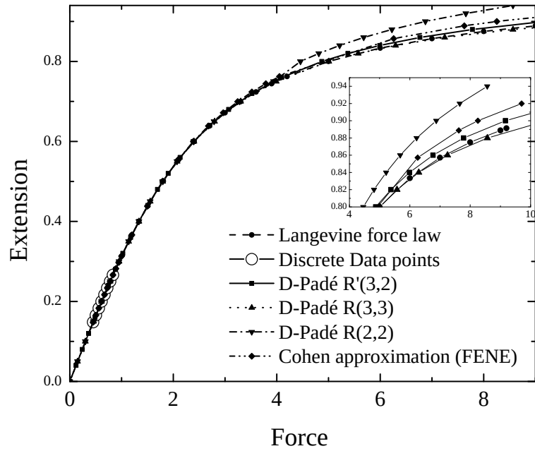
Figure 3.17: Validating the D-Pad  approximation method with known functions. Inset shows relative accuracy at the finite extensibility region.
