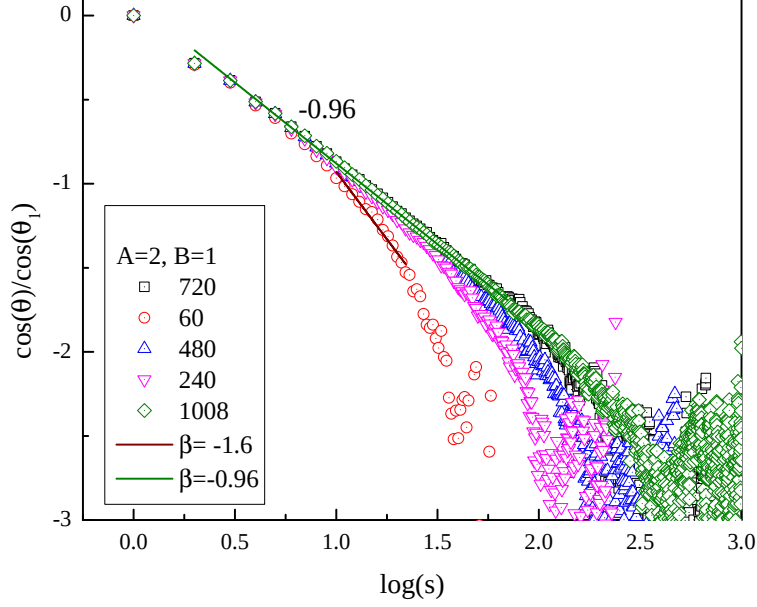
Figure 3.8: Normalized bond autocorrelation function along the chain in Athermal solvent. Note that for the small chain ( n = 61 ) the intermediate scaling region is absent and for large n curves reach a universal behavior.
