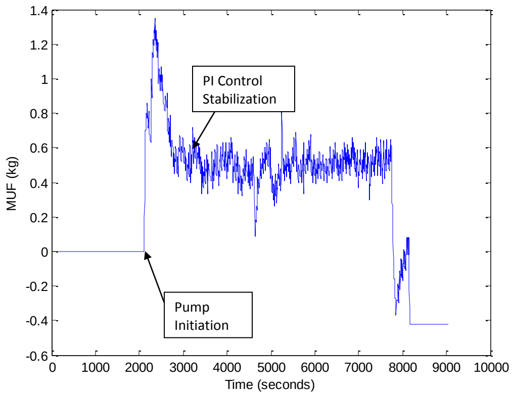
Figure 12 - PI Control Stabilization and MUF Calculation
