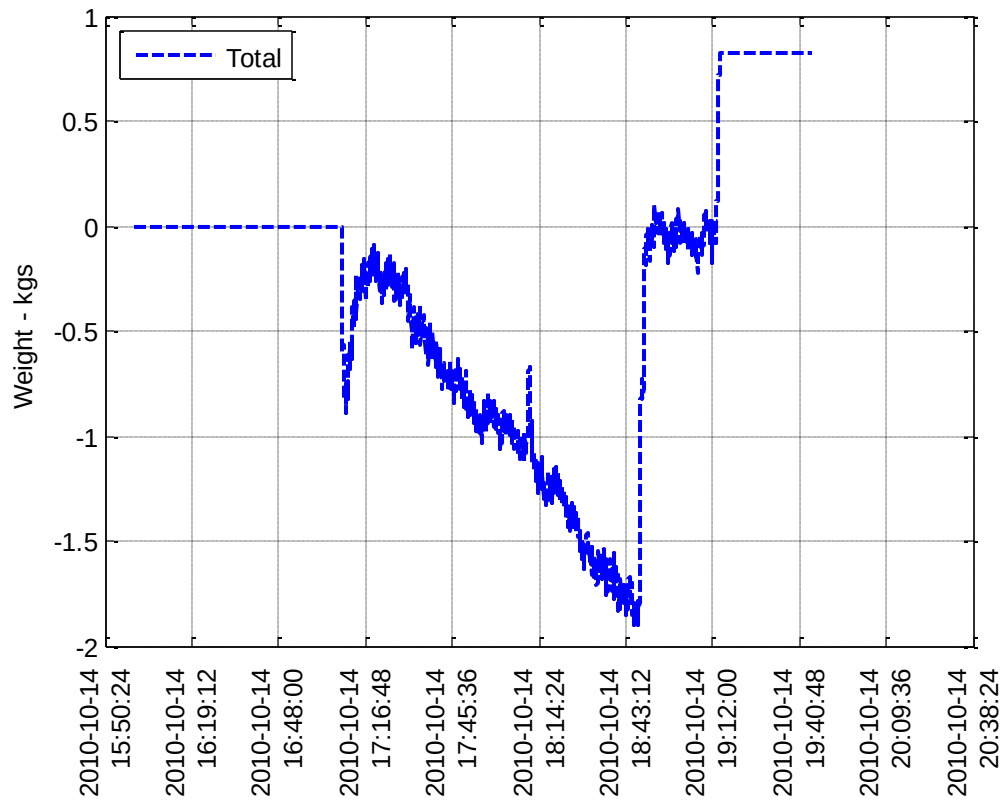
Figure A24 - Cumulative Inventory Difference for Fast Diversion
