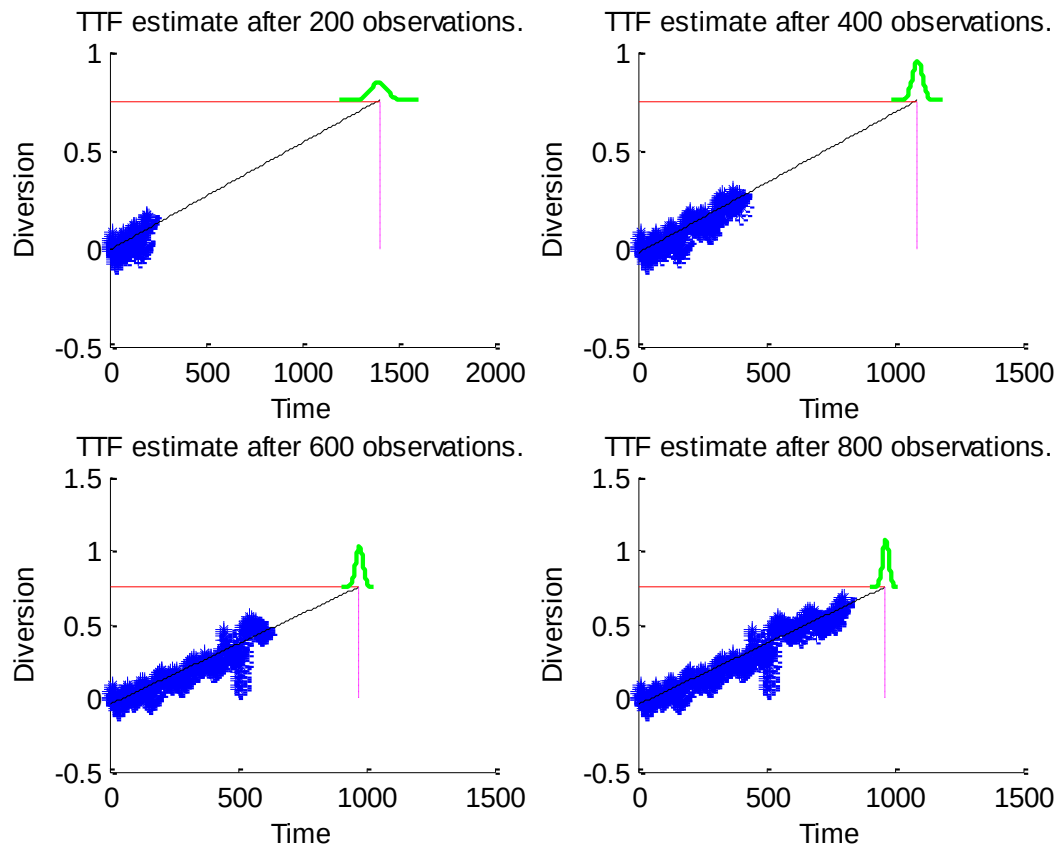
Figure 27 - General Path Model Predictions for Diversion
