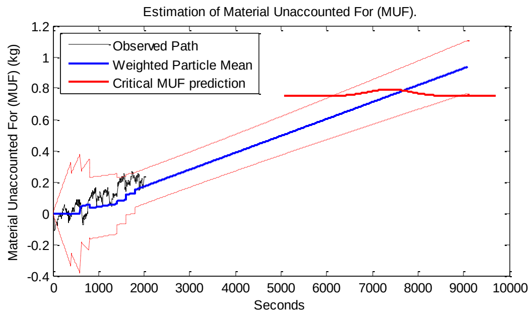
Figure 30 - Particle Filter Prediction at 33 Minutes, 20 Seconds
