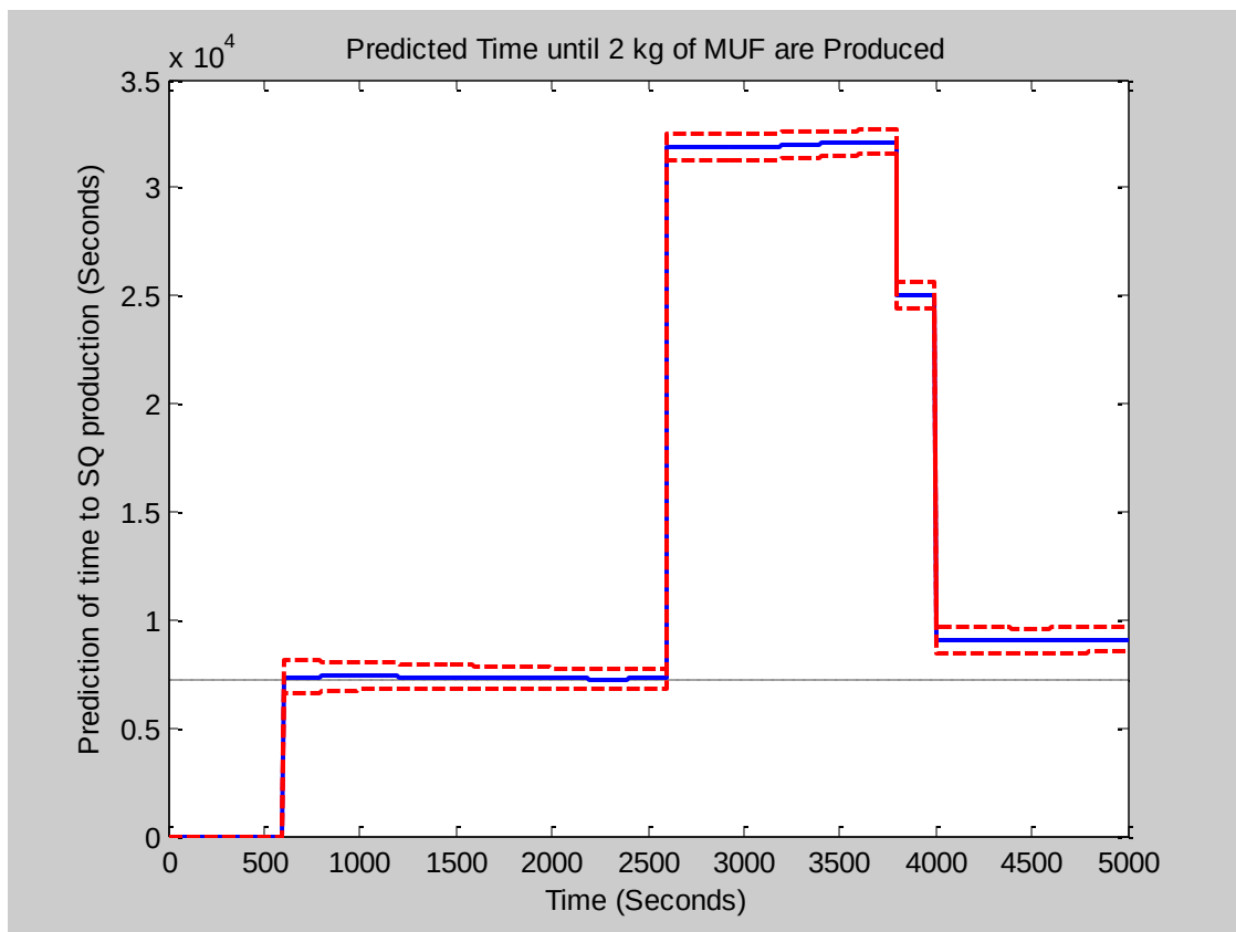
Figure 43 - Predictions of Significant Quantity Prediction for Fast Diversion
