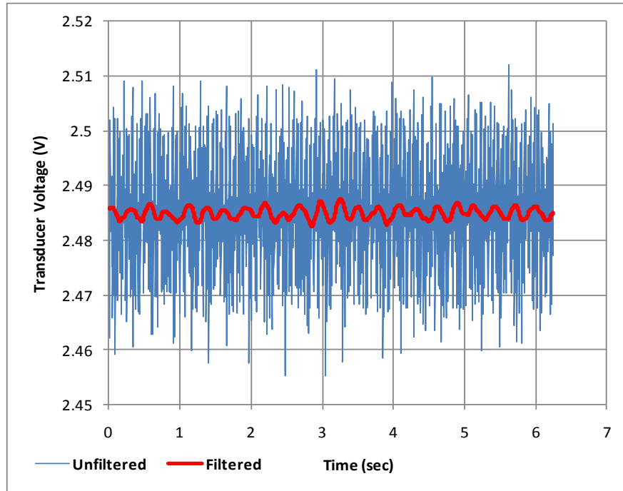
Figure 17 - Filtered and Unfiltered Pressure Transducer Signals
