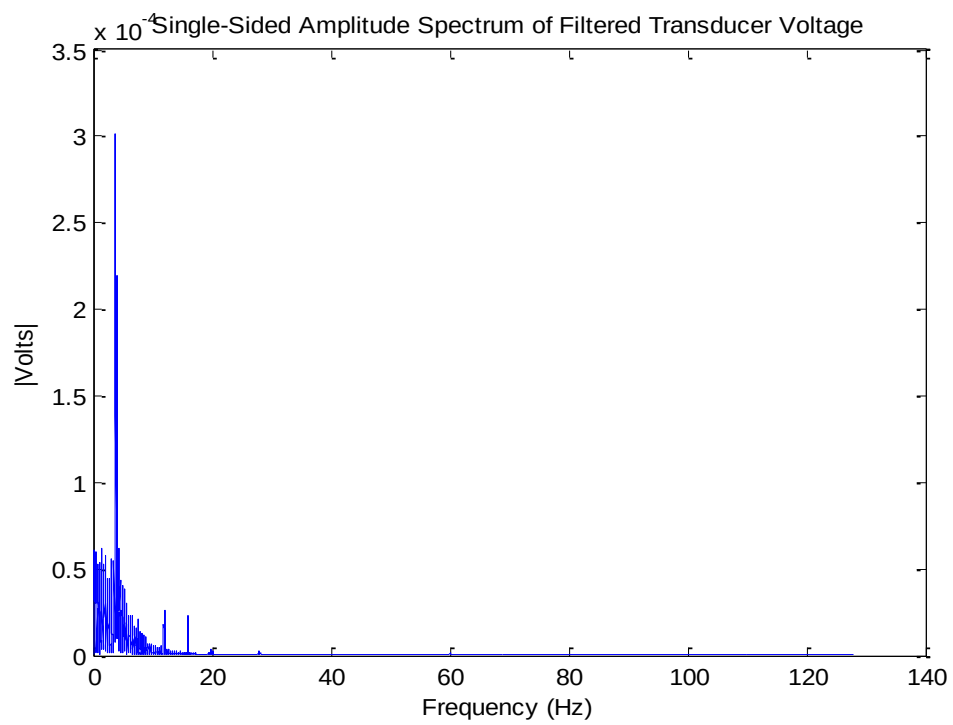
Figure 18 - Filtered Pressure Transducer Signal Frequency Spectrum
