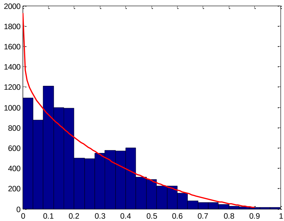
Figure A16 - Weighted Particle Distribution when System Measurements are out of Range
