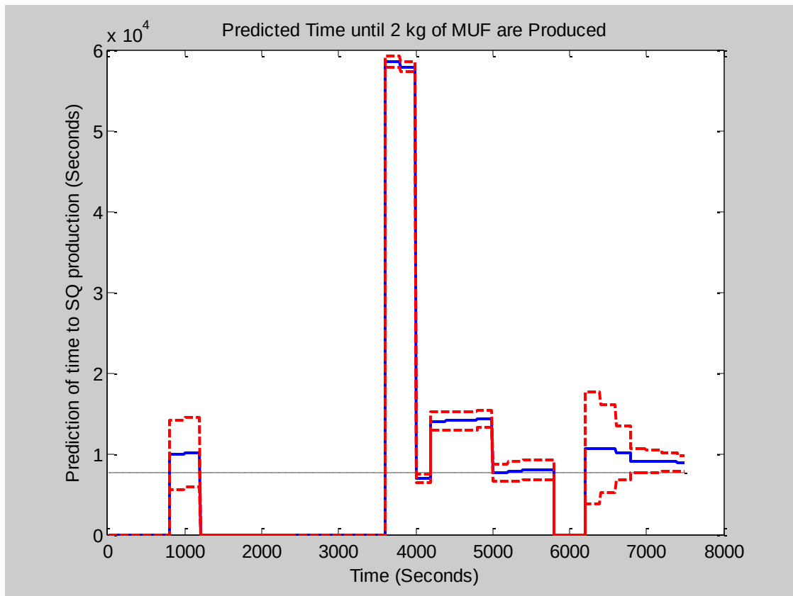
Figure 48 - Predictions of Significant Quantity Production during Intermittent Diversion
