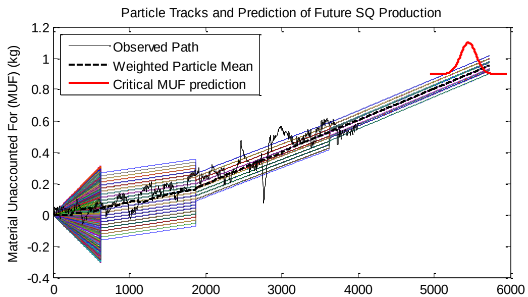
Figure A11 - Low Measurement Noise Estimate and Near-Constant Particle Weights
