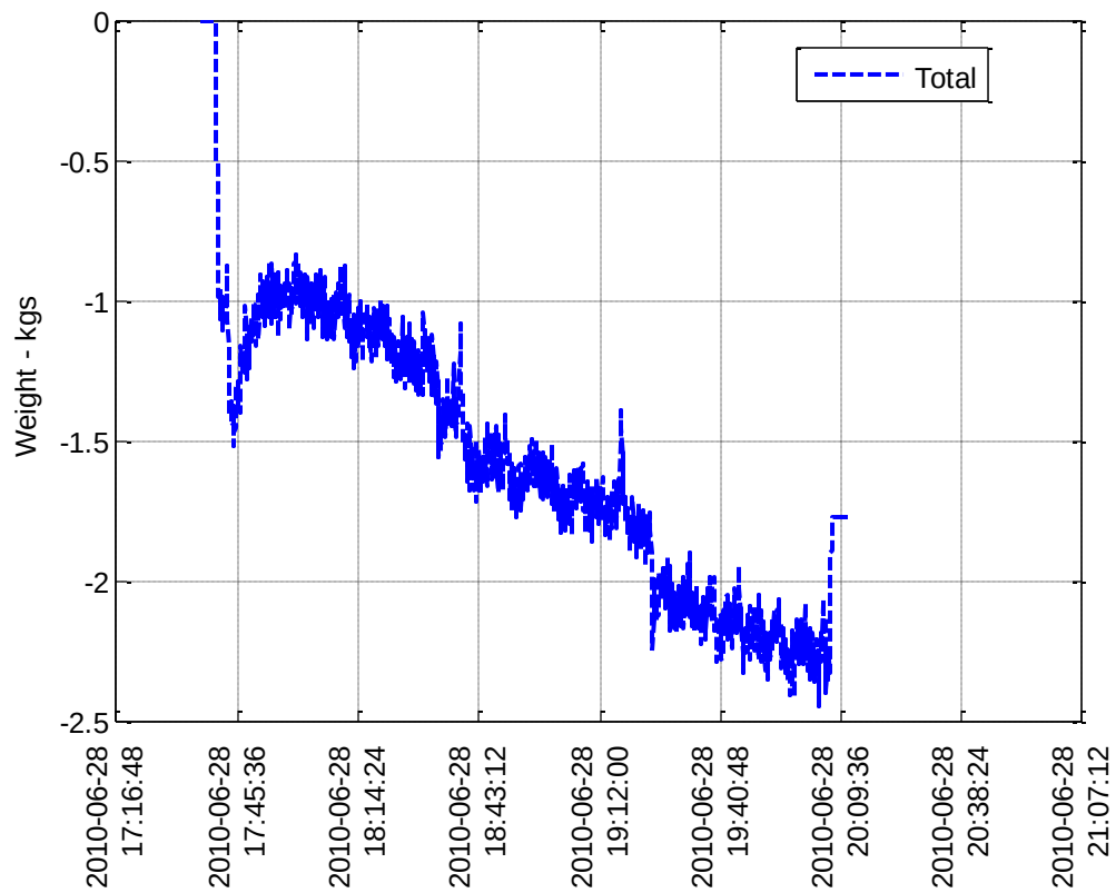
Figure A22 - Cumulative Inventory Difference for Slow Diversion
