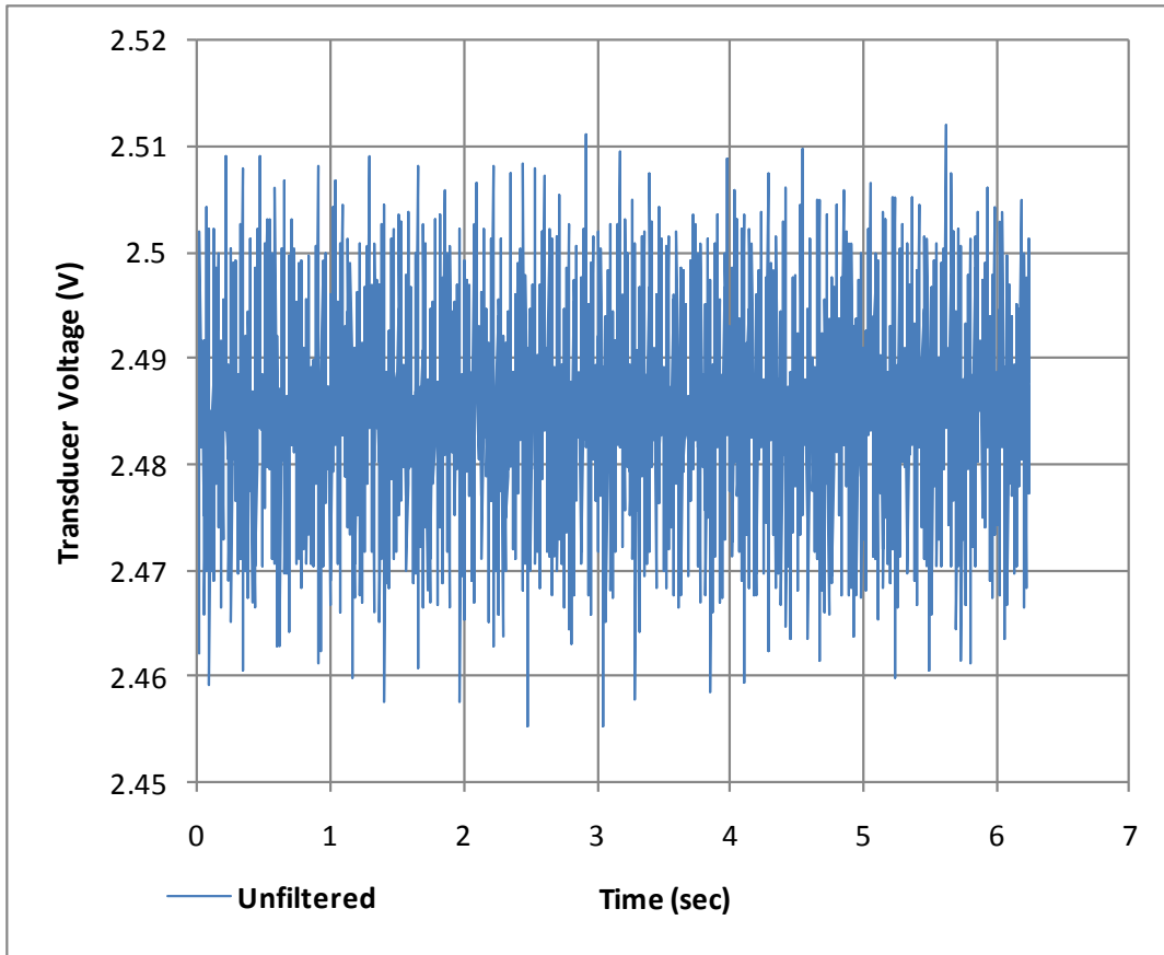
Figure 15 - Pressure Transducer Voltage with no Surge Tank Flow
