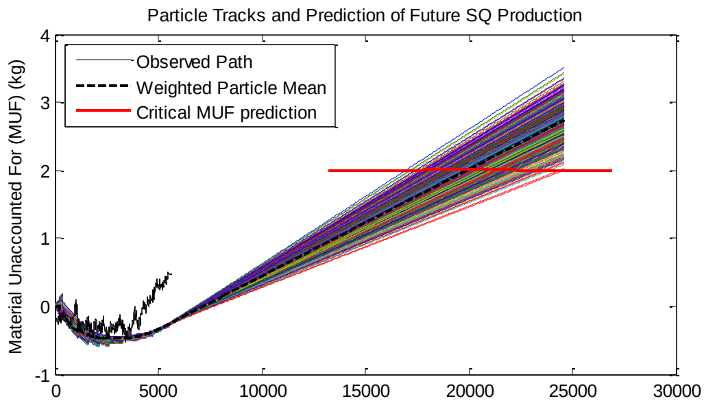
Figure A14 - Low Dynamic Noise Estimate and Slow Particle Response
