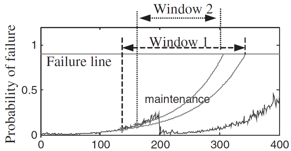
Figure 9 - GPM Failure Prediction of an Elevator Door [Yan, et al., 2004]
