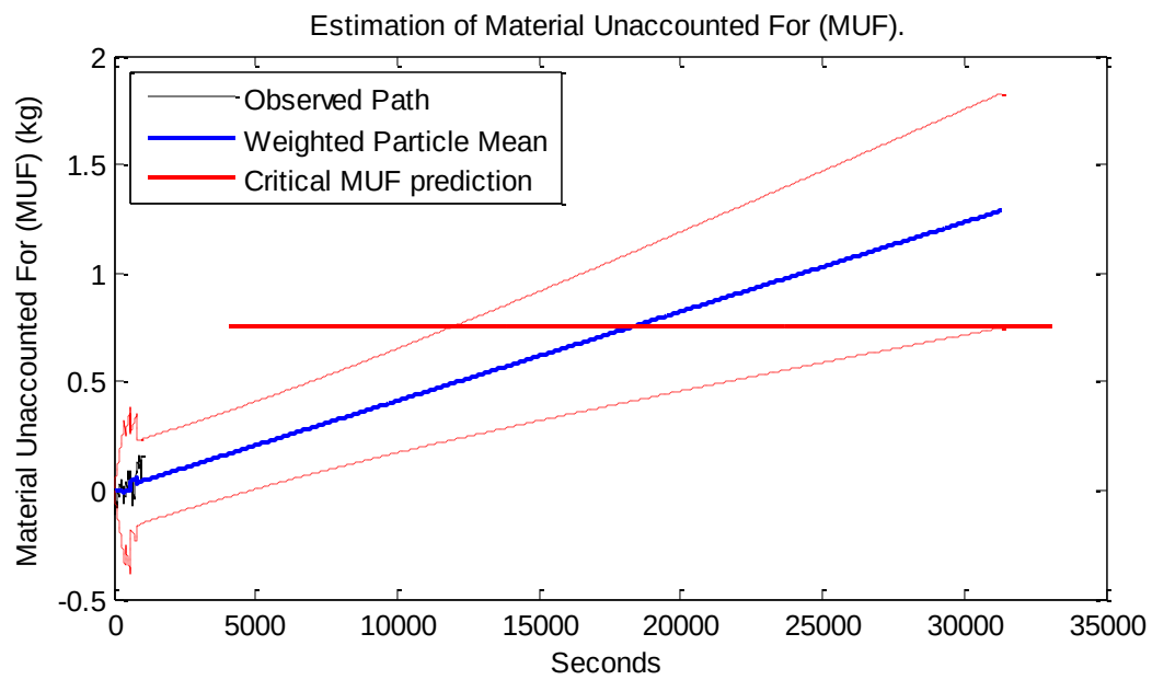
Figure 29 - Particle Filter Prediction at 16 Minutes, 40 Seconds
