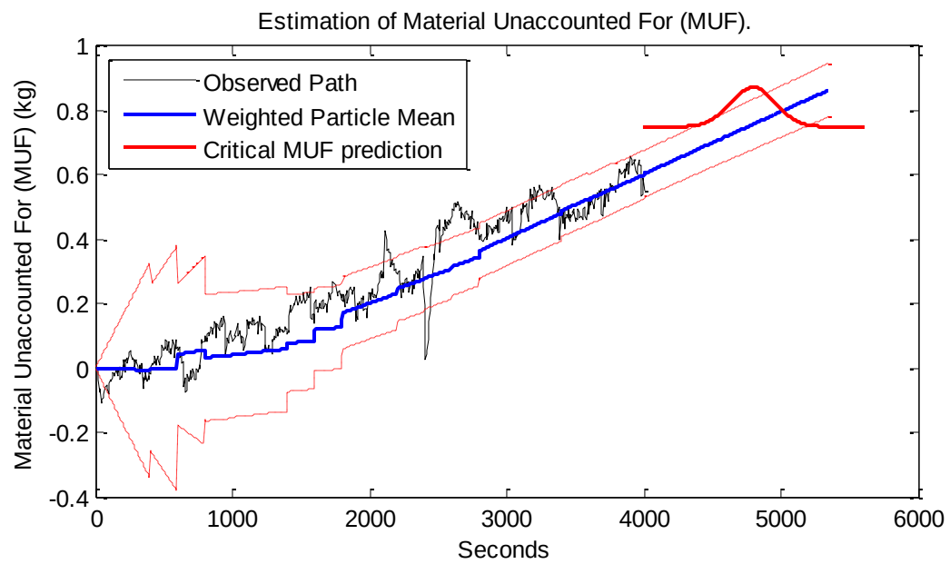
Figure 32 - Particle Filter Prediction at 66 Minutes, 40 Seconds
