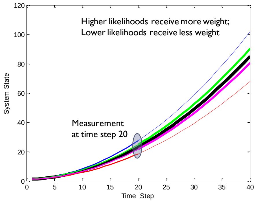
Figure 11 - Sample Estimates of the System State after Weighting
