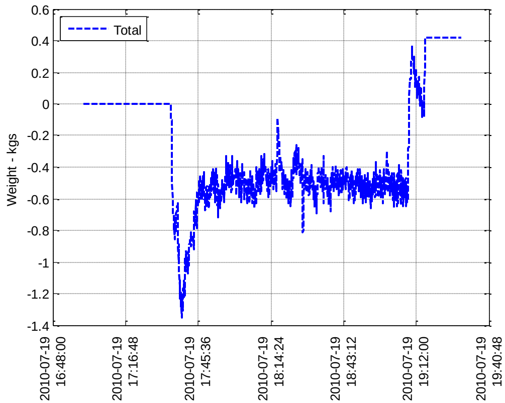
Figure A20 - Cumulative Inventory Difference for Legitimate Operation
