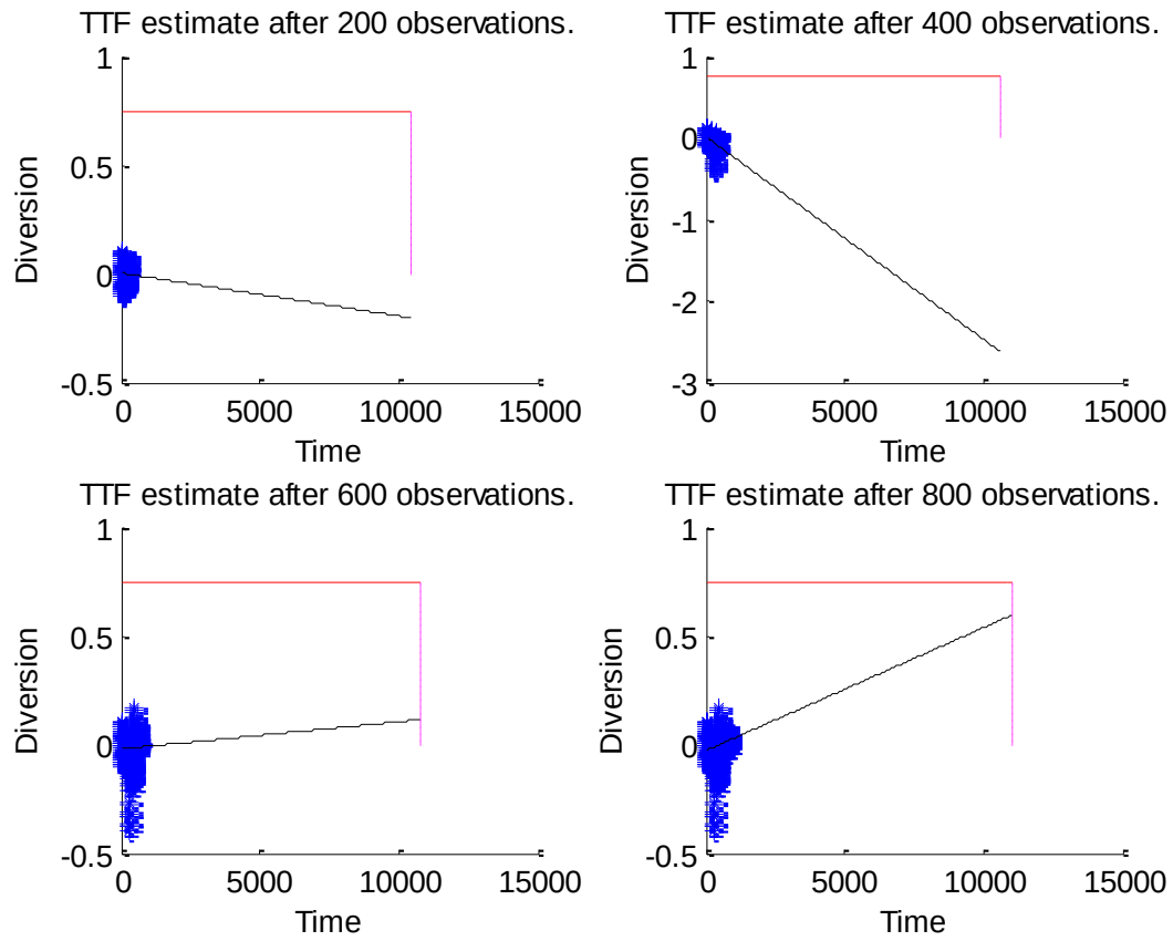
Figure 28 - General Path Model Predictions for a Legitimate Run
