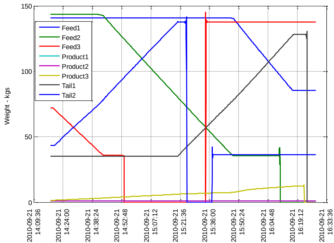
Figure A25 - Load Cell Profiles for Intermittent Diversion
