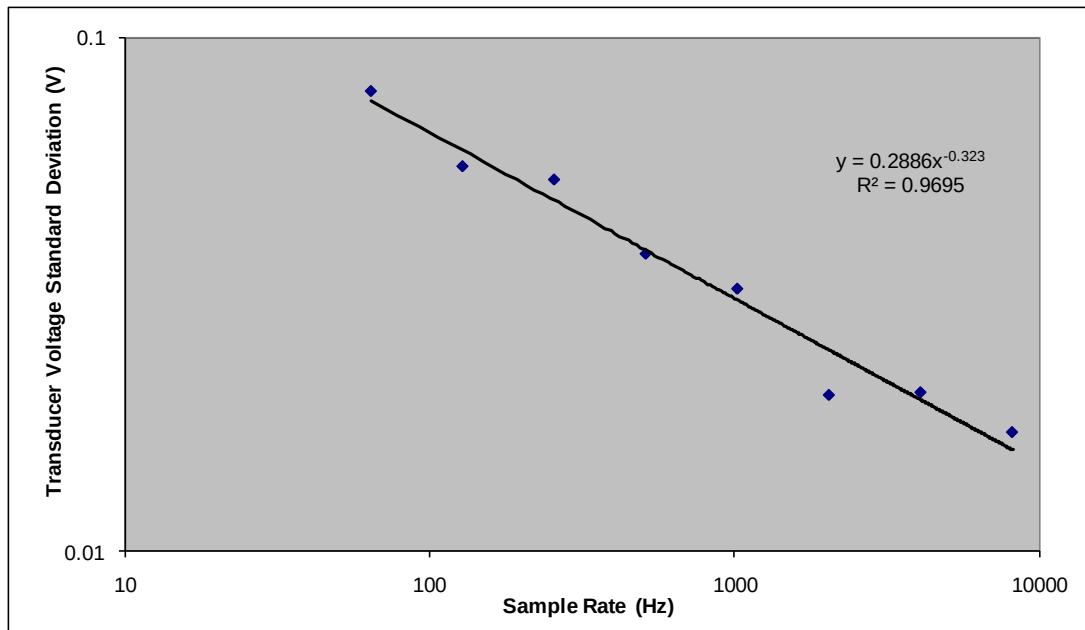
Figure 19 - Voltage Standard Deviation as a Function of Sample Rate
