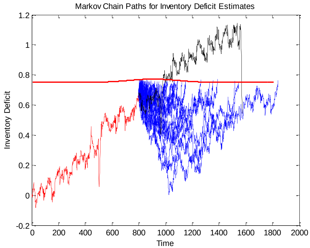
Figure 25 - Markov Chains for Fast Diversion after 800 Time Steps
