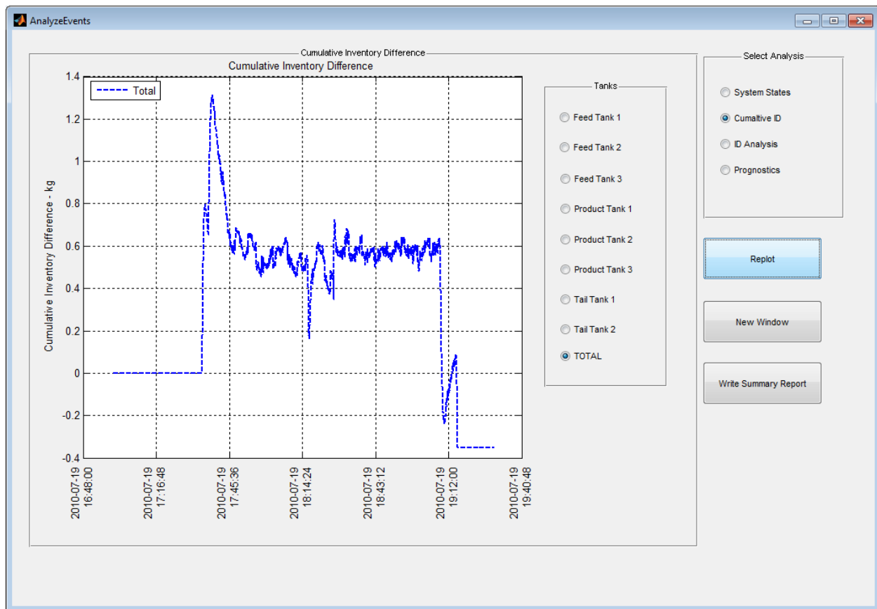
Figure 6 - PlotEvents Net Inventory Difference for a Run of the Mock F&W Facility
