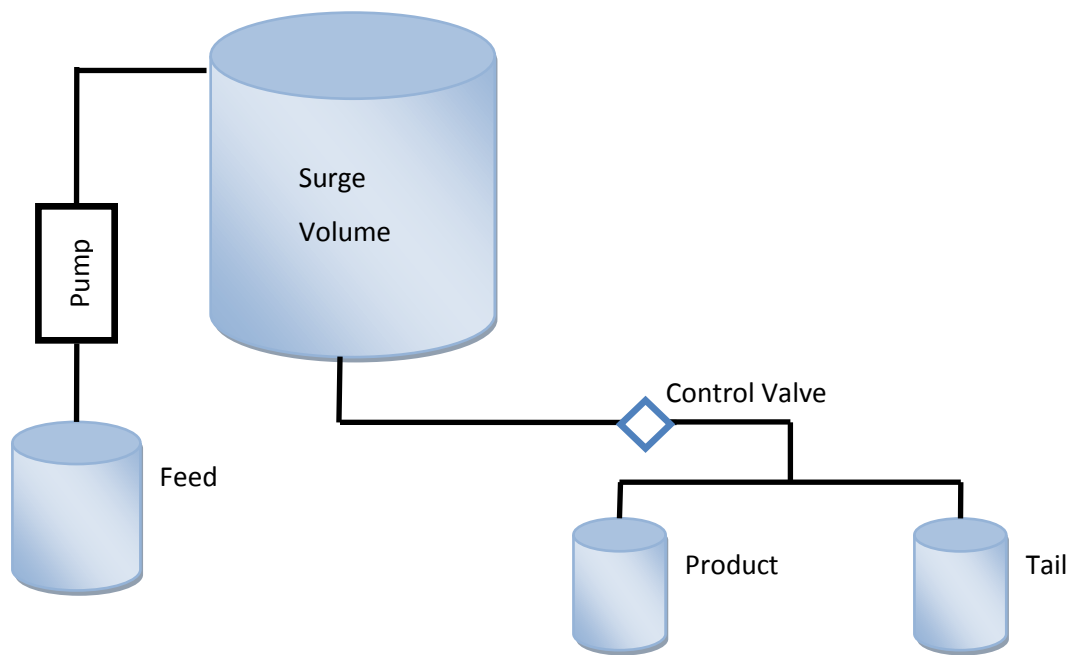
Figure 20 - Simplified schematic of the mock F&W facility
