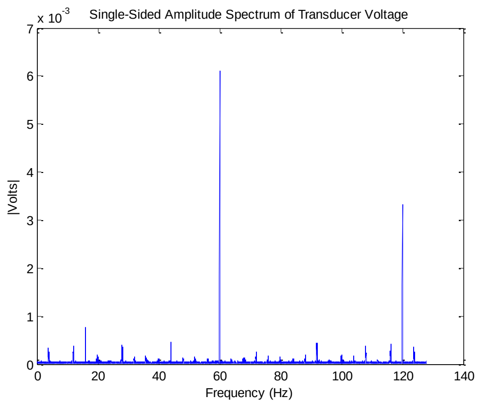
Figure 16 - Unfiltered Pressure Transducer Signal - Fast Fourier Transform
