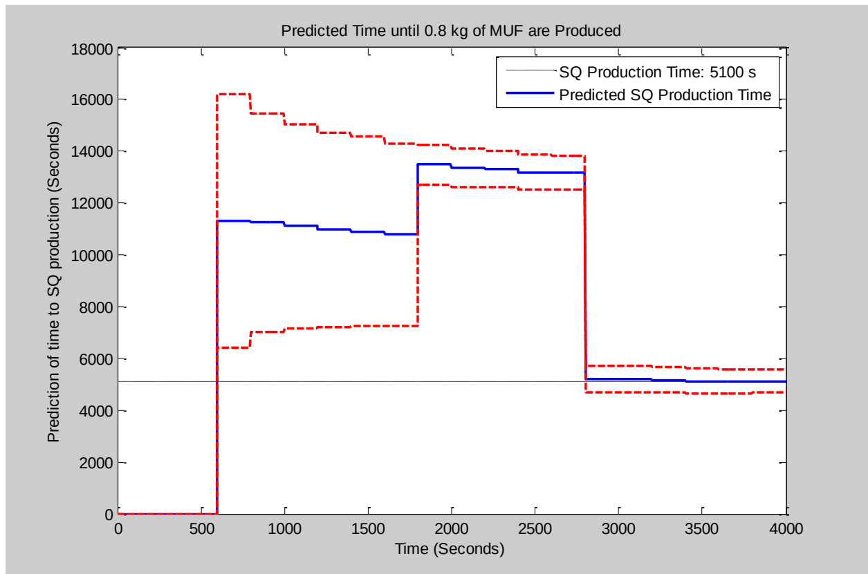
Figure 40 - Predictions of SQ Production during Slow Diversion
