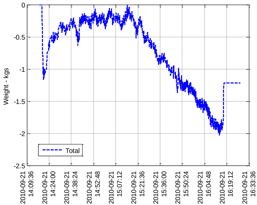
Figure A26 - Cumulative Inventory Difference for Intermittent Diversion
