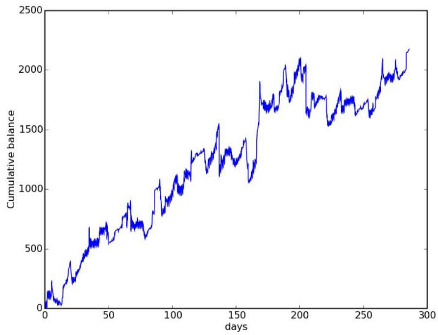
Figure 1 - MUF Calculation from Capenhurst Load Cell Evaluation [Howell, et al., 2009]
