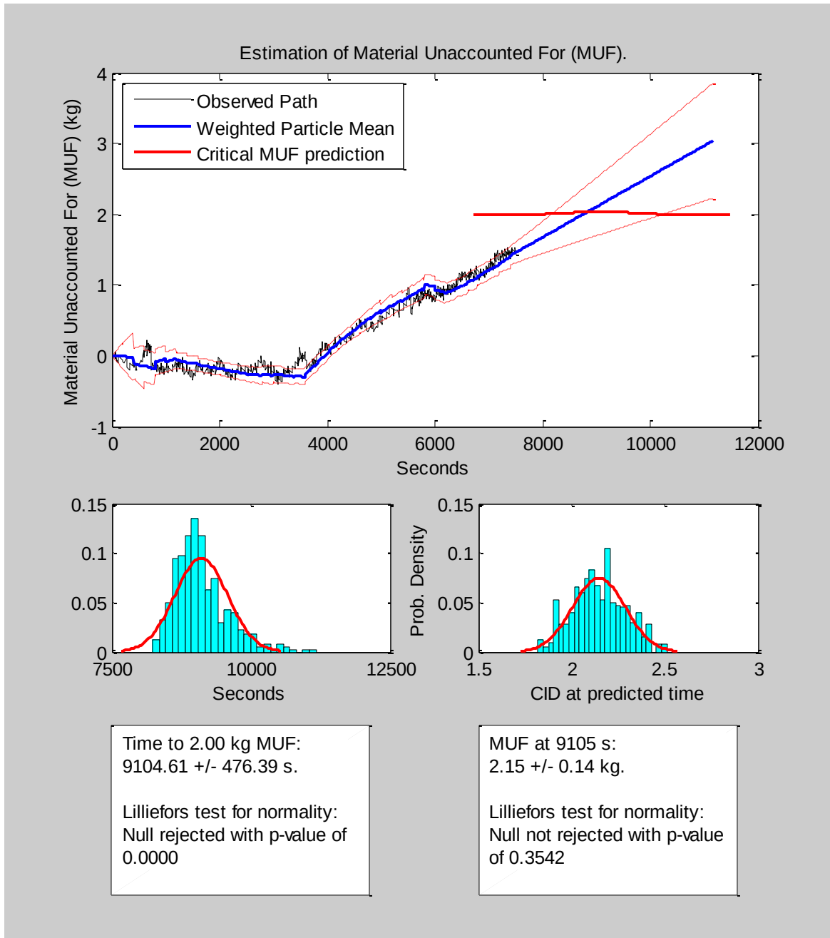
Figure 46 - Particle Statistics for the Intermittent Diversion Run at Time = 125 minutes.
