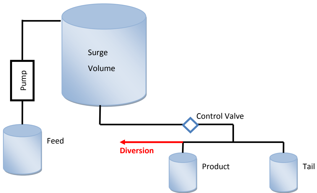
Figure 22 - Schematic of the Mock Facility with Diversion
