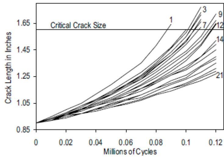
Figure 8 - Fatigue Crack Propagation in a Metal Plate [Lu, et al., 1993]
