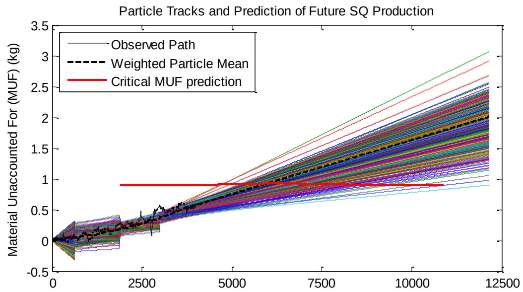
Figure A12 - High Measurement Noise Estimate and Uncontrolled Particle Distribution
