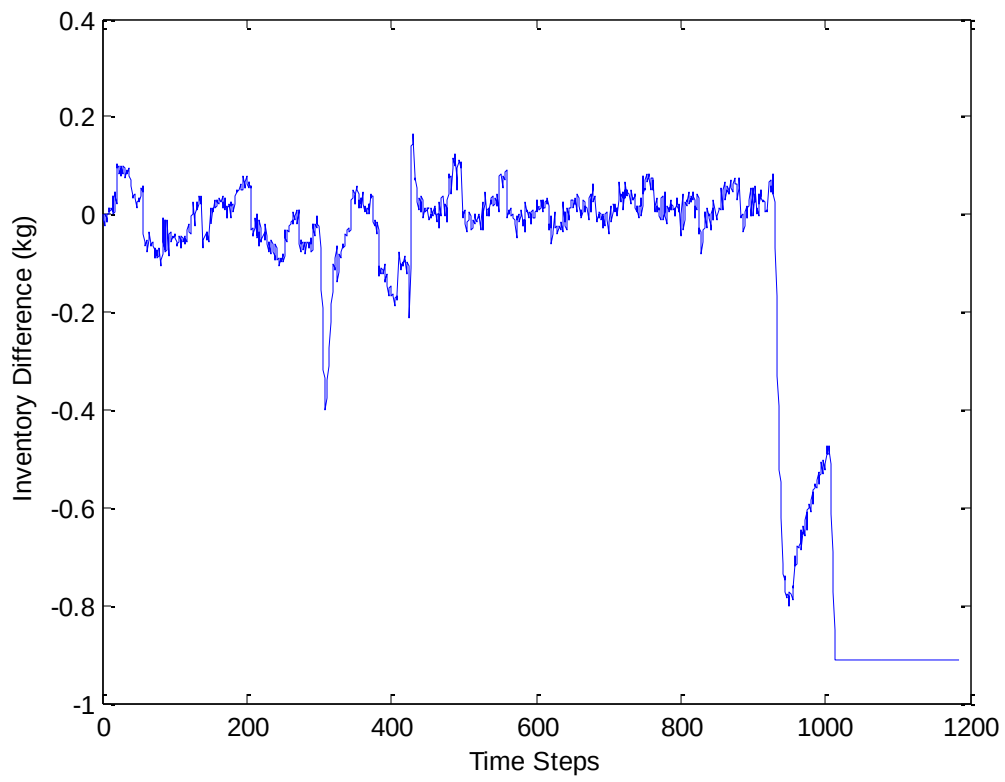
Figure 24 - Modified Inventory Difference for a Legitimate Run
