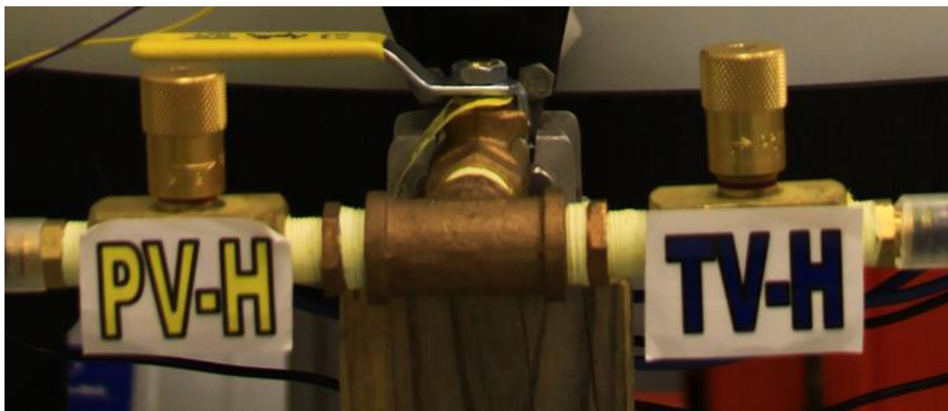
Figure A5 - Product and Tails Needle Valves, and Surge Tank Cutoff Valve
