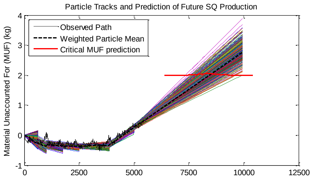
Figure A18 - Dynamic Noise Estimate Updating and Controlled Particle Variance
