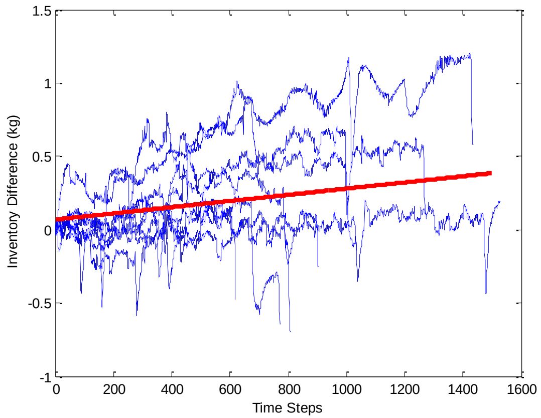
Figure 26 - General Path Model Prior Function Development
