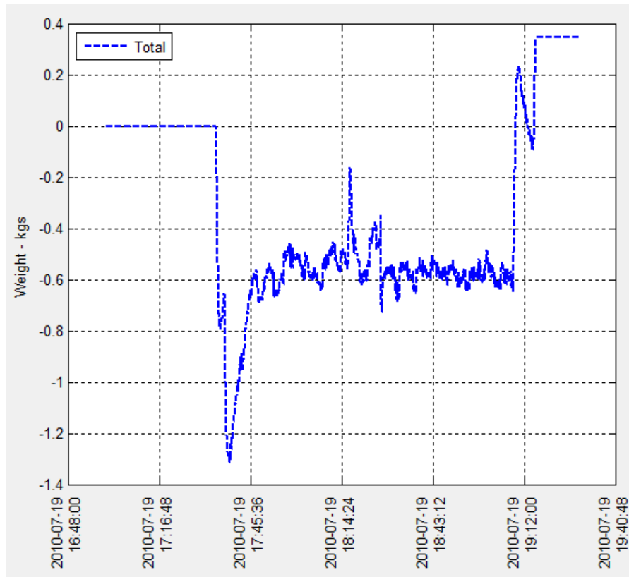
Figure 23 - Inventory Difference for a Legitimate Run
