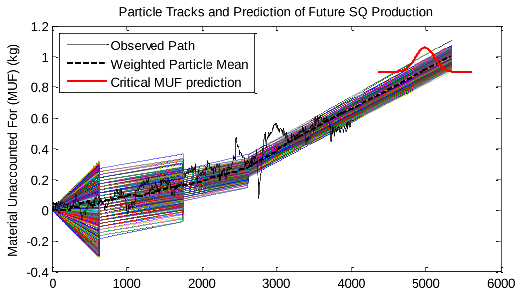
Figure A13 - Accurate Dynamic Noise and Balanced Particle Distribution
