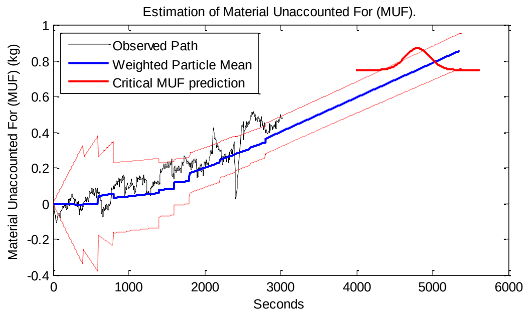
Figure 31 - Particle Filter Prediction at 50 Minutes
