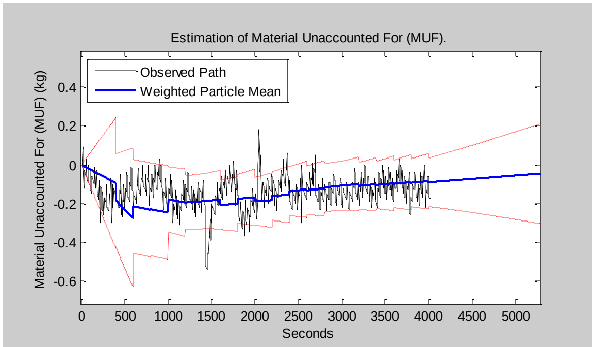
Figure 34 - Weighted Mean Particle Trace for Non-Diversion.
