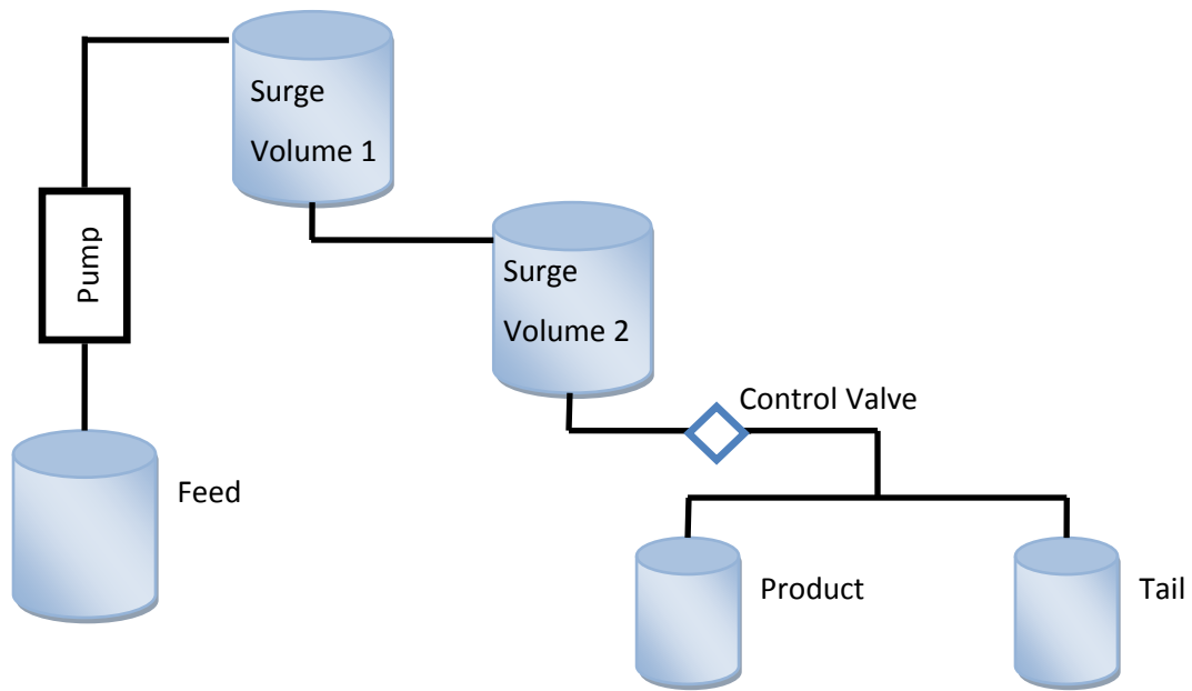
Figure 21 - Mock Facility with a Cascade of Surge Tanks
