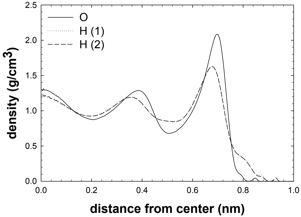
Figure 33: Radial density distribution of oxygen and hydrogen atoms when the radius of silica nanochannel is 1.0 nm (NaF). The system consists of 467 water molecules, 6 sodium ions, 2 chloride ions. 4 negative charges are distributed on the wall surface. The channel length is 6.651 nm, while the concentration of chloride ions ( 0.132/\text{nm}^3 ) and density of charges on the wall ( 0.0957/\text{nm}^2 ) are kept constant.
