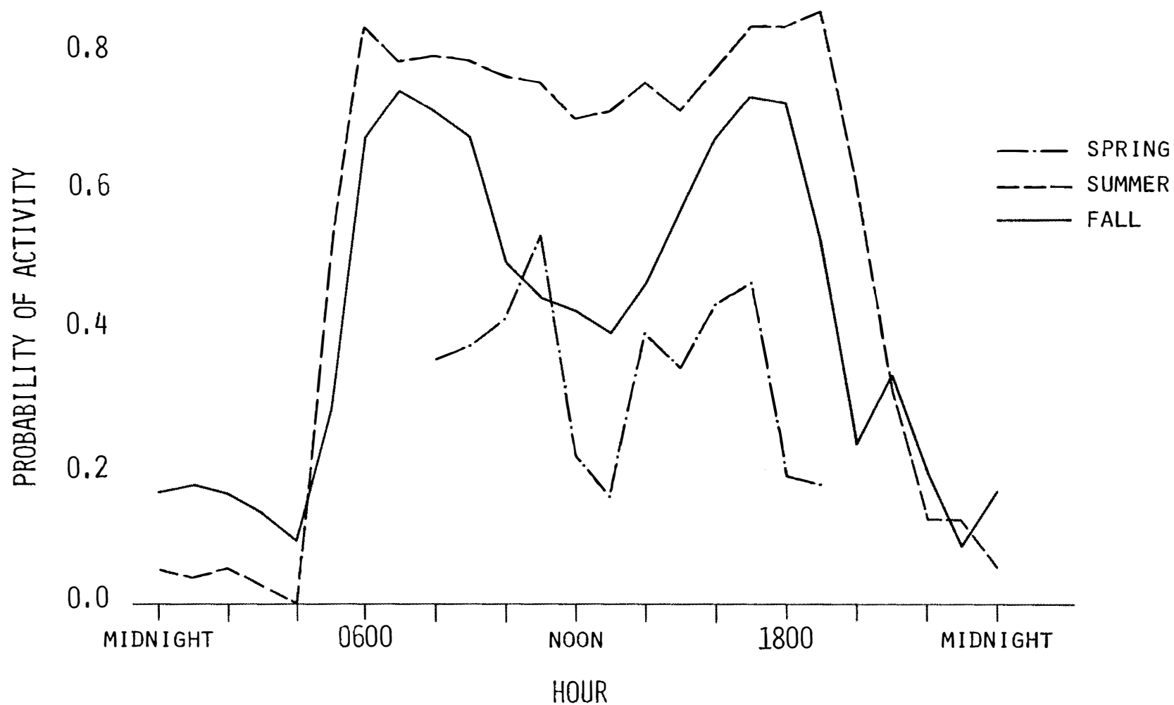
Fig. 4. Hourly probability of activity for black bears in the GSMNP, 1980-82.
