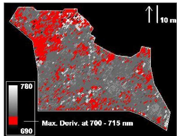
Figure 6.2-29: REPI; 07 May 2015.
