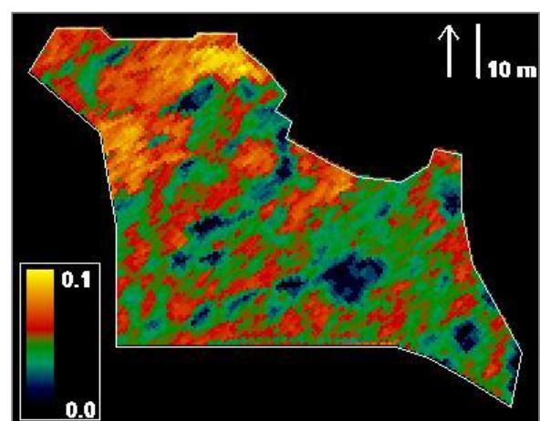
Figure 6.2-14: SGI; 07 May 2015.
