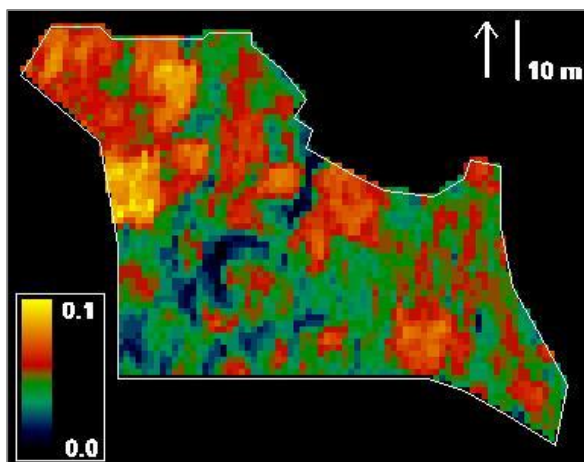
Figure 6.2-13: SGI; 17 April 2015.
