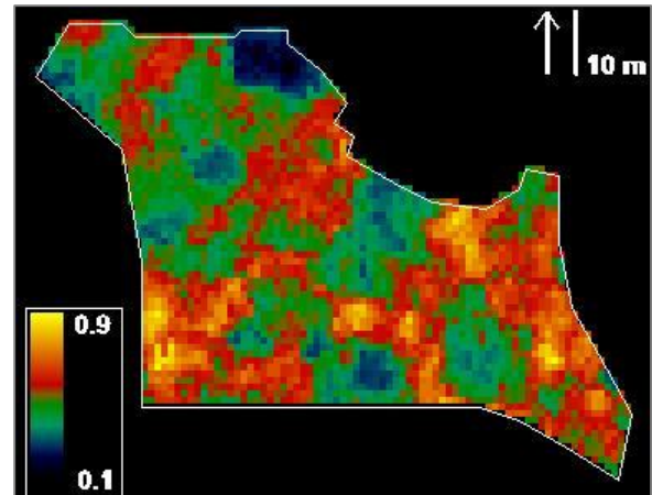
Figure 6.2-25: MRENDVI; 17 April 2015.
