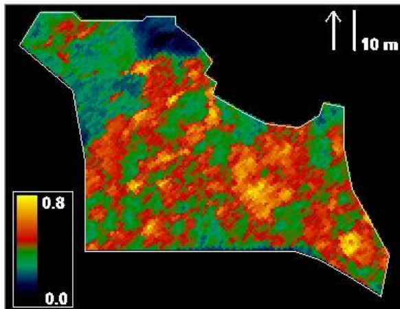
Figure 6.2-20: RENDVI; 07 May 2015.
