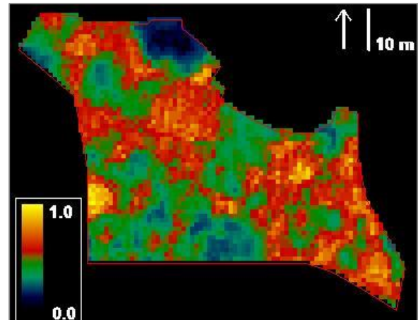
Figure 6.2-10: NDVI; 17 April 2015.
