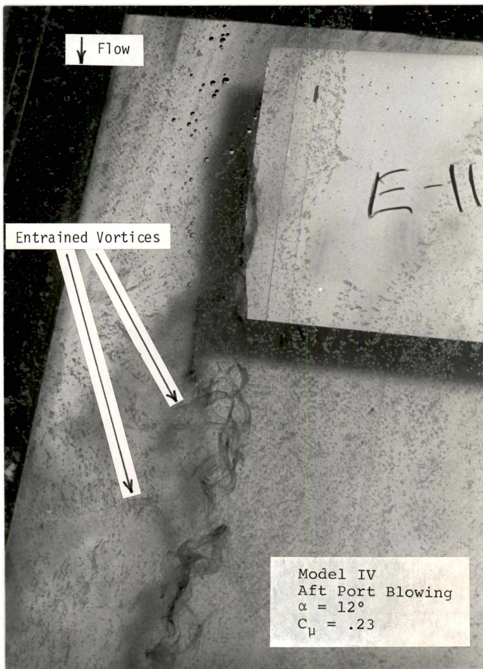
Figure 25. Entrained Vortices
