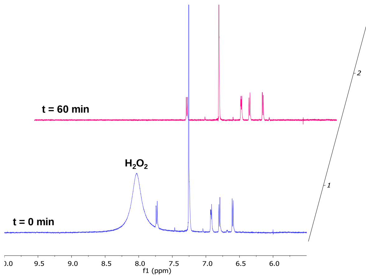
Figure 71 NMR spectra t = 0 minutes (1, blue) and t = 60 minutes (2, pink) illustrating the consumption of \text{H}_2\text{O}_2 .
