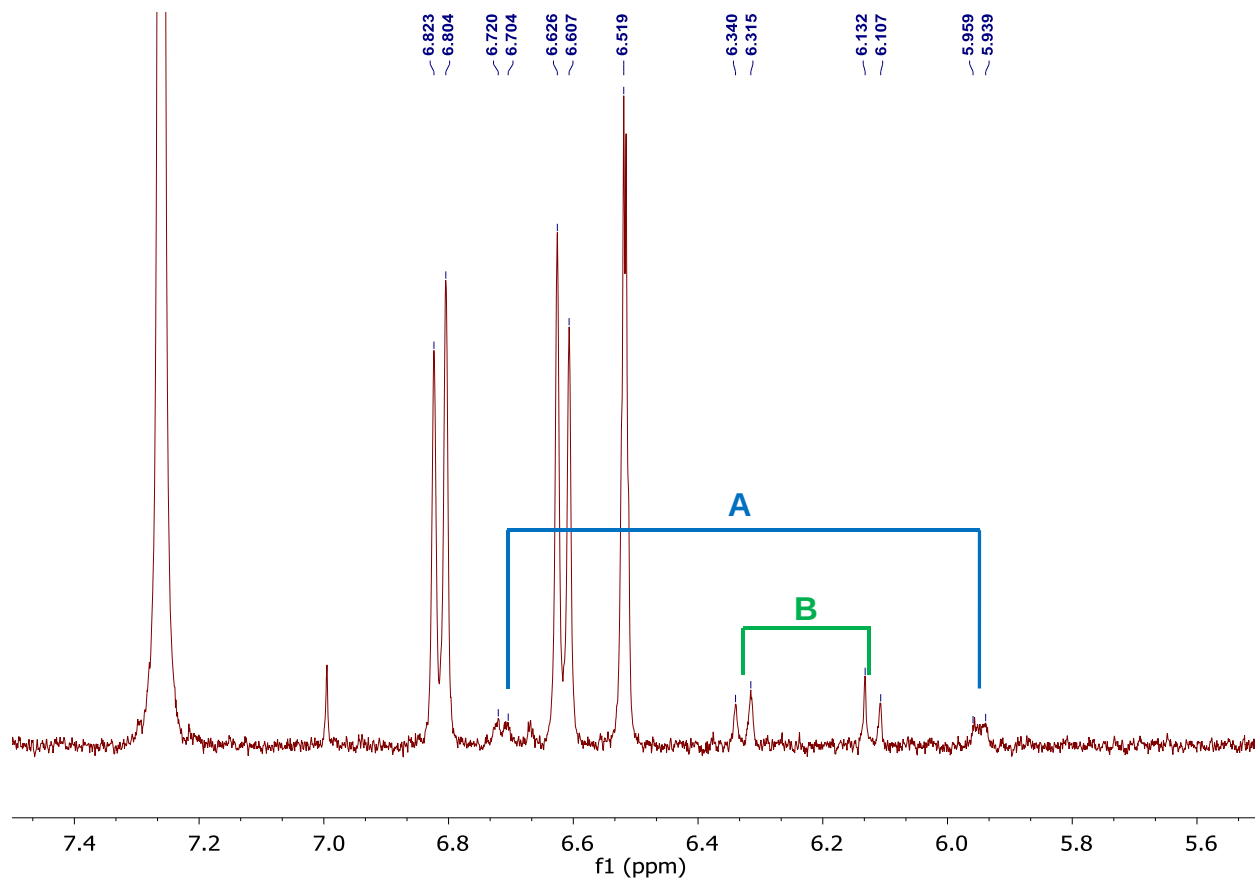
Figure 120 Typical NMR spectrum taken at 60 minutes after the addition of hydrogen peroxide illustrating the two sets of doublets corresponding to the two major side products.
