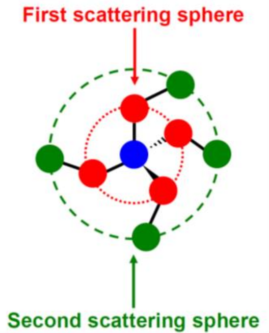
Figure 49 Illustration of the scattering spheres.
