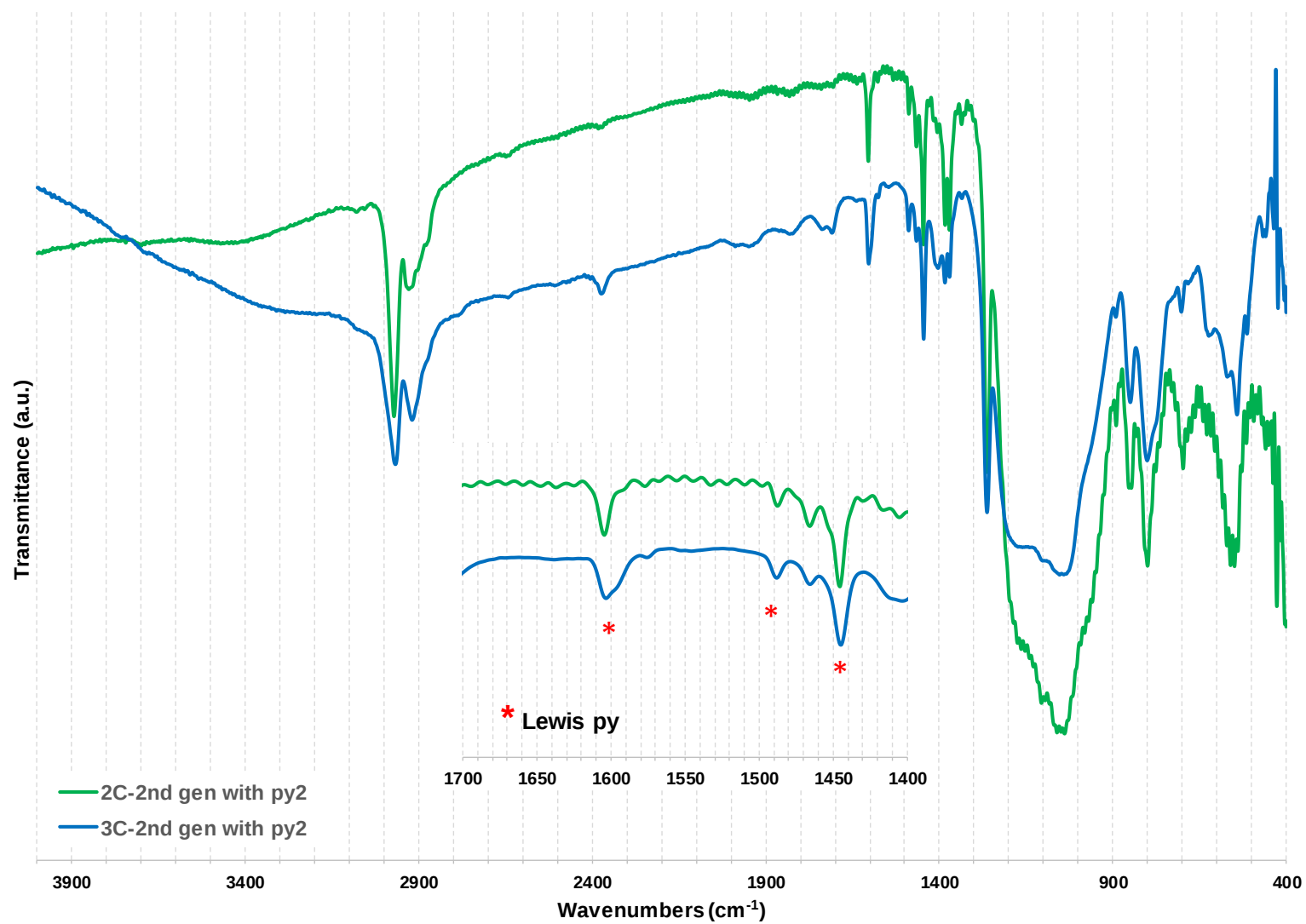
Figure 108 FTIR spectra of 2C-2 nd gen with py 2 (green) and 3C-2 nd gen with py 2 after the second cross-linking reaction.
