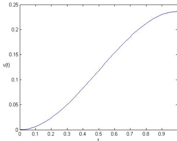
Figure 3: Solution to u'''(x) + Lu'(x) + K \cos(u(x)) = 0 with u(0) = u'(0) = u'(1) = 0
