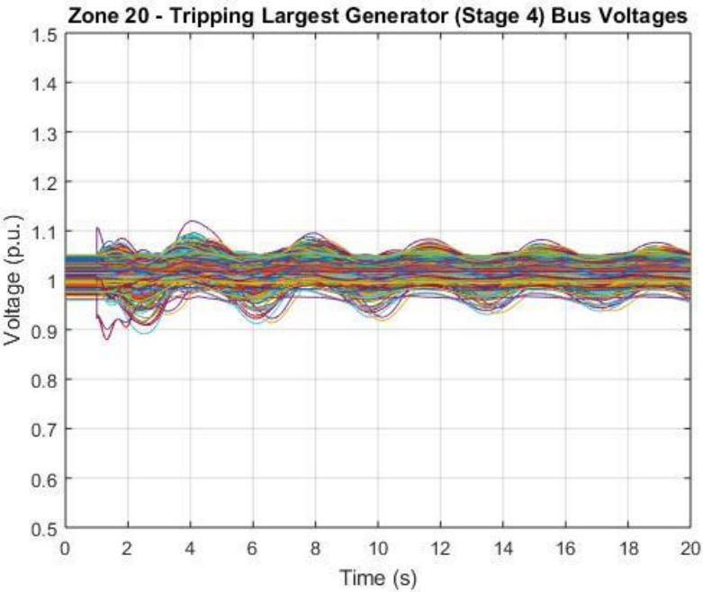
Figure 4.19. System voltage while tripping 4 levels from largest generator in Zone 20
