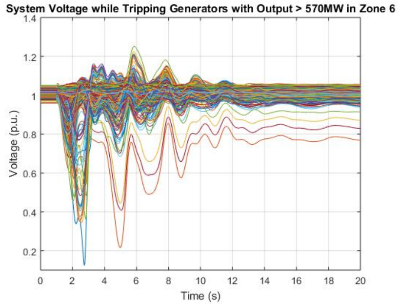
Figure 4.6. System voltage while tripping generators with output greater than 570 MW in Zone 6
