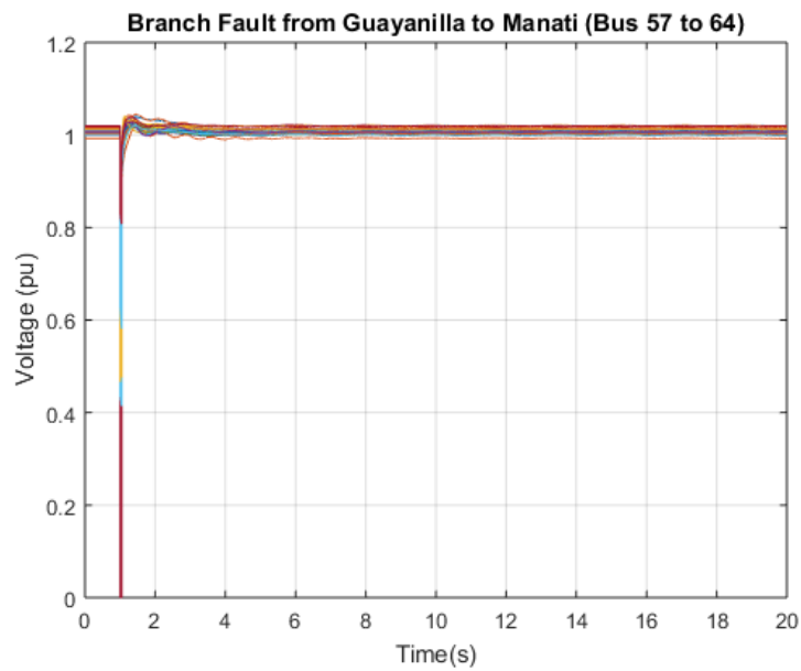
Figure 3.17. System voltage after a three-phase short-circuit fault on the Guayanilla-Manatí 230kV transmission line
