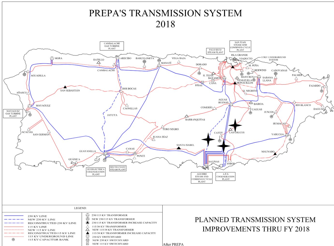
Figure 3.22. Transmission map indicating Cluster 2 with annotations added to map from [38]
