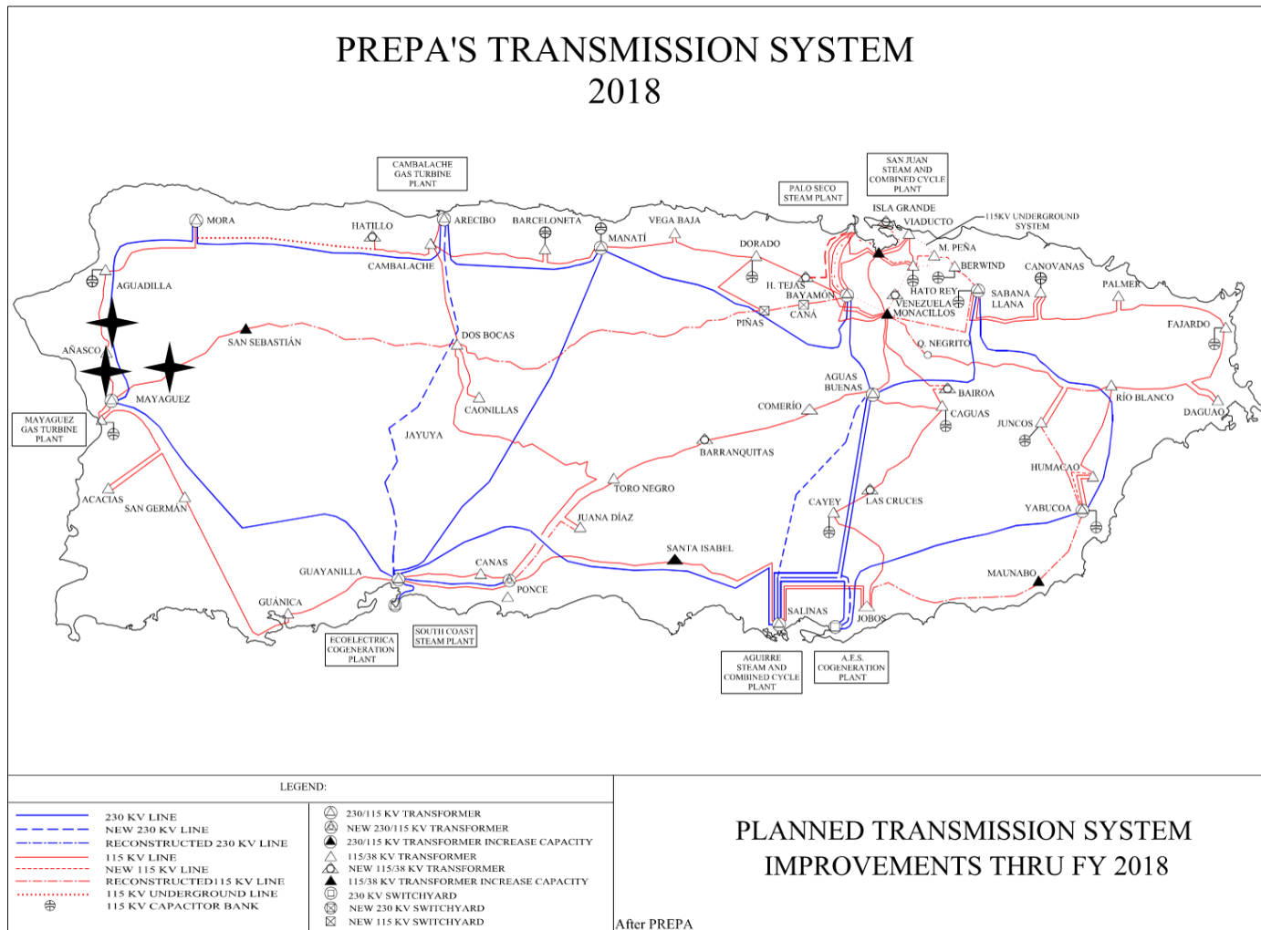
Figure 3.26. Transmission map indicating Cluster 4 with annotations added to map from [38]
