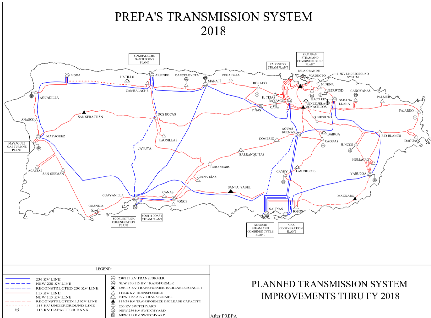
Figure 3.1. PREPA's 2018 transmission system [38]
