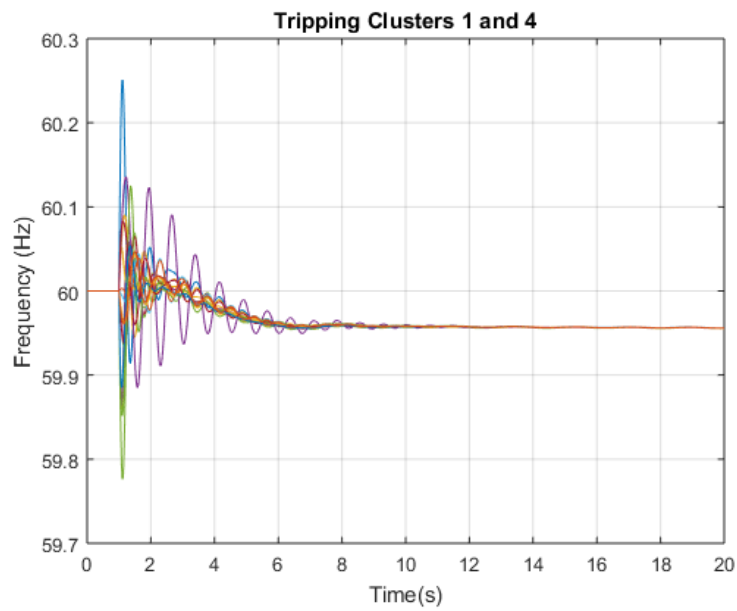
Figure 3.28. Frequency response after tripping Cluster 1 and Cluster 4
