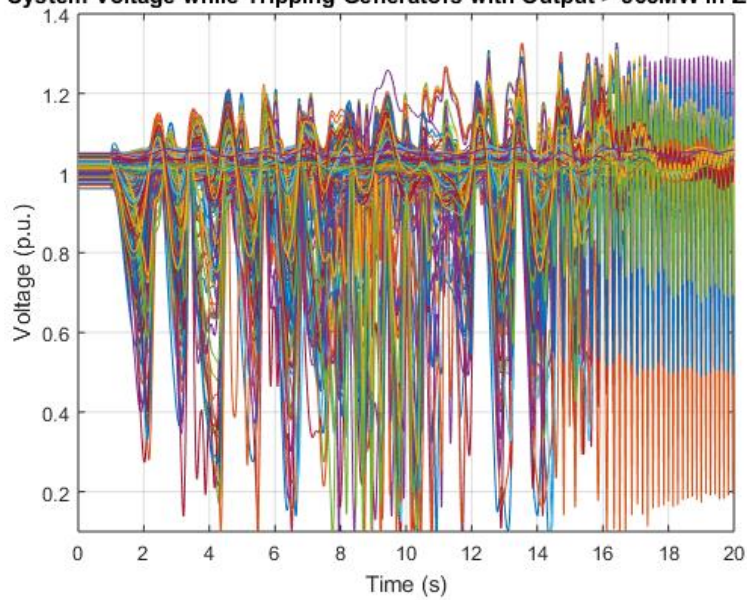
Figure 4.8. System voltage while tripping generators with output greater than 565 MW in Zone 6
