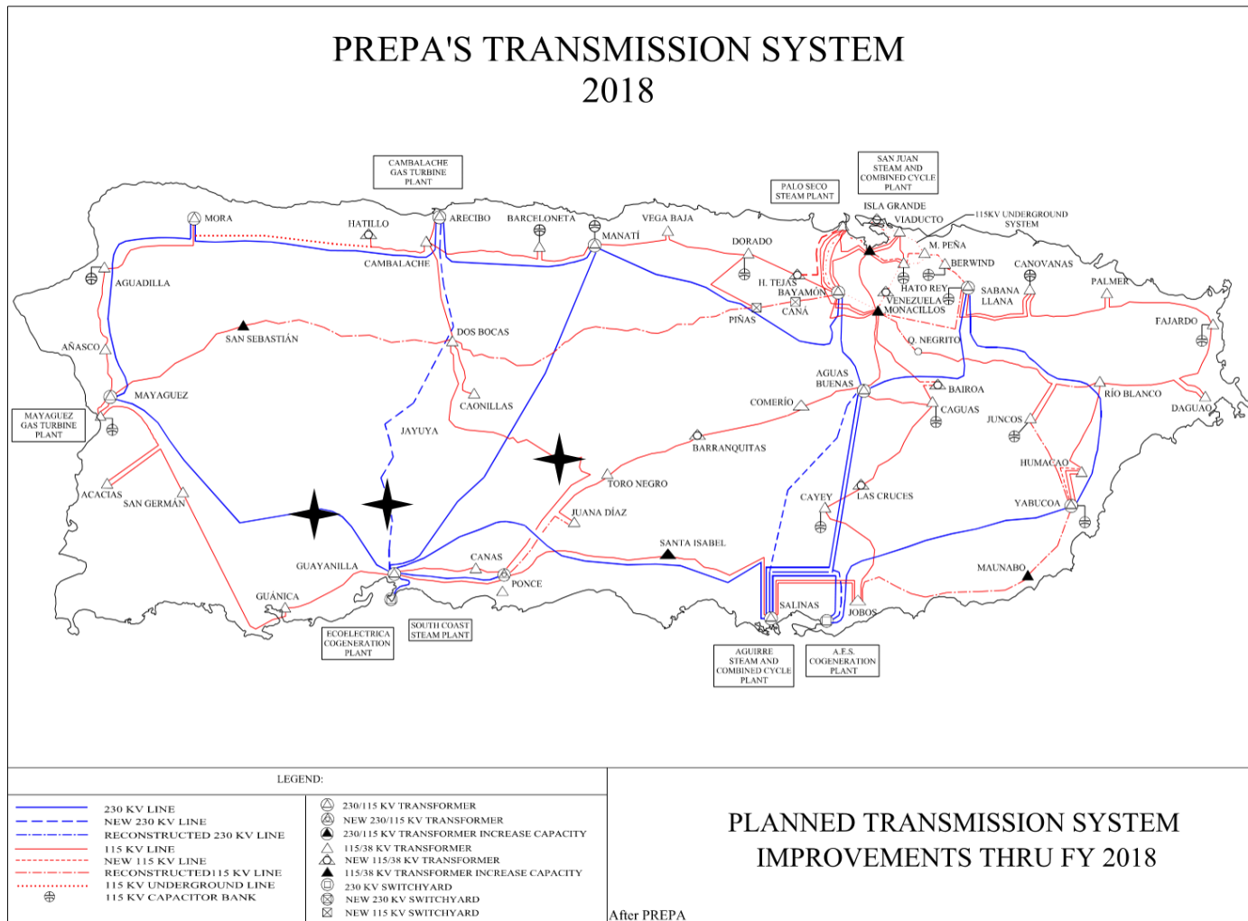
Figure 3.20. Transmission map indicating Cluster 1 with annotations added to map from [38]
