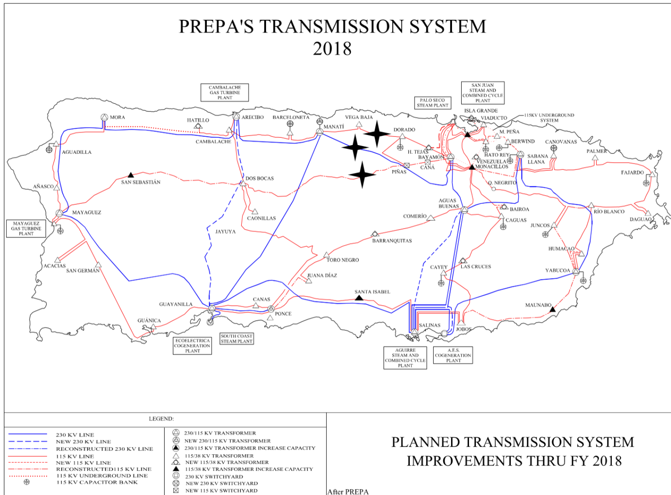
Figure 3.24. Transmission map indicating Cluster 3 with annotations added to map from [38]
