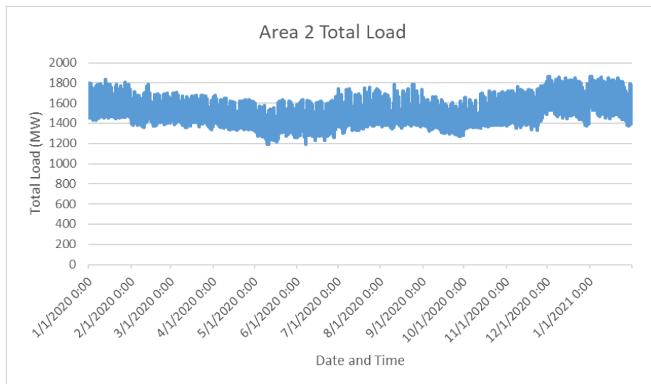
Figure 2.7. Total load curve for Area 2 of the 23-bus system
