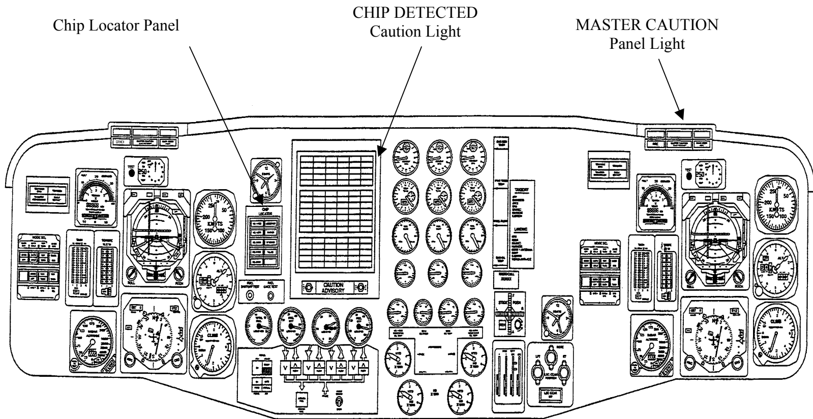
Figure 10 Instrument Panel
