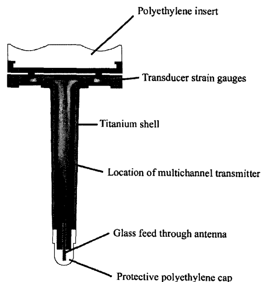
Figure 2. D'Lima and Colwell's 2005 telemetric knee design
