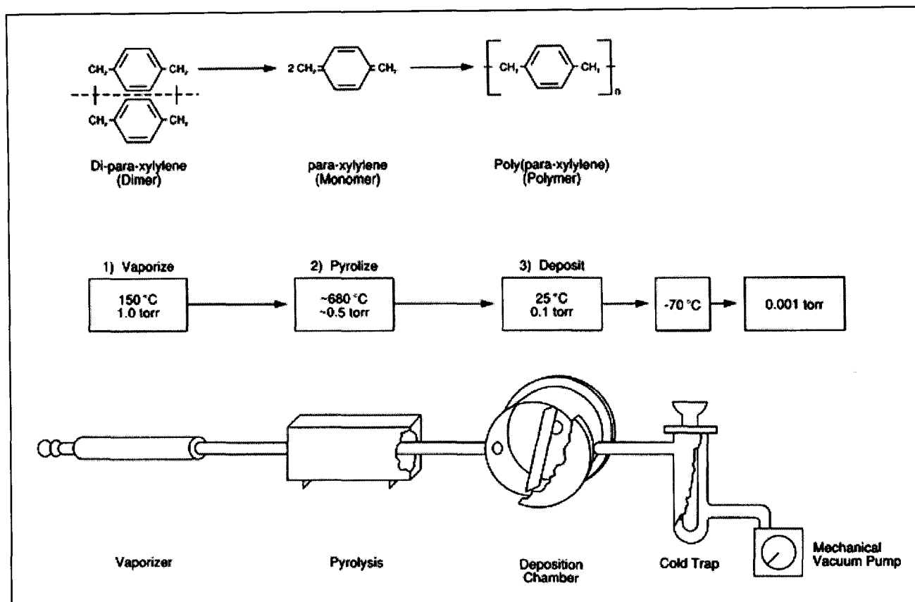
Figure 7. Parylene Deposition Schematic [31]
