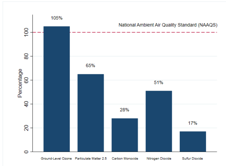
Figure A1.1: Nonattainment of O 3 Standards
