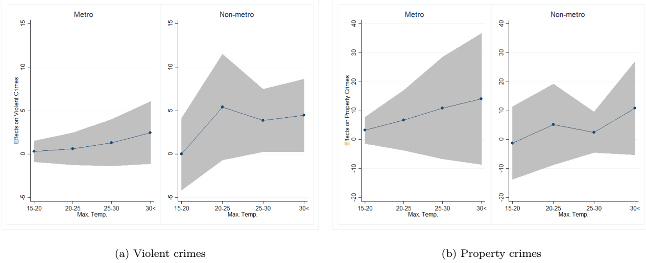
Figure 3.3: Marginal Effects of Temperature (Simple FE Model)
