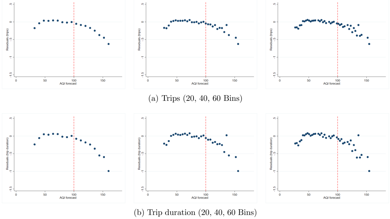
Figure 1.2: Residual Plots
