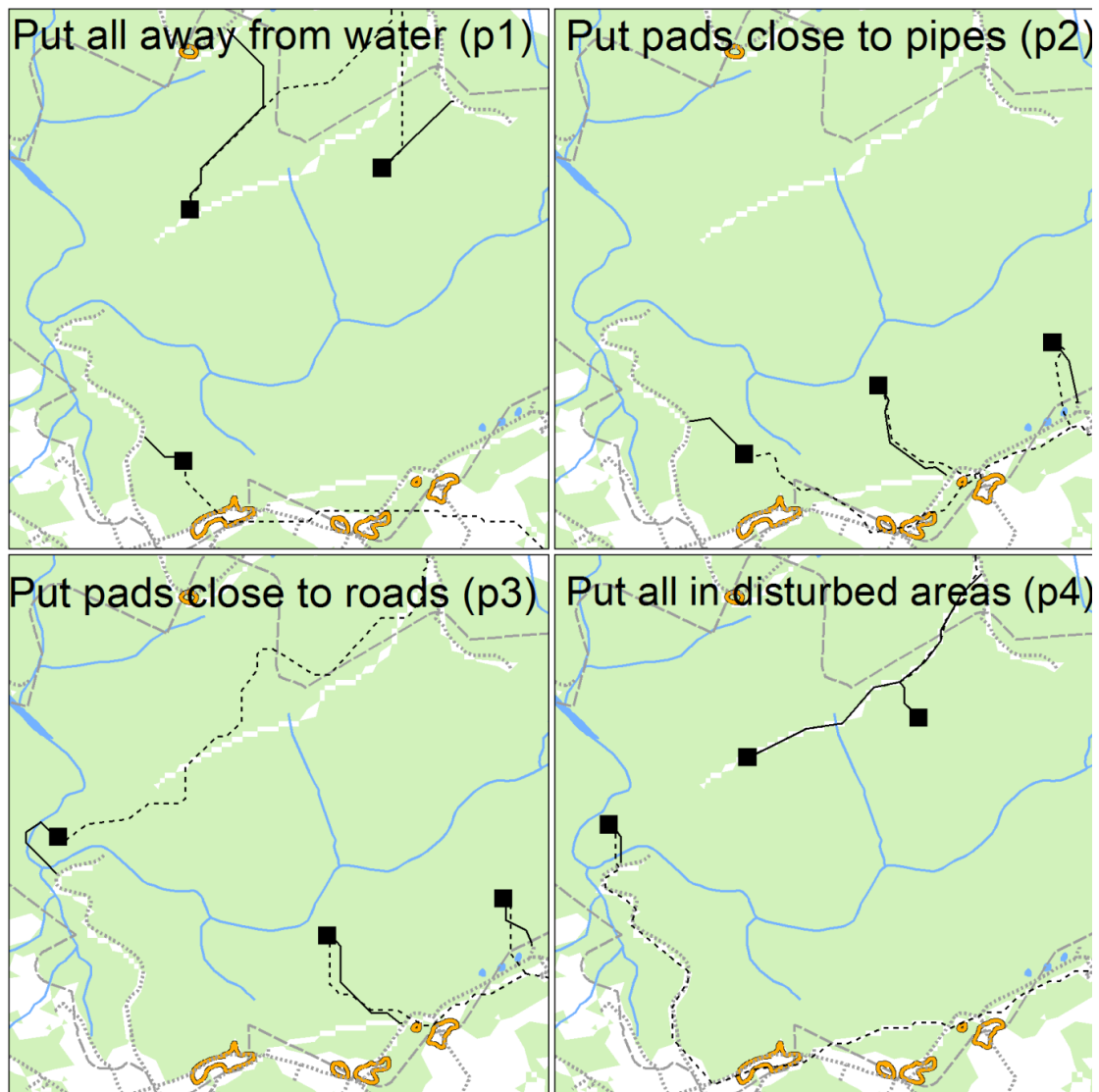
Fig. 2.3. Four layouts of well pads (■), roads (-), and pipelines (--) at one of our twenty sites (medium gray --). Other layouts presented in the Appendix. Existing roads are medium gray dots (...); proposed infrastructure is black. Each layout is the result of following a different simple siting practice (codes here). Each layout, if developed, would result in different impacts on forests (green or light gray), aquatic habitats (blue or medium gray), erosion, and cultural features (orange or dark gray with black outline) (Table S 2.2 for values).
