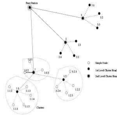
Figure 2.4: Hierarchical Clustering
