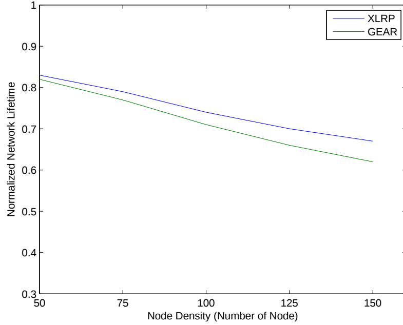
Figure 5.4: Lifetime of the sensor network with increasing network density
