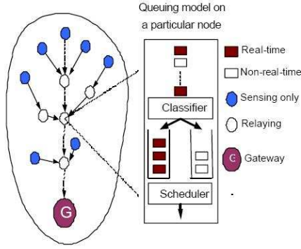
Figure 2.7: Queuing model for Energy Aware QoS Routing
