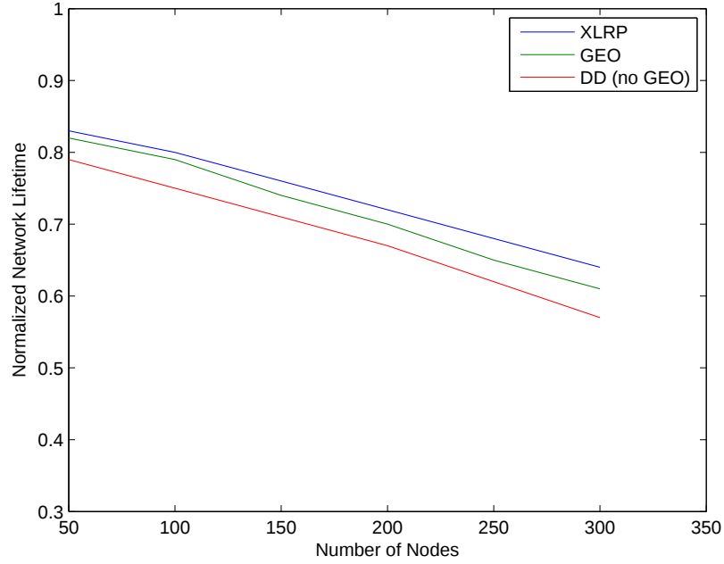
Figure 5.3: Lifetime of the sensor network with increasing network size
