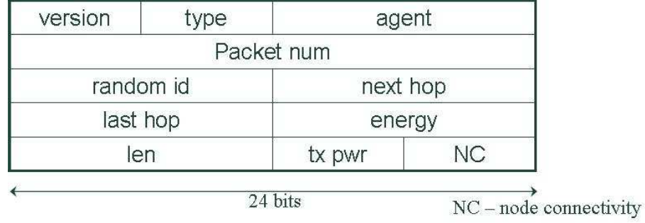
Figure 4.4: XLRP Header Format
