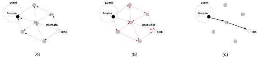
Figure 2.2: Directed Diffusion (a) Interest Propagation Phase (b) Gradient Setup Phase (c) Data Dissemination Phase.
