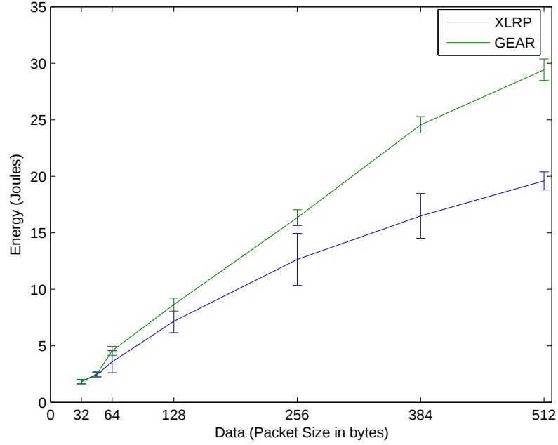
Figure 5.1: Energy consumption with varying data size
