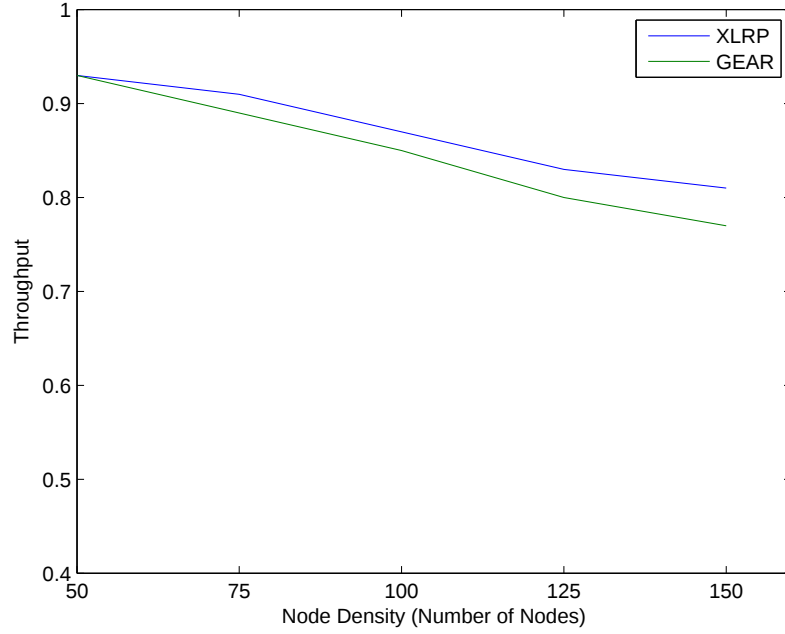
Figure 5.5: Throughput of the network with increasing node density
