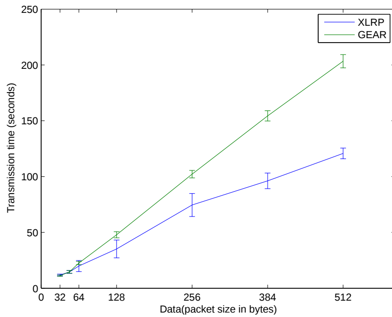
Figure 5.2: Latency Measure with respect to data size
