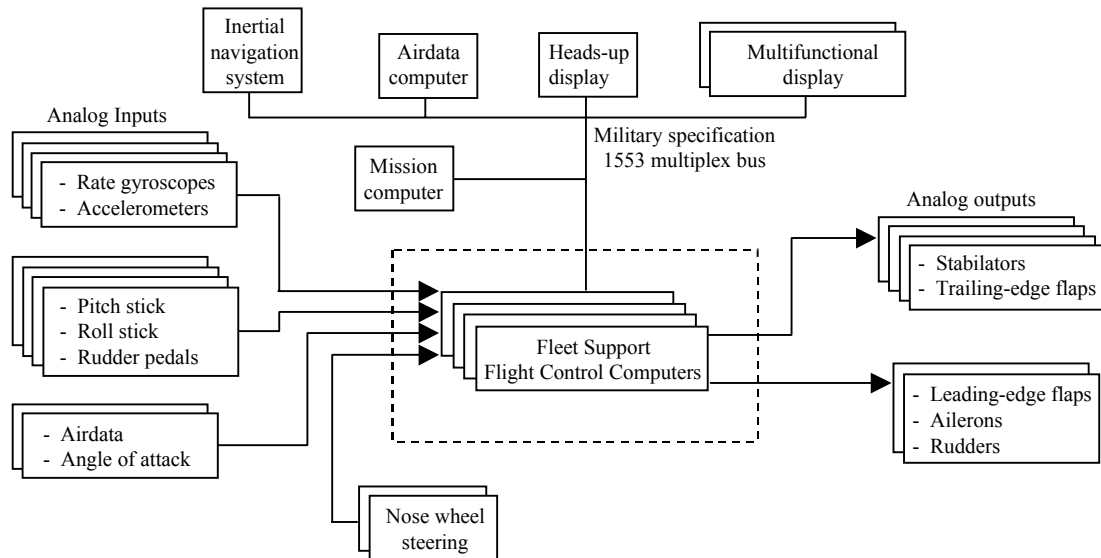
Figure 5: F/A-18C FCS Components
