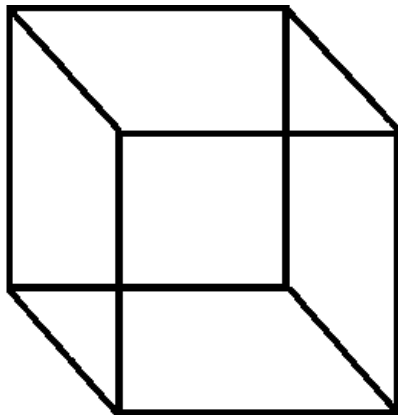
Figure 91. Necker Cube
