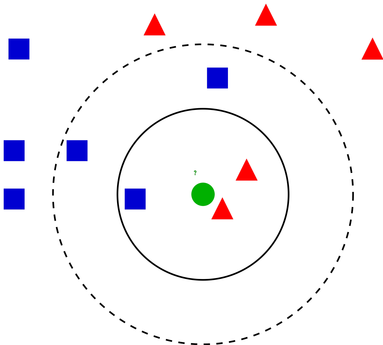
Figure 1.3: K-NN
