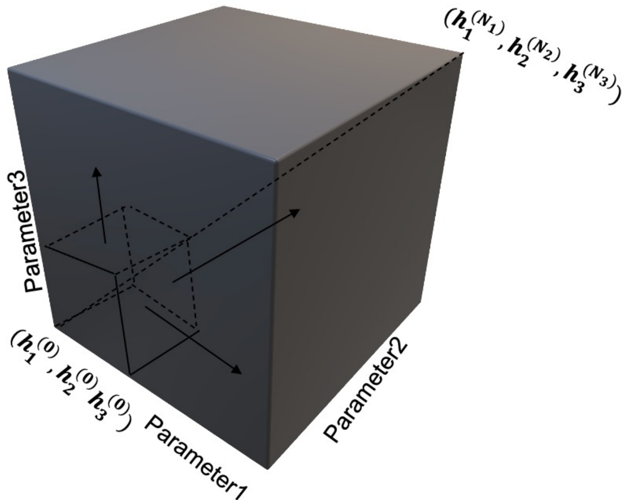
Figure 3.2: 3-D Case
