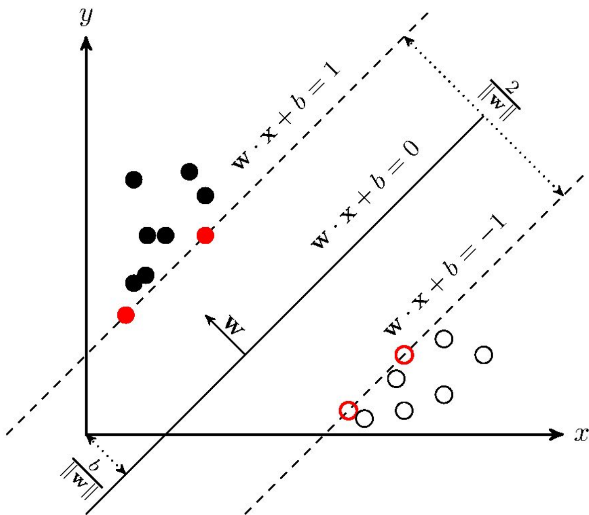
Figure 1.4: SVM
