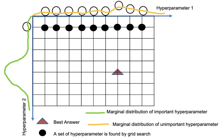
(a) Grid search
