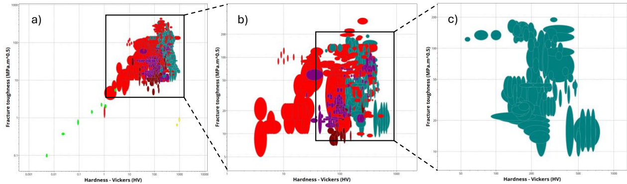
Figure 2. Candidate pool of a) all metals, b) castable metals, and c) castable Fe-C alloys [7].
