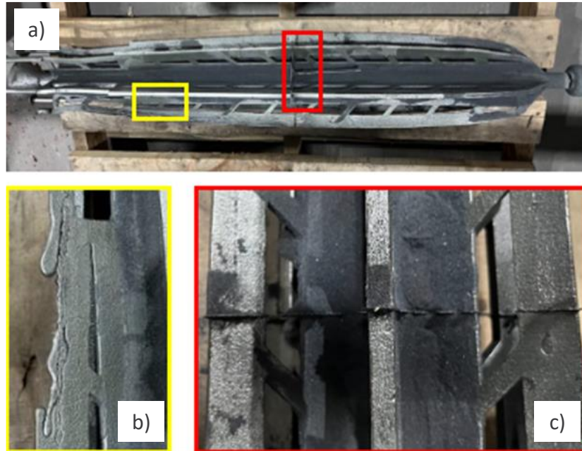
Figure 26. Casting failures seen a) on the whole cast structure, b) on the thinnest blade, and c) as misalignment.
