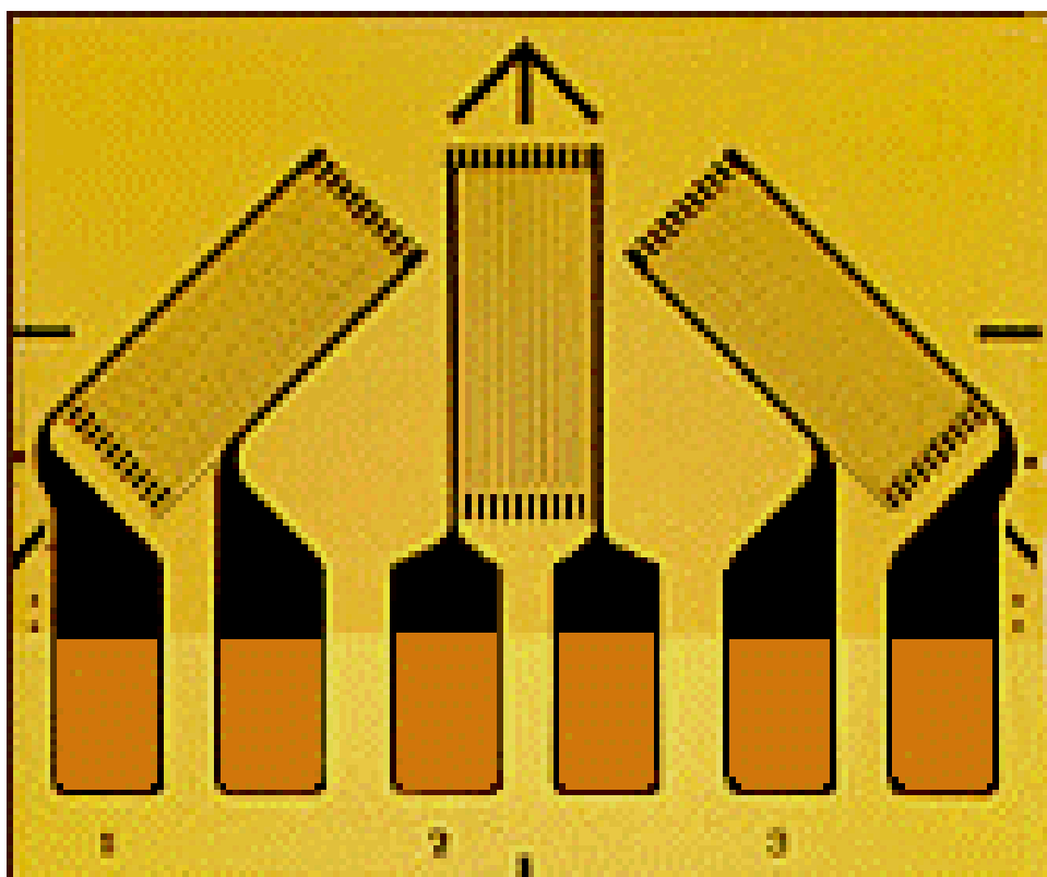
Figure B8. A 45-degree Strain Gage Rosette.
