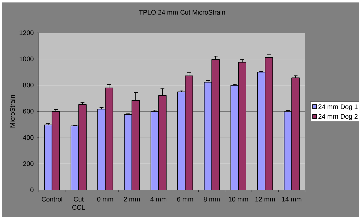
Figure B21. TPLO 24 mm Cut MicroStrains.
