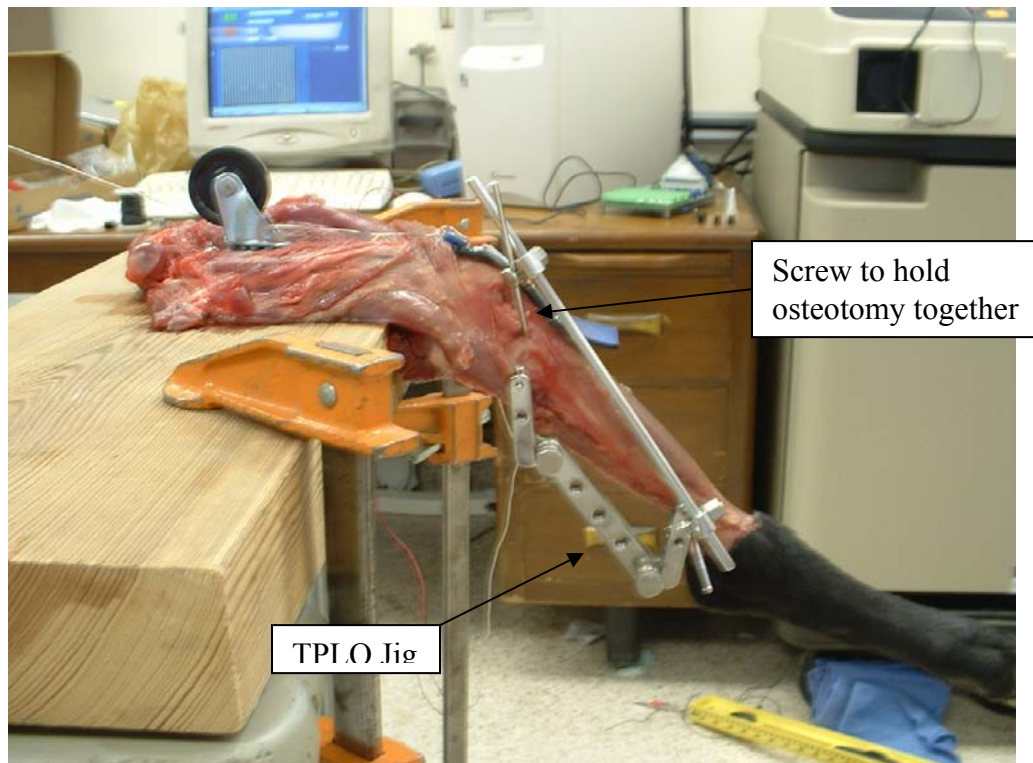
Figure B18. Bone Plate Substitute for TPLO.
