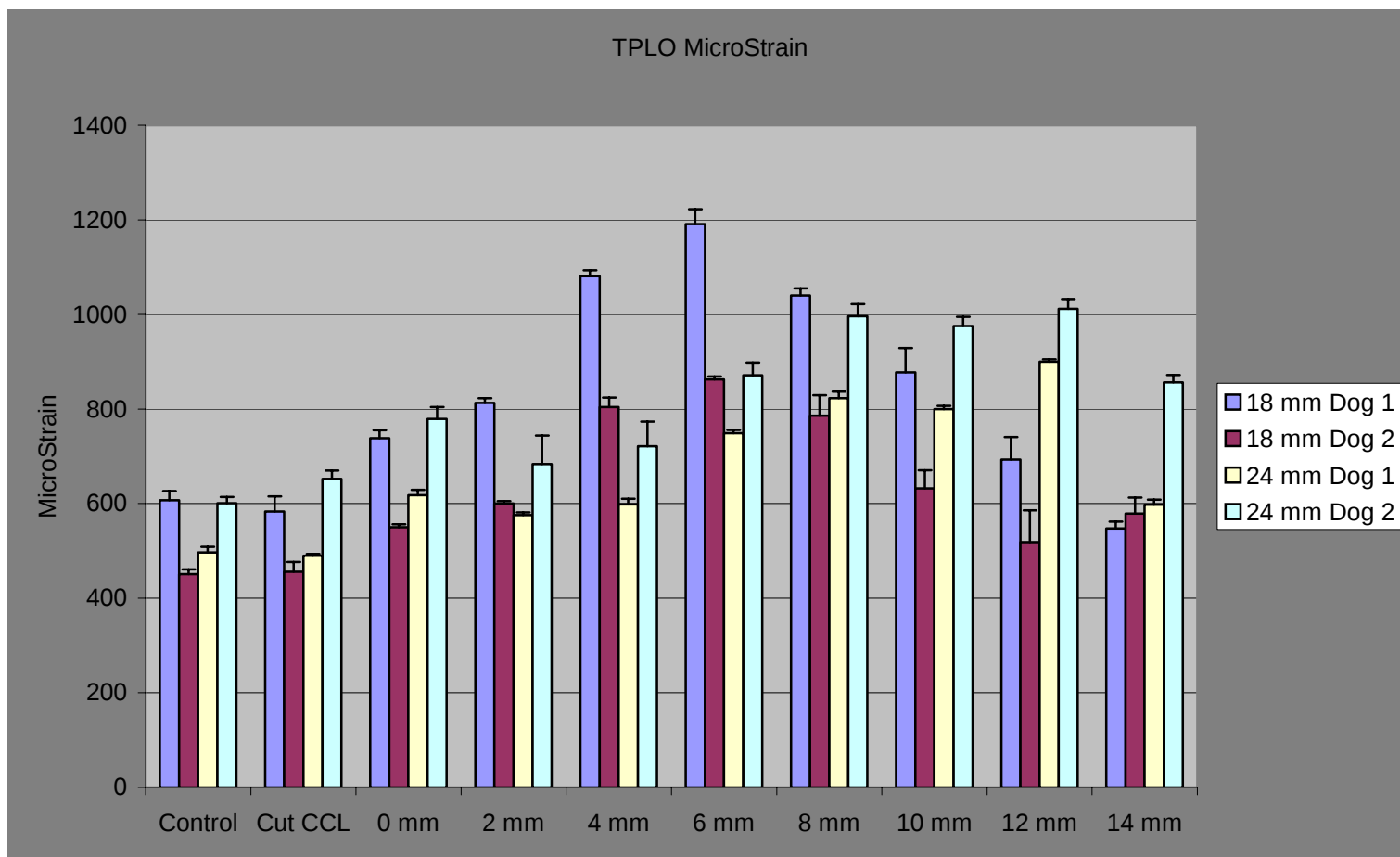
Figure B19. TPLO MicroStrains.
