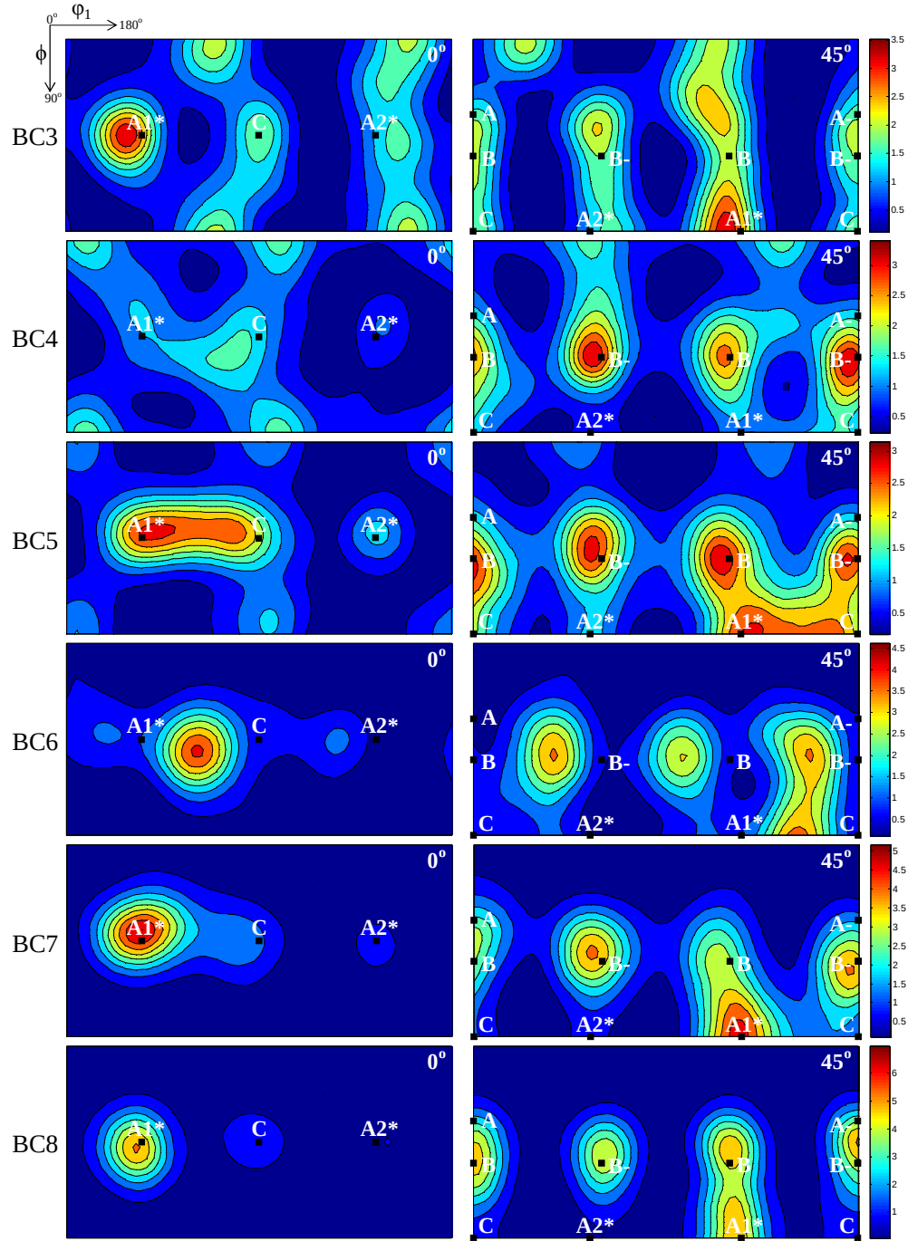
Figure 5.5. Orientation distribution function (ODF) sections ( \phi_2 = 0^\circ and \phi_2 = 45^\circ ) showing the qualitative texture evolution of the fcc austenite under biaxial torsion/compression as a function of equivalent strain from BC3 to BC8.
