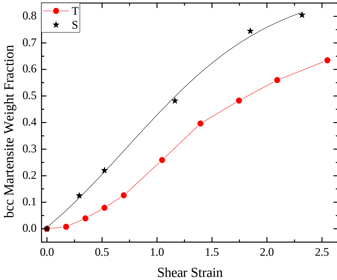
Figure 5.3. bcc martensite phase evolution as a function of applied shear strain under stepwise tension-torsion (S) in comparison to tension (T). The only difference between the two cases are that the S specimens were subjected to a uniaxial tensile 'pre-strain' of about 0.13 before the subsequent torsion.
