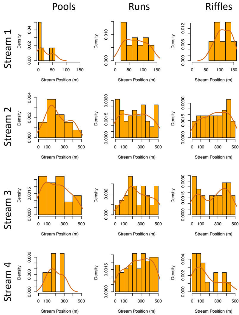
Figure S6: Frequency histograms and kernel density plots of the linear position of stream habitats across each of four replicate contact zones.
