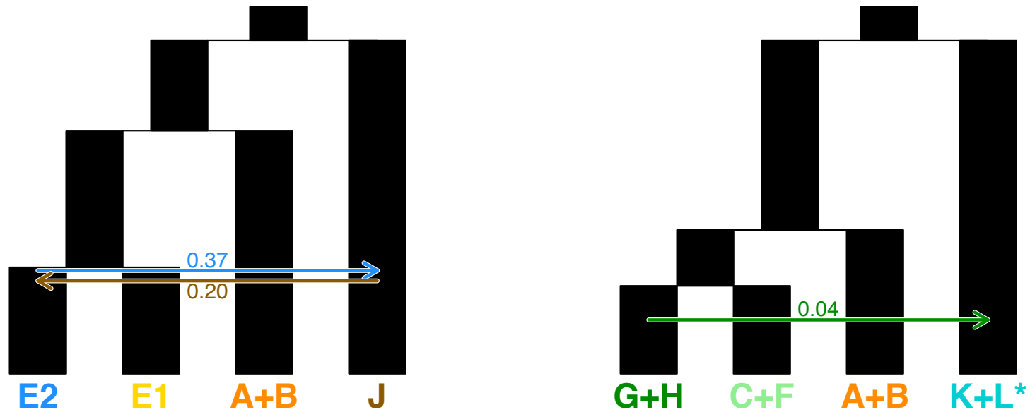
Figure 8: Best migration models as inferred from coalescent simulations in fastsimcoal2 . Arrows represents migration in a coalescent framework (i.e., the reverse of forward-time), and are labeled with migration estimates. Bar heights represent relative coalescent times. Colors correspond to major lineages as explained in the Results .
