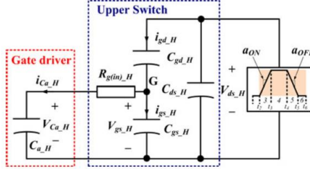
(a) Simplified equivalent circuit of synchronous switch during switching of active switch
