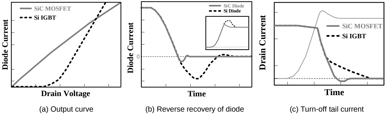
Fig. 7. IGBT shortcomings
