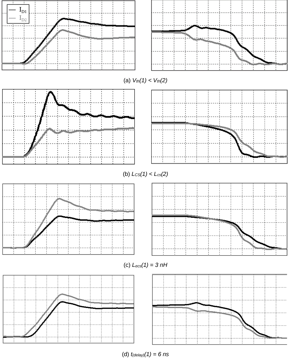
Fig. 29. Dynamic current sharing between two devices with varying parameters (left) turn-on (right) turn-off
