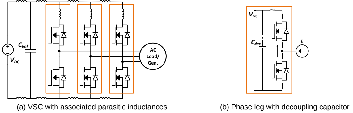
Fig. 13. Parasitic inductances inherent in VSC
