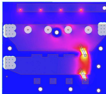
(d) Position 4 top (left) and bottom (right) current distribution with 7.04 nH
