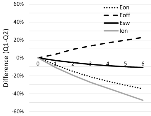
(c) Variation in equivalent L_{ecs}(1)
