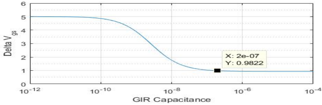
Fig. 54. Induced gate voltage as a function of C_{gir}
