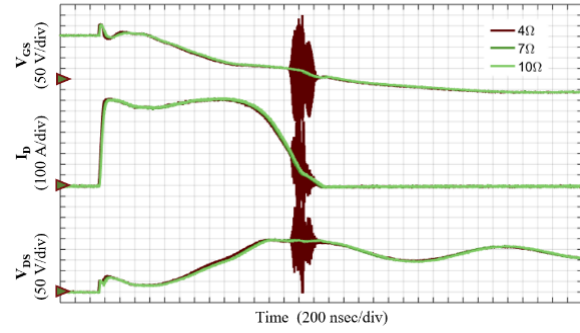
(b) Experimental short-circuit turn-off tests
