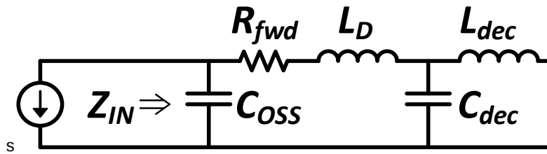
Fig. 14. Small signal equivalent circuit of power loop
