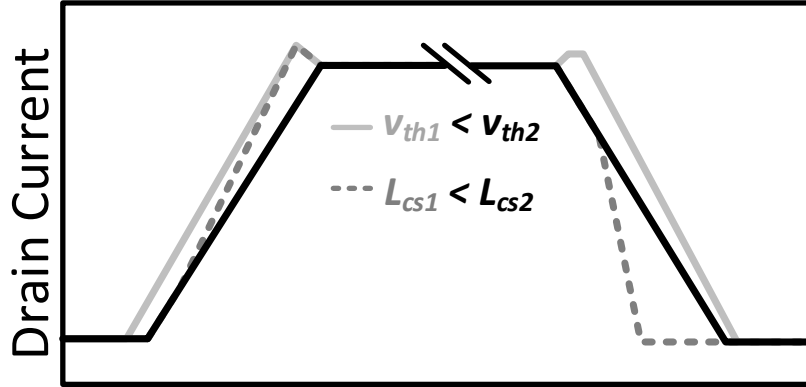
Fig. 9. Effects of V_{th} and L_{cs} variation on dynamic current sharing in parallel devices
