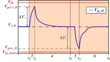
(b) Effect of induced gate current on synchronous gate voltage
