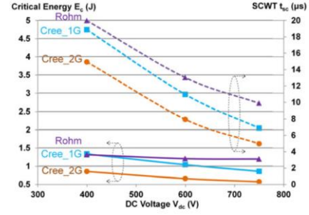
(b) DC bus voltage dependency
