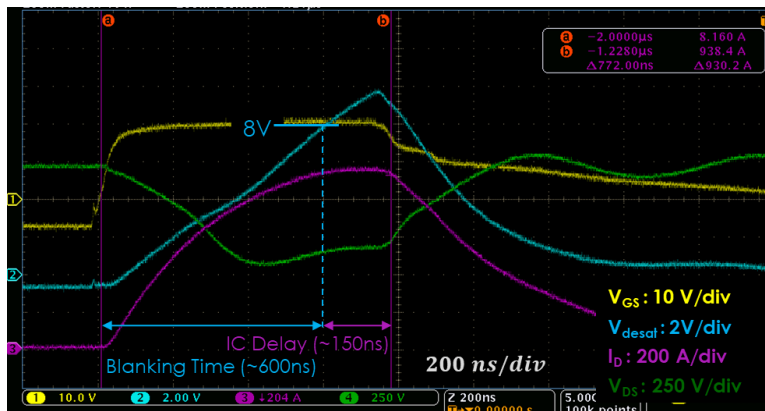
Fig. 39. Hard switching fault detection and turn off with single MOSFET
