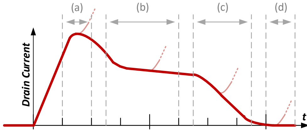
Fig. 18. Short-circuit current waveform and failure modes for both IGBTs and MOSFETs
