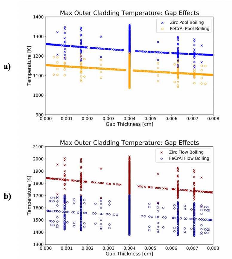
Figure 47. Maximum outer cladding temperature relationship to gap thickness in the Zircaloy and FeCrAl rodlets under a) pool boiling and b) flow boiling conditions. All cases experienced DNB.
