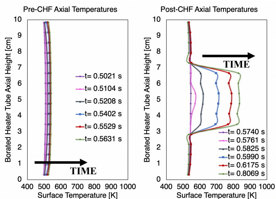
Figure 24. Pre-and-post CHF axial cladding temperatures for the borated heater tube as a result of application of power pulse in TREAT.
