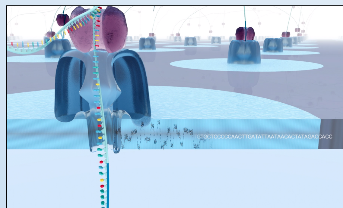
Figure 4: Nanopore sequencing graphic. 2
