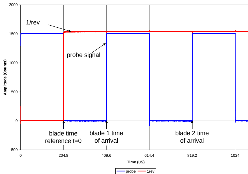
Figure 12. Stable input source probe and 1/rev signals
