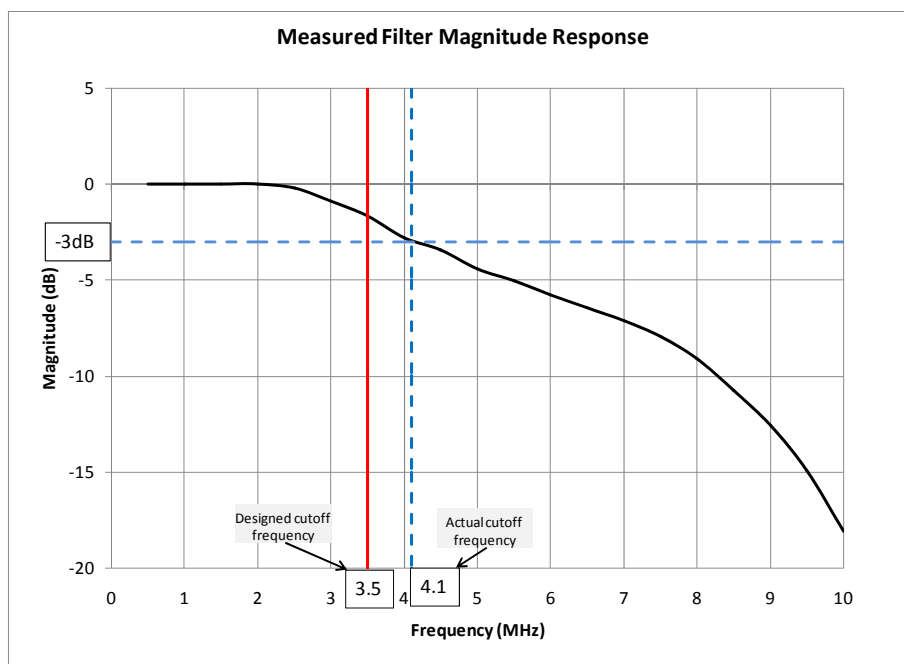
Figure 16. Measured magnitude response for the second order Bessel low-pass filter as implemented
