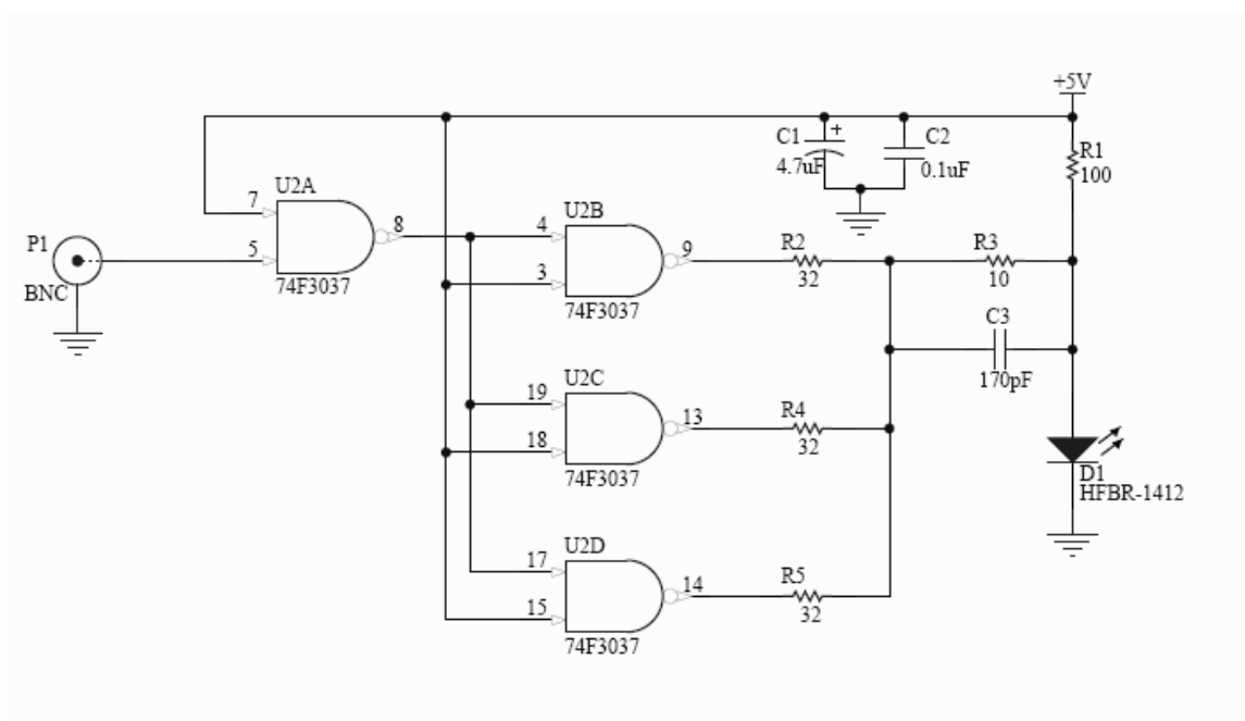
Figure 11. High speed fiber optic transmitter
