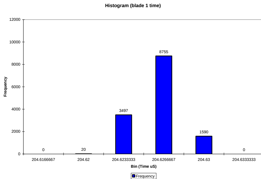
Figure 17. Histogram of Blade 1 time of arrival measurement
