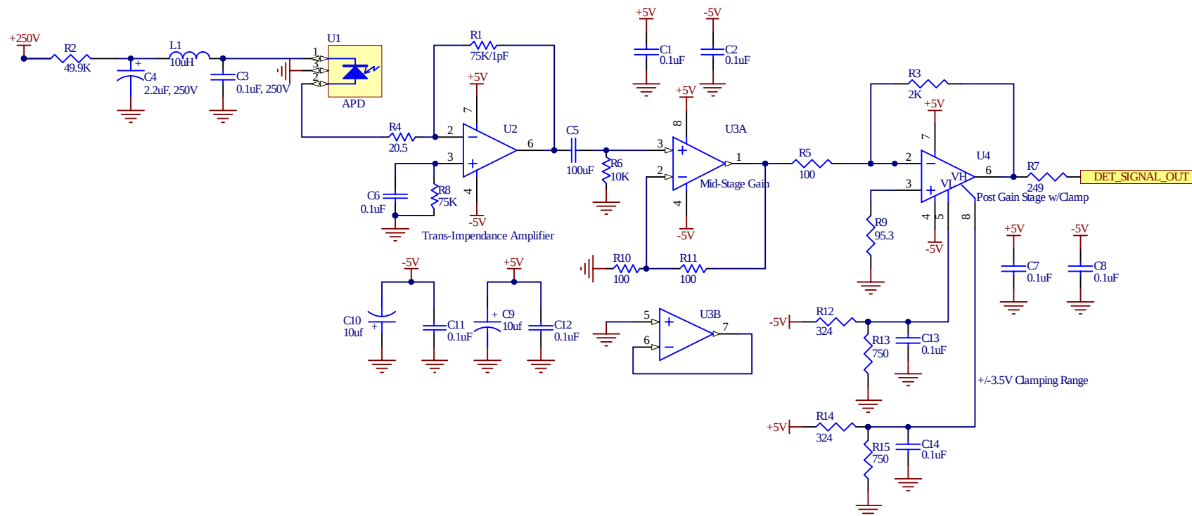
Figure 5. Photo-detector system schematic
