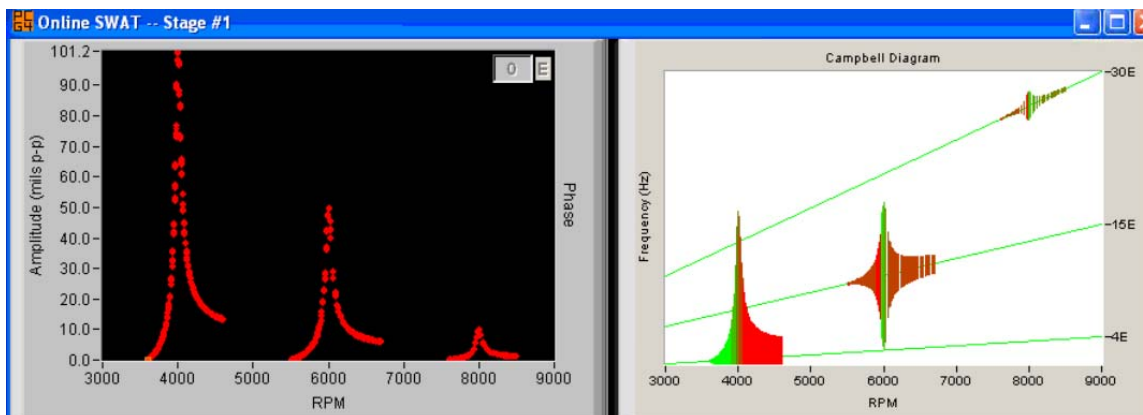
Figure 3. Online screenshot displaying blade deflection amplitude, frequency, and phase from simulated data
