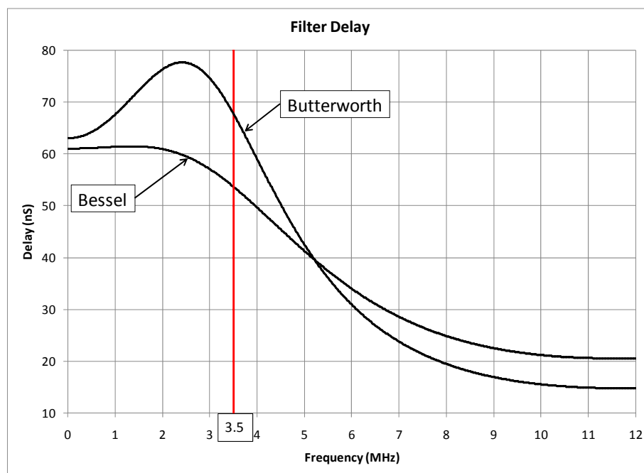
Figure 14. Comparison of group delay for the second order Butterworth and Bessel low-pass filters
