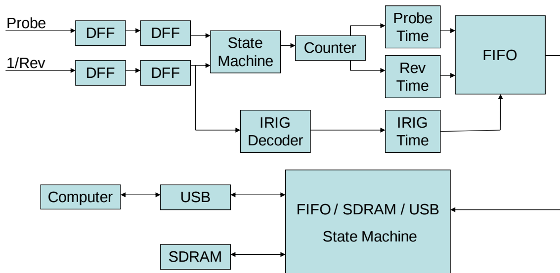
Figure 10. High speed counter design block diagram
