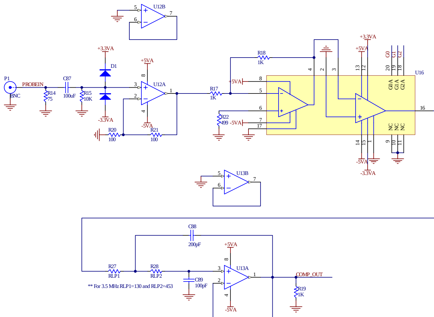
Figure 6. Analog signal conditioning schematic including variable gain amplifier and low-pass filter Approved for public release; distribution is unlimited.
