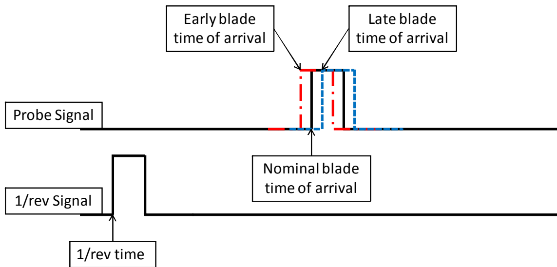
Figure 2. Example of NSMS time of arrival basics
