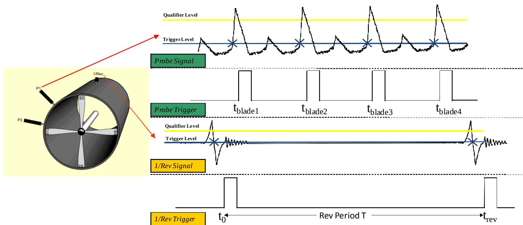
Figure 1. Example of NSMS measurement signals
