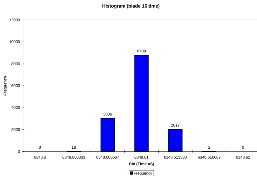
Figure 19. Histogram of Blade 16 time of arrival measurement
