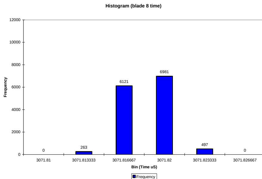
Figure 18. Histogram of Blade 8 time of arrival measurement
