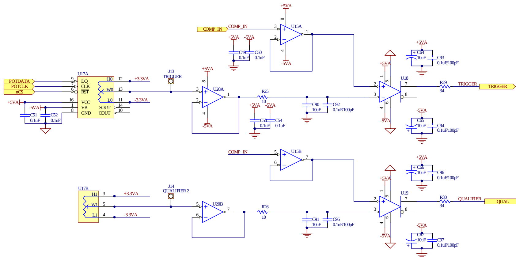
Figure 7. Analog signal conditioning schematic including trigger and qualifier comparators
