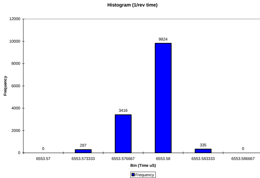
Figure 20. Histogram of 1/rev time of arrival measurement
