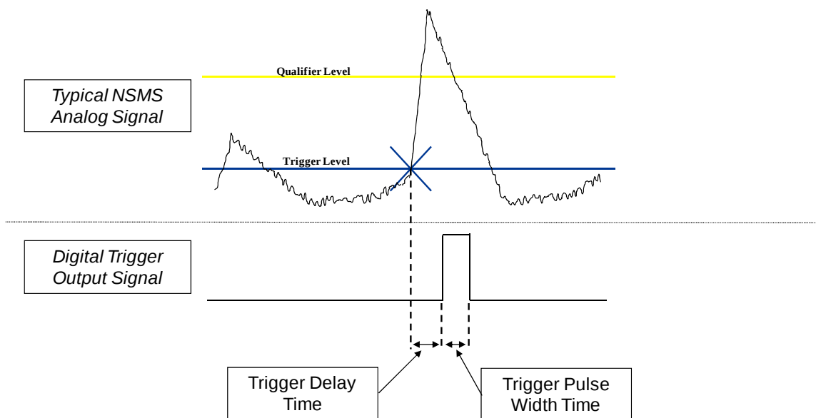
Figure 9. Illustration of trigger and qualifier levels including trigger delay and trigger pulse width
