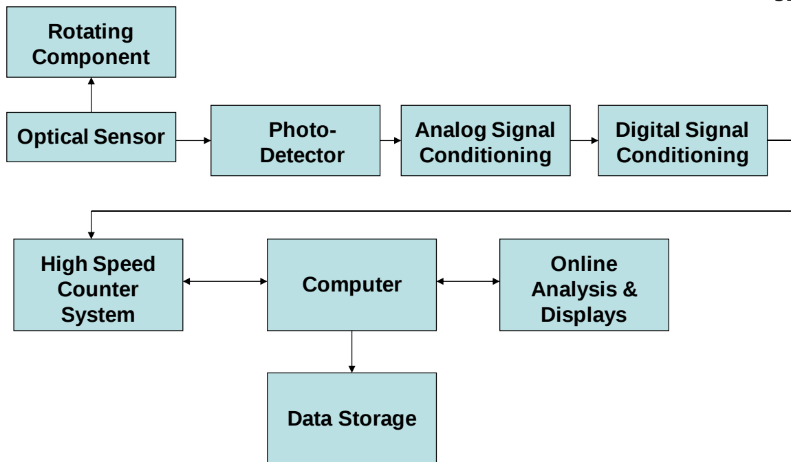
Figure 4. Overall system block diagram
