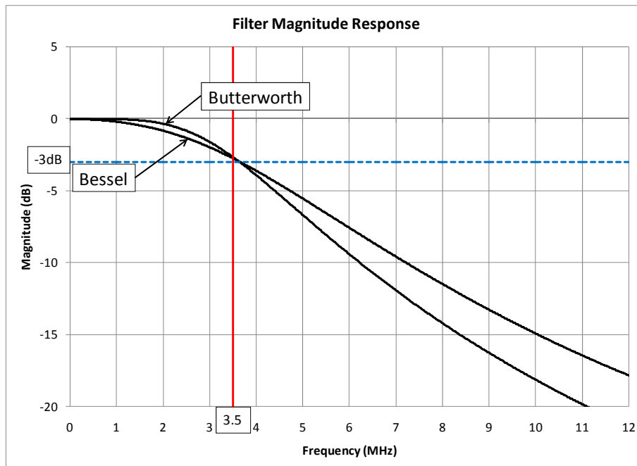
Figure 15. Comparison of magnitude response for the second order Butterworth and Bessel low-pass filters
