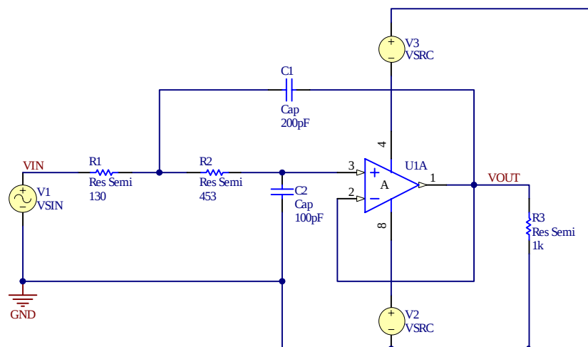
Figure 13. Low-pass filter P-SPICE simulation schematic
