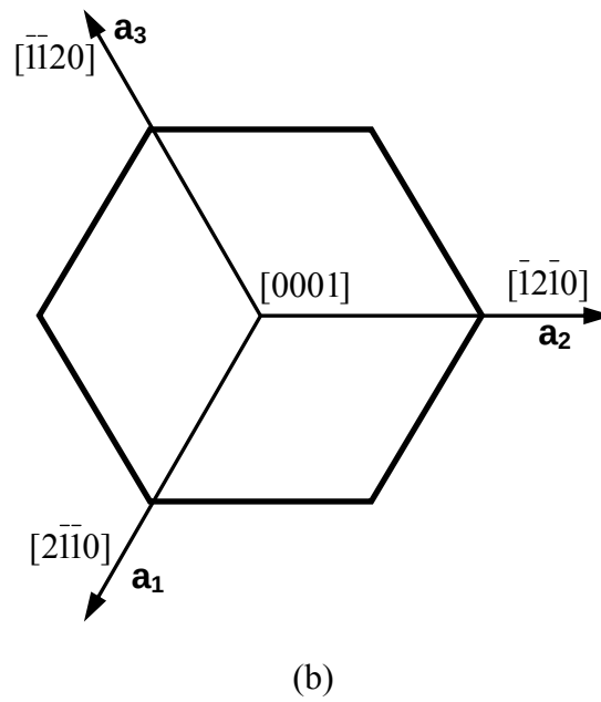
Figure 1.1. Structure of a hcp crystal [6, 8].
