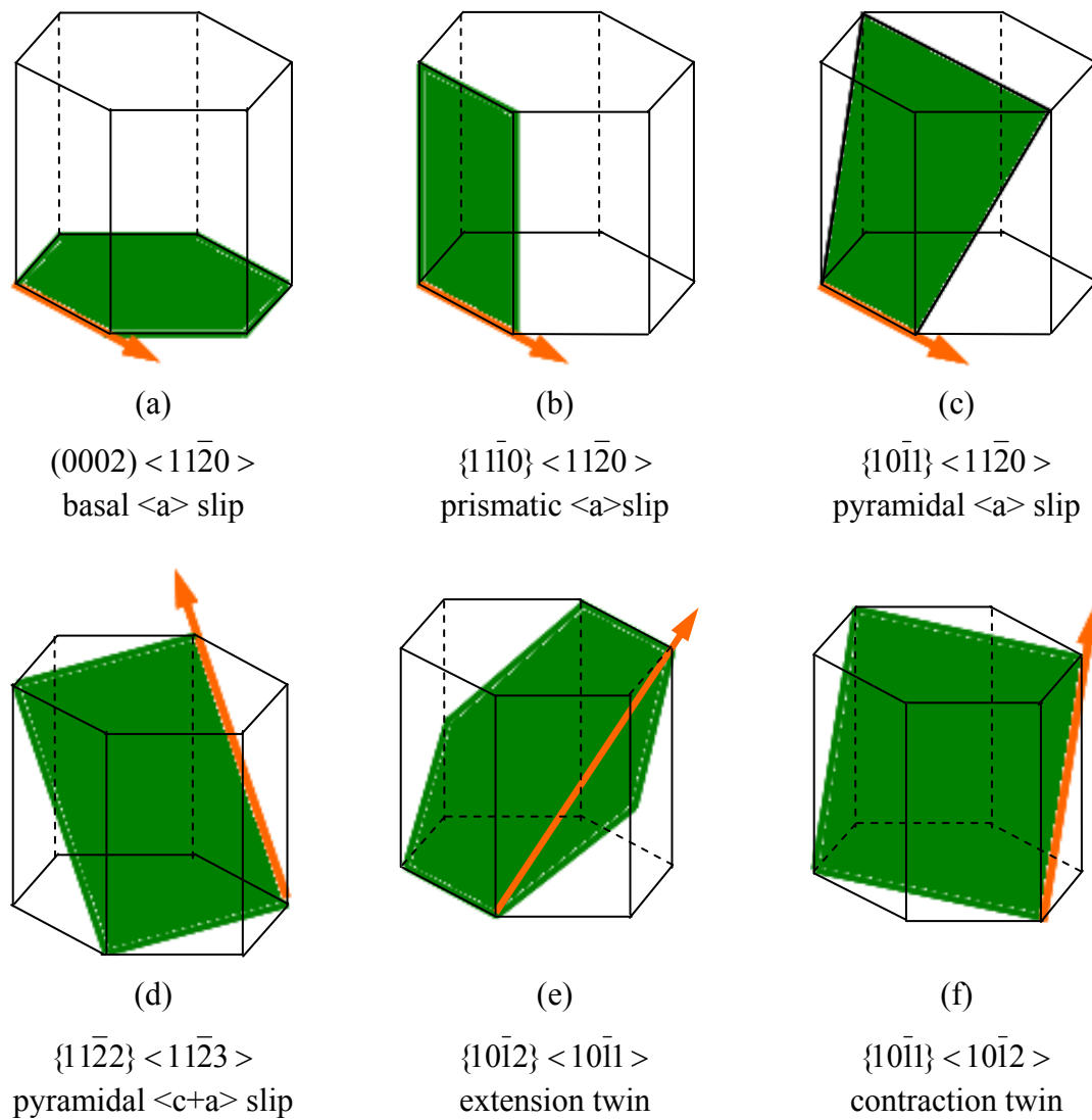
Figure 1.2. Potential deformation systems in magnesium [8, 9, 11].
