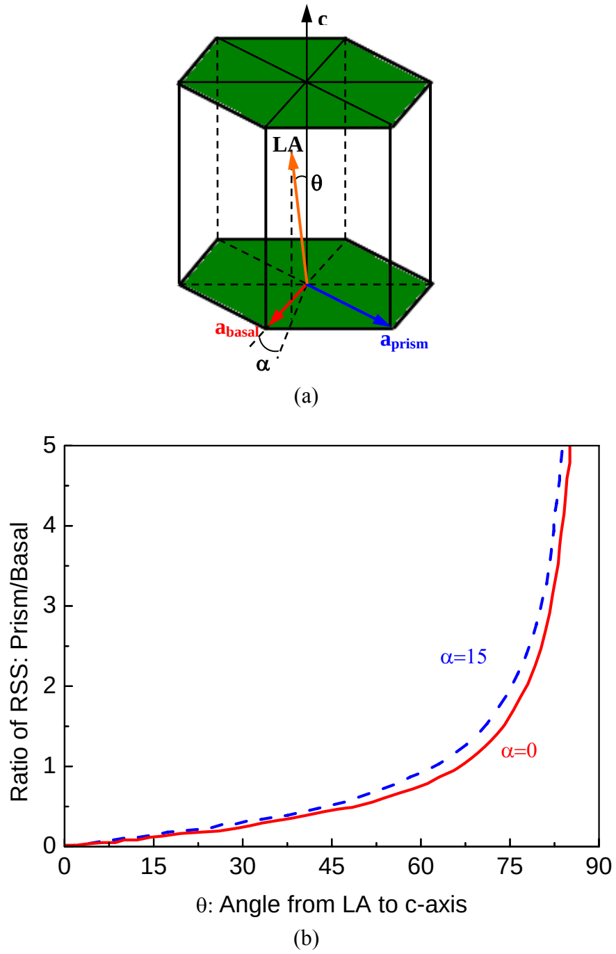
Figure 1.9. a) Schematic of single crystal under uniaxial loading; (b) Variation of the ratio of resolved shear stress (RSS) between prismatic and basal \langle a \rangle slips with an angle between the loading axis (LA) and c-axis [29].
