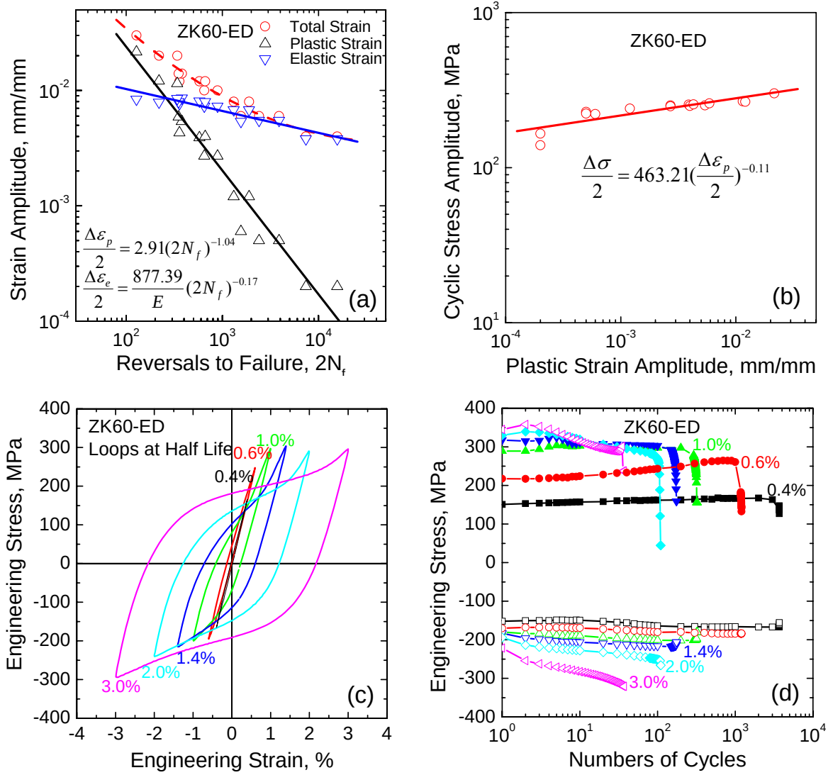
Figure 5.1. The low-cycle fatigue behavior of the as-extruded ZK60A alloy under the ED loading: a) \epsilon -N fatigue life curves; b) cyclic stress and strain curves; c) hysteresis loops at half life for various total strain amplitudes; and d) cyclic tensile and compressive peak stress responses.
