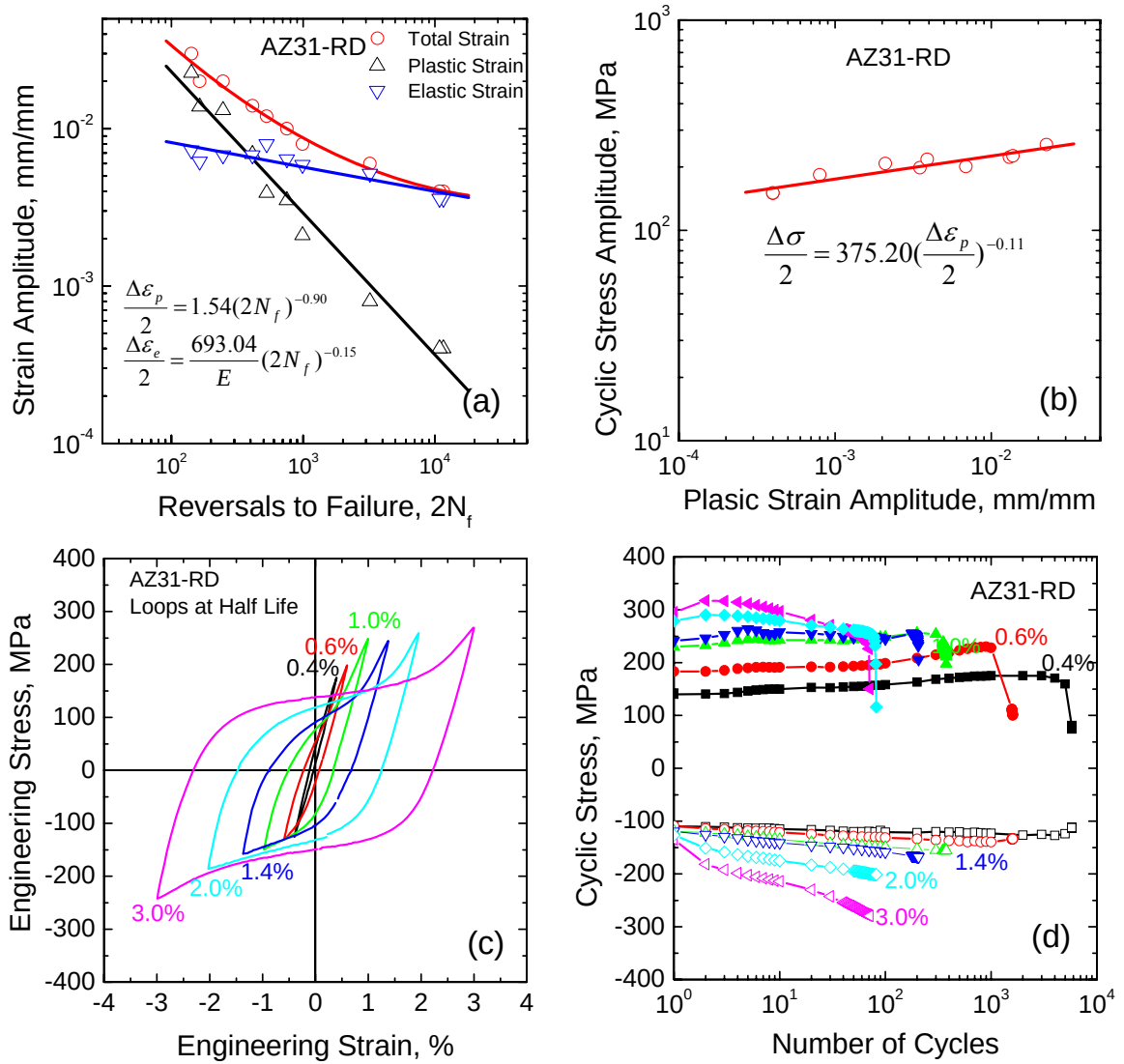
Figure 5.5. The low-cycle fatigue behavior of the as-rolled AZ31B alloy under the RD loading: a) \epsilon - N fatigue life curves; b) cyclic stress and strain curves; c) hysteresis loops at half life for various total strain amplitudes; and d) cyclic tensile and compressive peak stress responses.
