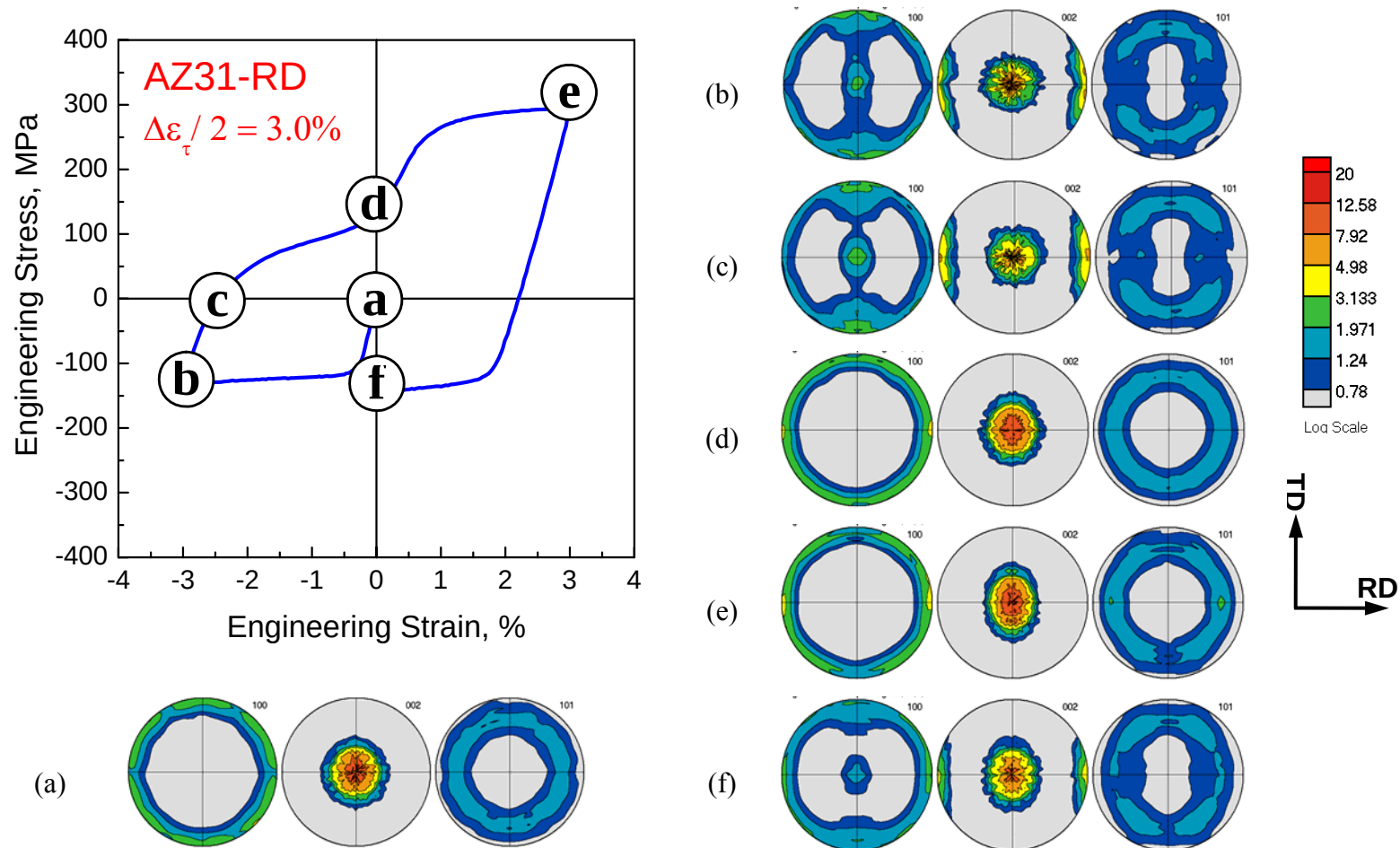
Figure 5.34. Measured crystallographic textures along the hysteresis loop during the first cycle deformation using ex situ synchrotron diffraction: a) strain-free, b) – 3.0 % strain, c) 0 MPa stress, d) 0 % strain, e) + 3.0 % strain, and f) 0 % strain. Pole densities are expressed in multiples of a random distribution (mrd). The loading axis (along RD) is horizontally right.
