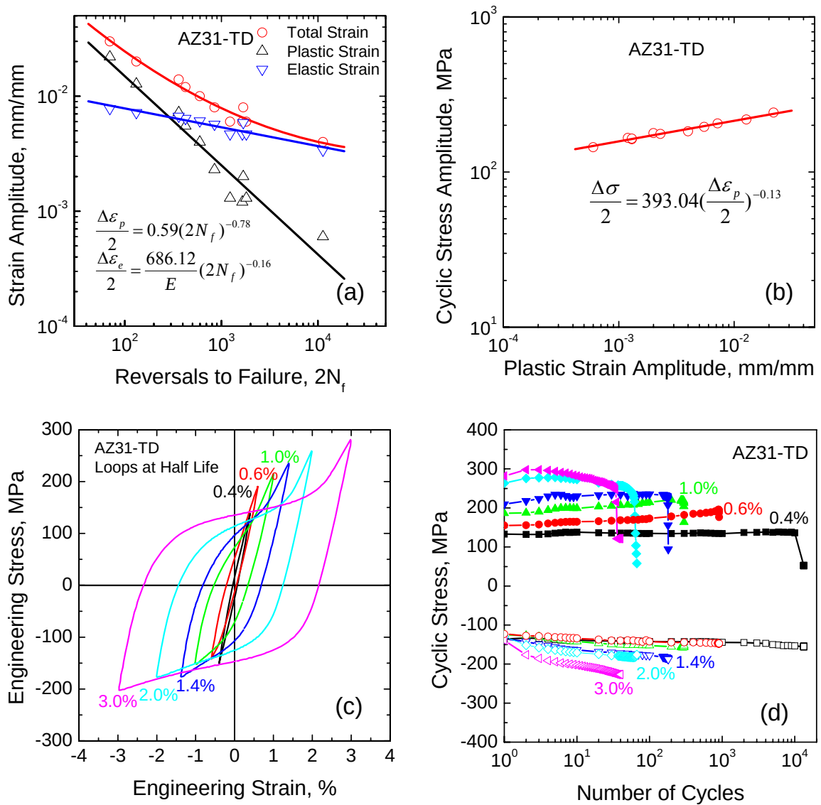
Figure 5.6. The low-cycle fatigue behavior of the as-rolled AZ31B alloy under the TD loading: a) \epsilon - N fatigue life curves; b) cyclic stress and strain curves; c) hysteresis loops at half life for various total strain amplitudes; and d) cyclic tensile and compressive peak stress responses.
