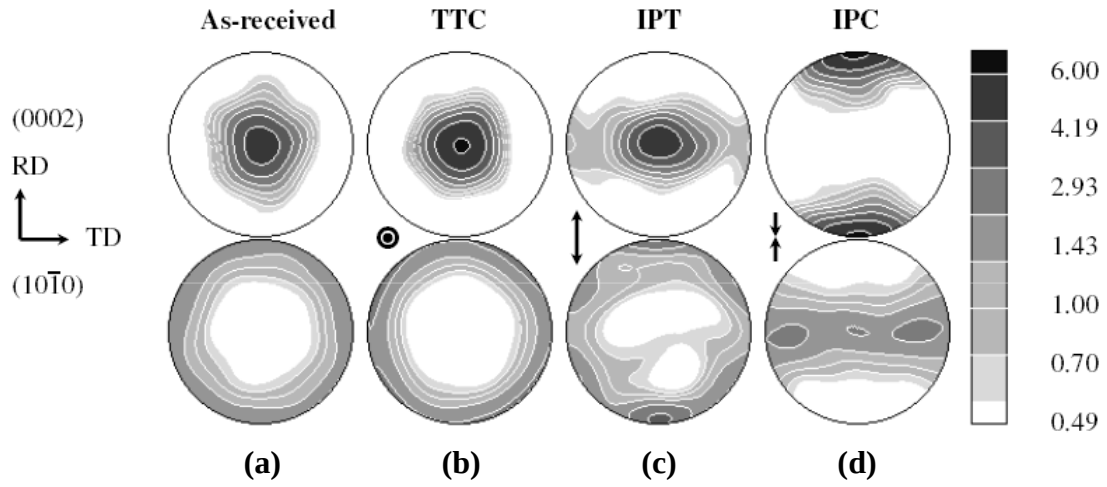
Figure 2.6. Basal and prismatic pole figures from the (a) as-received plate, (b) through-thickness compressed, (c) in-plane tensile tested, and (d) in-plane compressed samples. Arrows in (b), (c), and (d) denote the stress direction in the same coordinate system [36].
