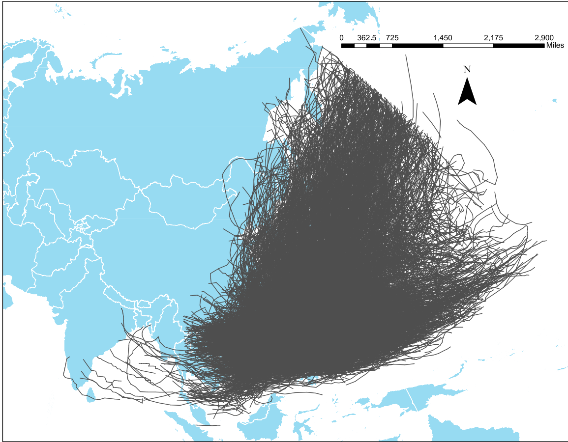
Figure 1b. Western Pacific TC tracks from IBTrACS spanning 1964 to 201 (n = 54,777).
