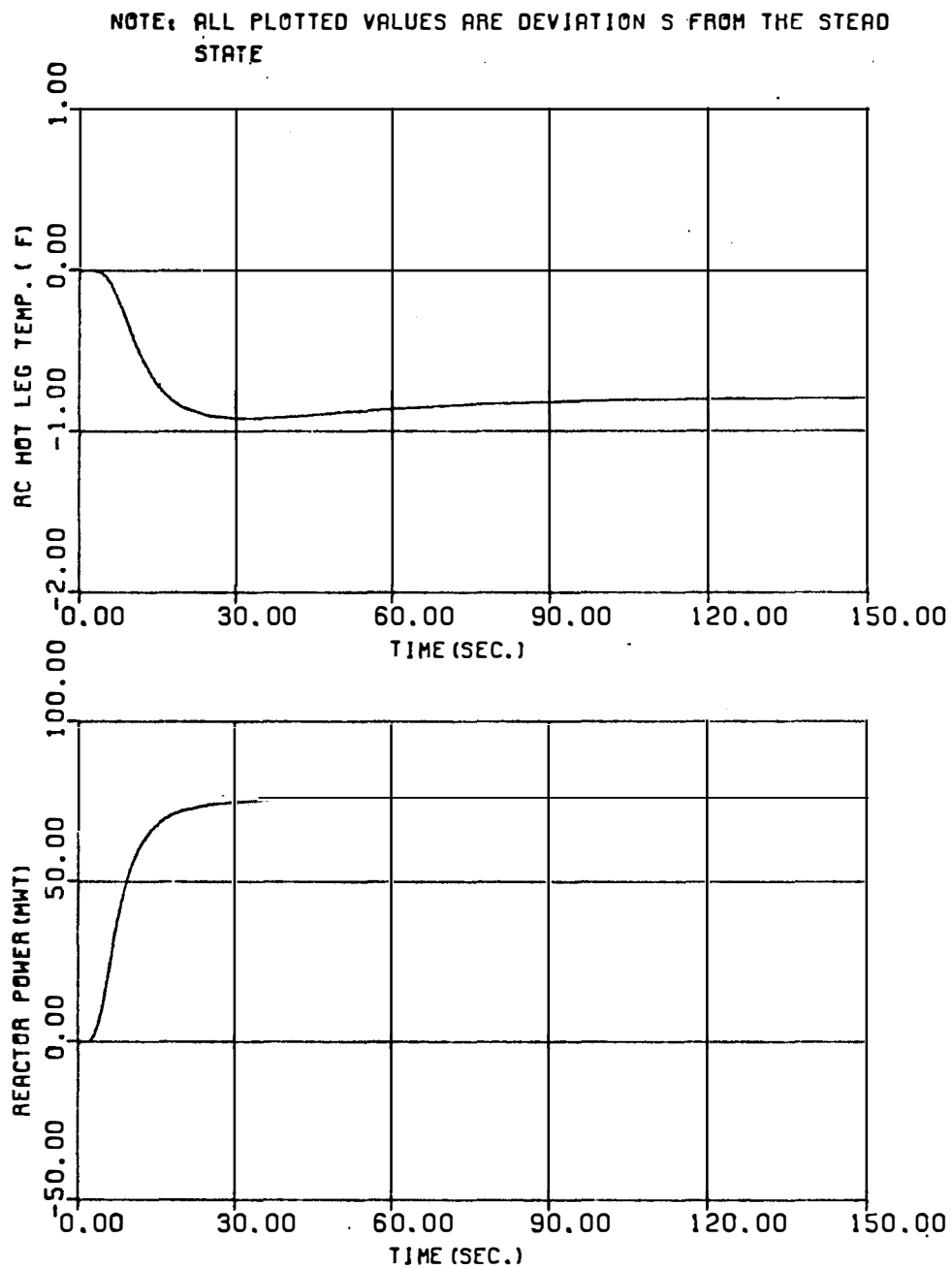
FIGURE D-4. TRANSIENT RESPONSE OF THE SYSTEM FOR 50 PSI STEP CHANGE IN THE TURBINE (1-ST STAGE) PRESSURE
