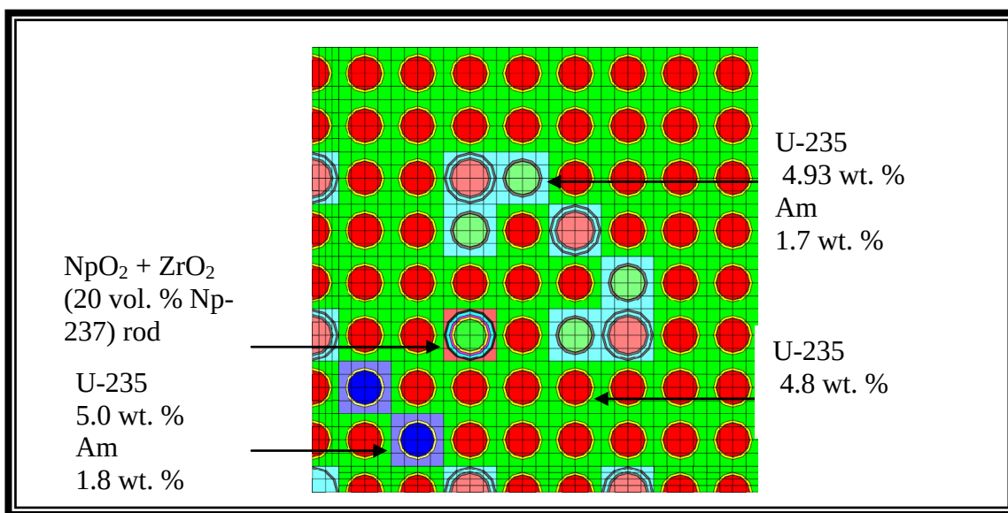
Figure 4:17 Optimized lattice with \text{NpO}_2 and low Am content
