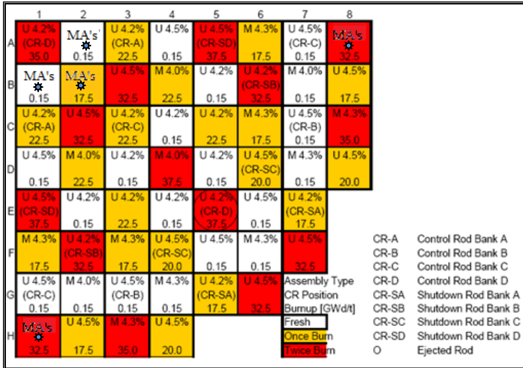
Figure 6:8 Central loading strategy with 4 fresh bundles with MAs
