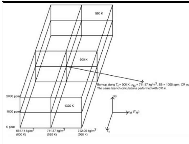
Figure 6:2 3D diagram of lattice physics branches (Kozlozwki et al. 2007)
