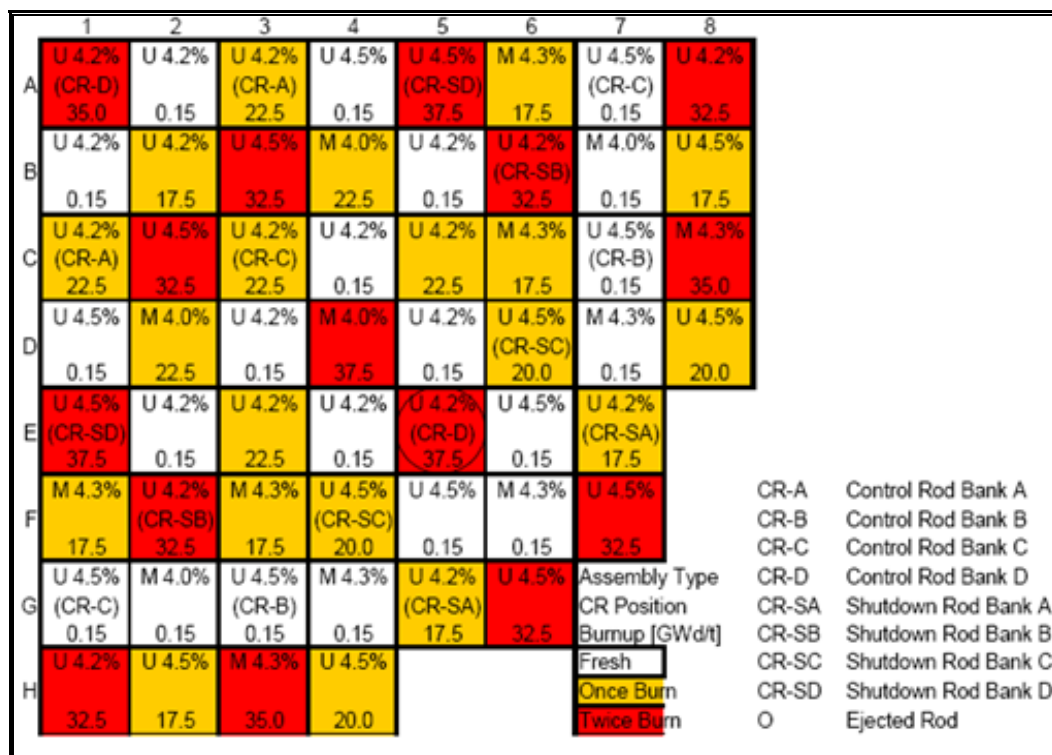
Figure 6:1 OECD benchmark core radial loading pattern (Kozlowski et al. 2006)
