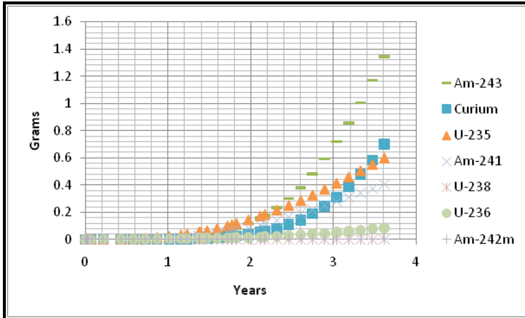
Figure 7:5 Near negligible radioisotopes in \text{NpO}_2 pins versus burnup
