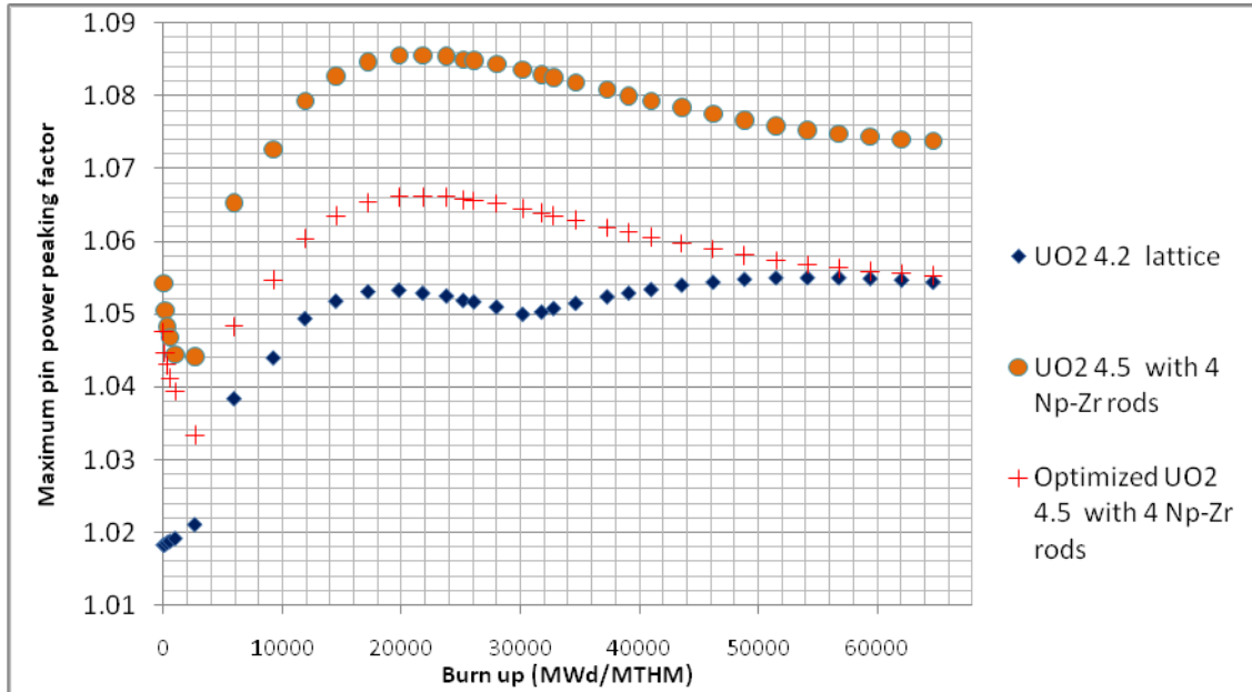
Figure 4:14 FORMOSA-L power peaking minimization for 4.5 w/o U-235 lattice with four \text{NpO}_2 + \text{AmO}_2 rods
