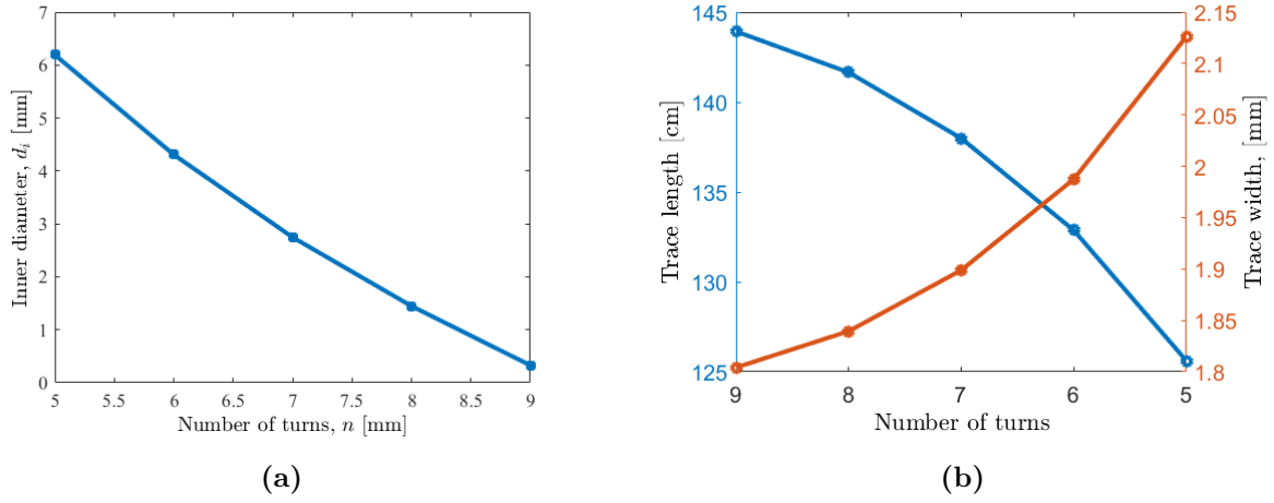
Figure 3.10: Inner diameter (b) and length and width of trace with different n (b).
