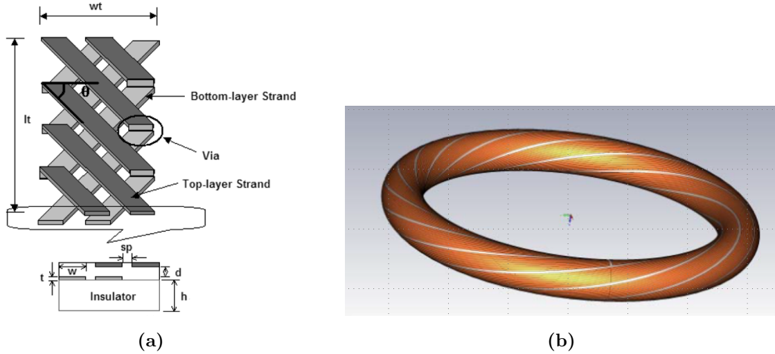
Figure 2.3: Picture showing the schematic of the planar Litz (a) [2], and 3D Litz (b) [3].
