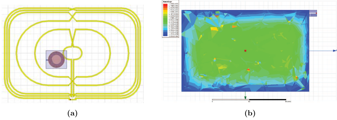
Figure 2.9: Intel coil structure (a) [8] and the uniform surface H-field (b) [9].
