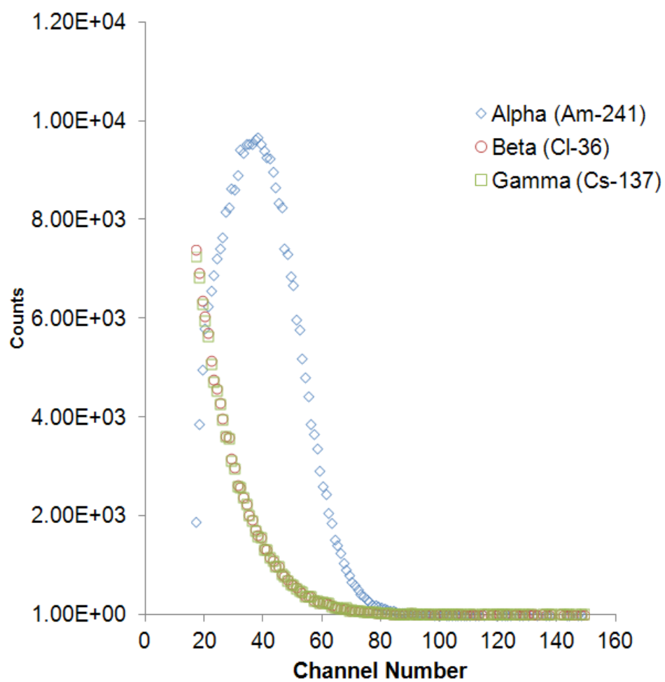
Figure 3.11: Alpha, beta and gamma response for PEN/LiF composite meltspun microfibers.
