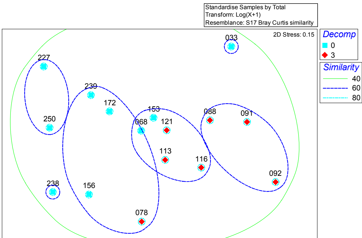
Figure 6-11. Multidimensional scale ordination of Bray-Curtis similarity matrix for decomposition bins None and High showing separation.
