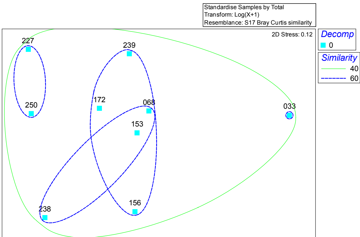
Figure 6-6. Multidimensional scale ordination of Bray-Curtis similarity matrix for decomposition bin None (0).
