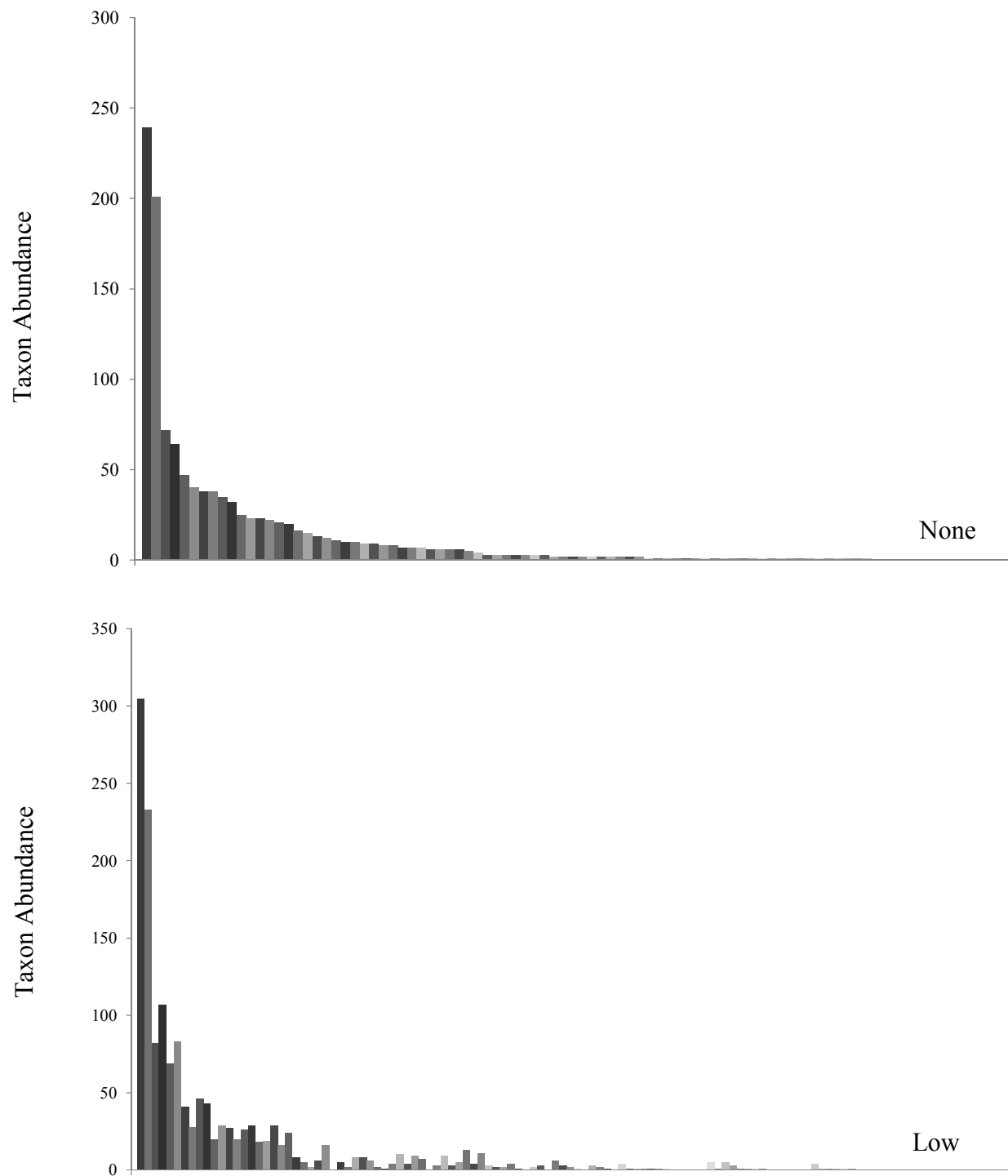
Figure 6-4. Abundance charts for decomposition bins None(top) and Low (bottom) inside the facility. Bin None is set as the reference sample.
