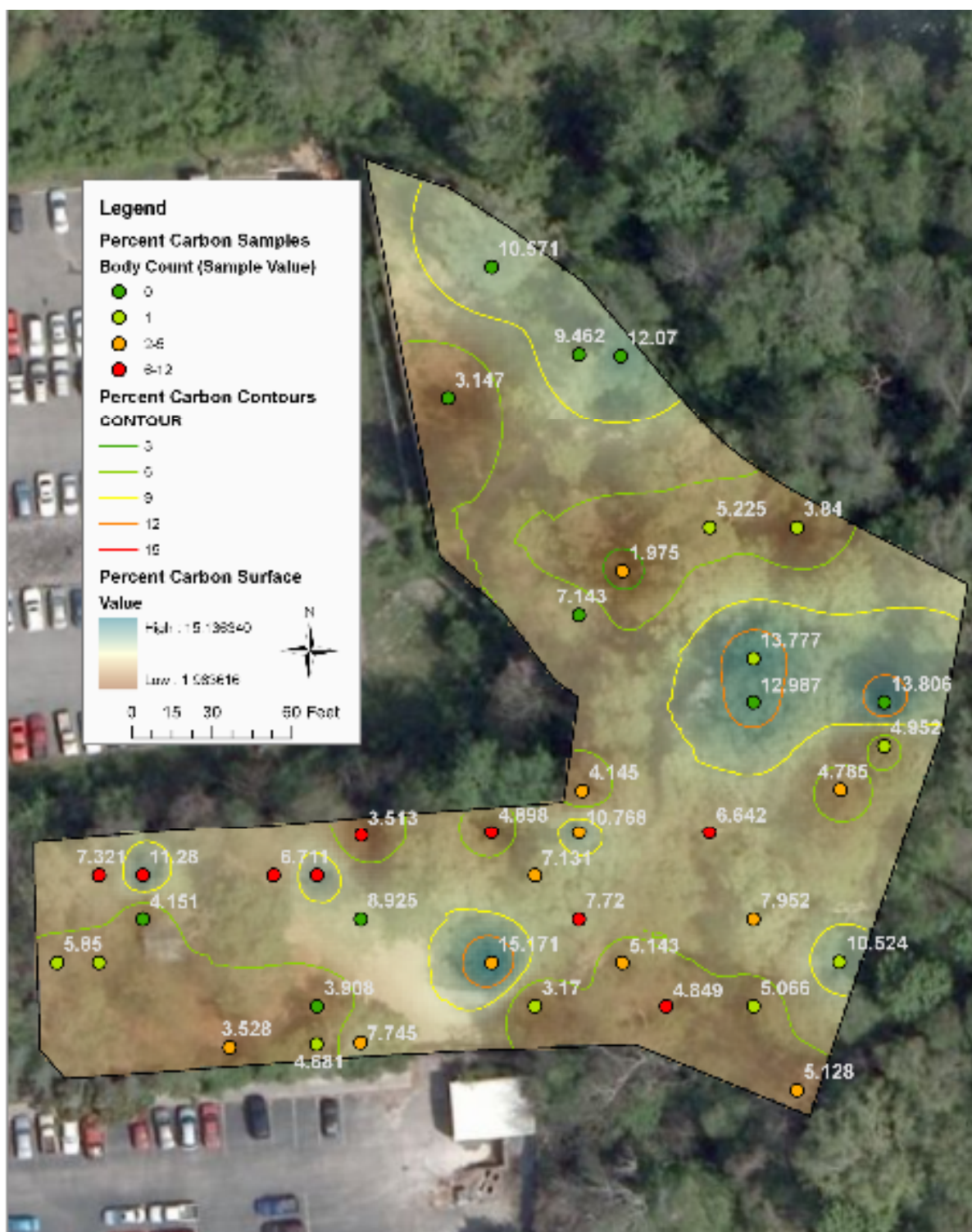
Figure D-4. Distribution of total carbon percent \text{g}^{-1} soil across UT ARF.
