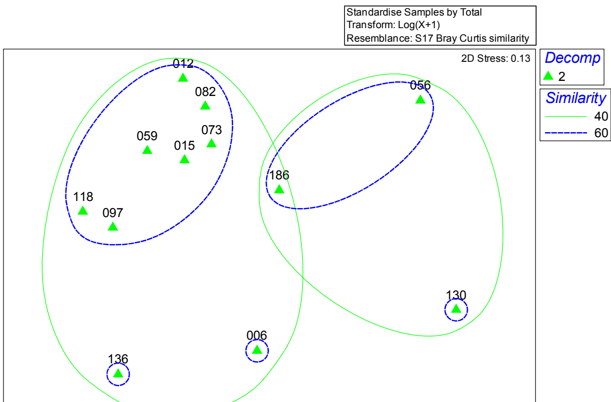
Figure 6-8. Multidimensional scale ordination of Bray-Curtis similarity matrix for decomposition bin Middle (2).
