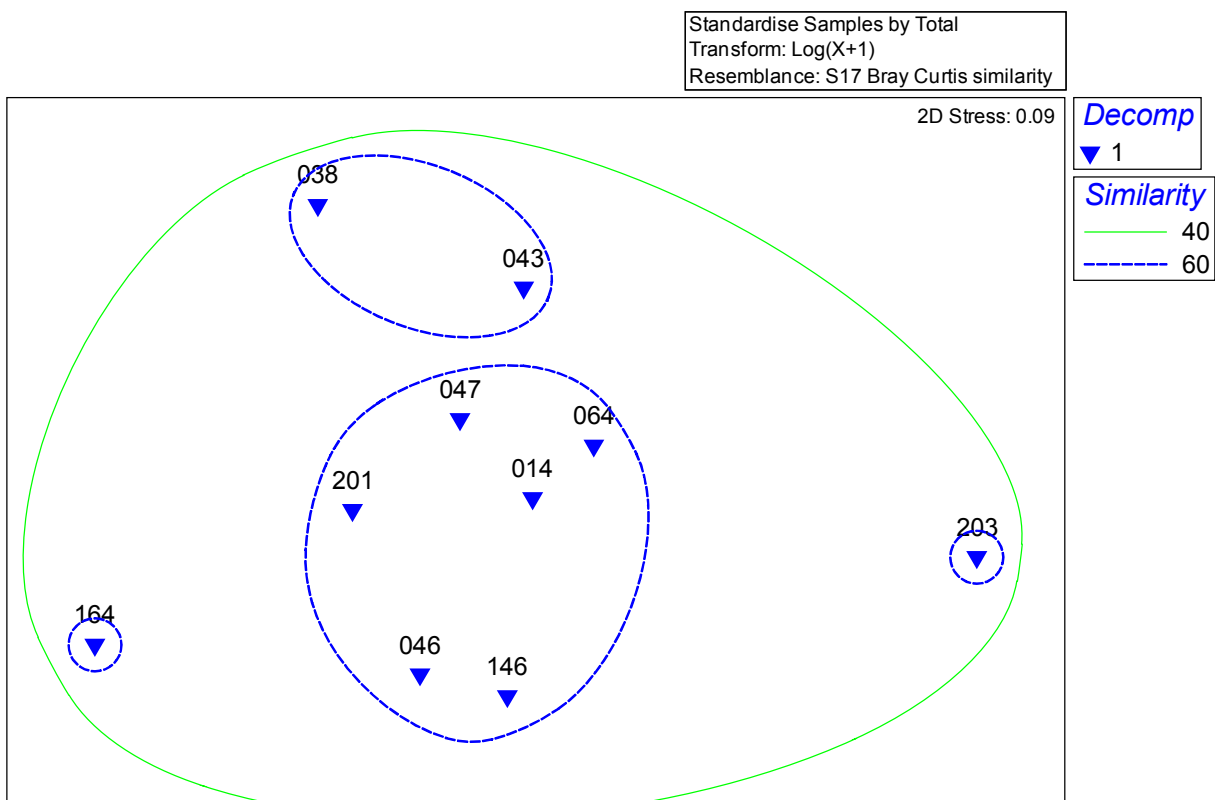
Figure 6-7. Multidimensional scale ordination of Bray-Curtis similarity matrix for decomposition bin Low (1).
