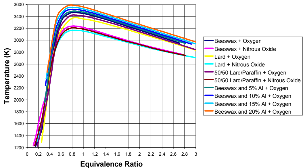
Temperature vs Equivalence Ratio Combustion Chamber Pressure = 150 psig
