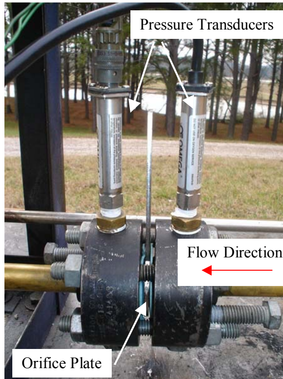
Figure 16: Pressure Transducers and Orifice Plate
