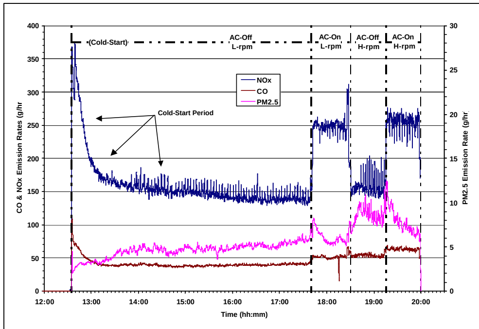
Figure 4.1. Emission rate behavior for 1996 Freightliner truck.
