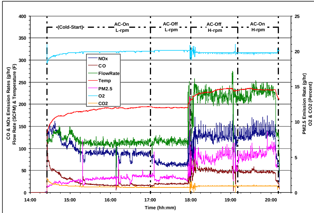
Figure E.9. Emission and flow rate behavior for 2000 Volvo truck (ID#9).
