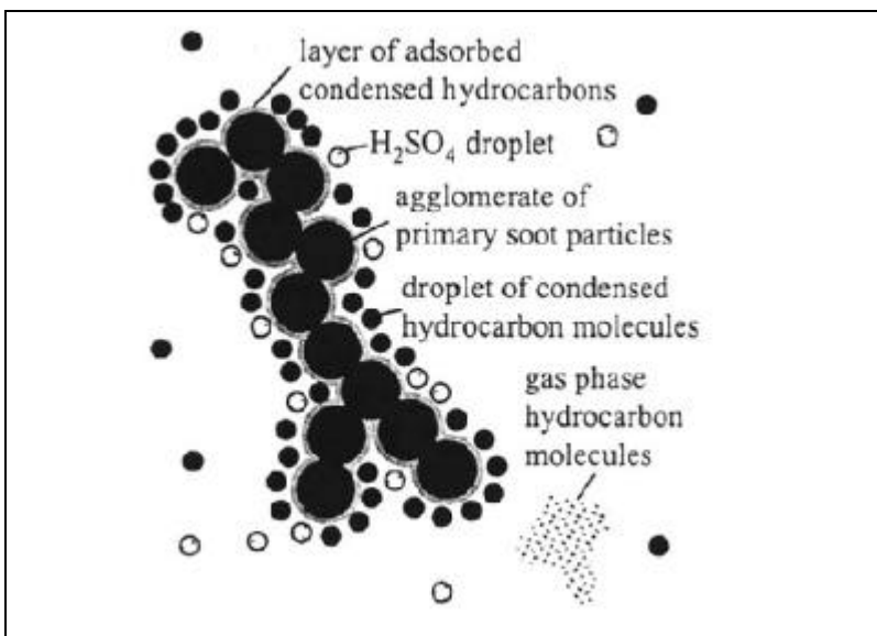
Figure 2.4. Schematic representation of aggregate diesel PM. Source: Walker 31
