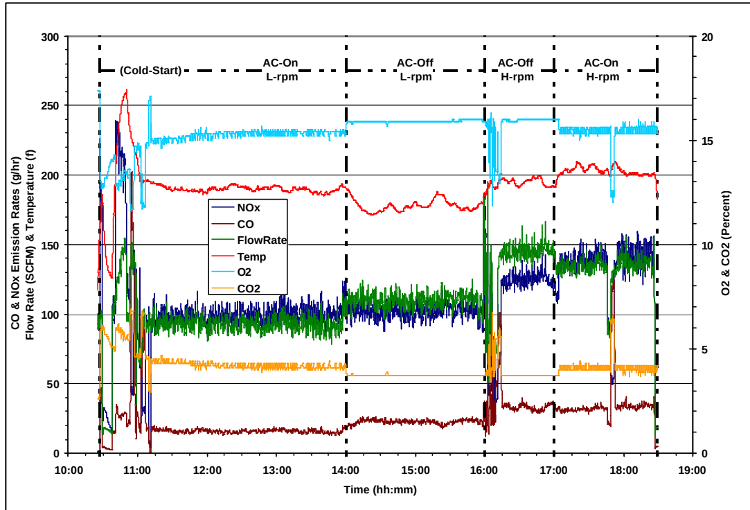
Figure E.3. Emission and flow rate behavior for 2004 Volvo truck (ID#3).
