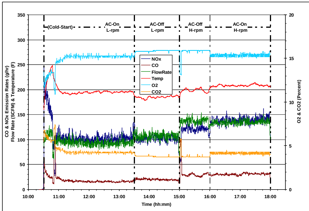
Figure E.4. Emission and flow rate behavior for 2004 Volvo truck (ID#4).
