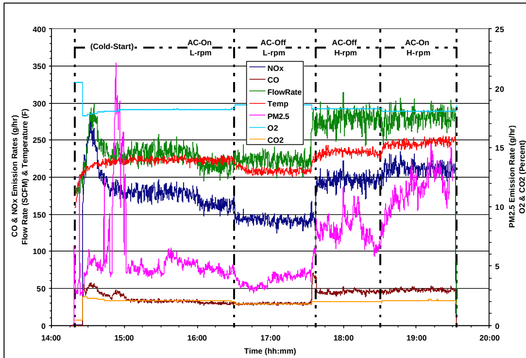
Figure E.10. Emission and flow rate behavior for 1998 Freightliner truck (ID#10).
