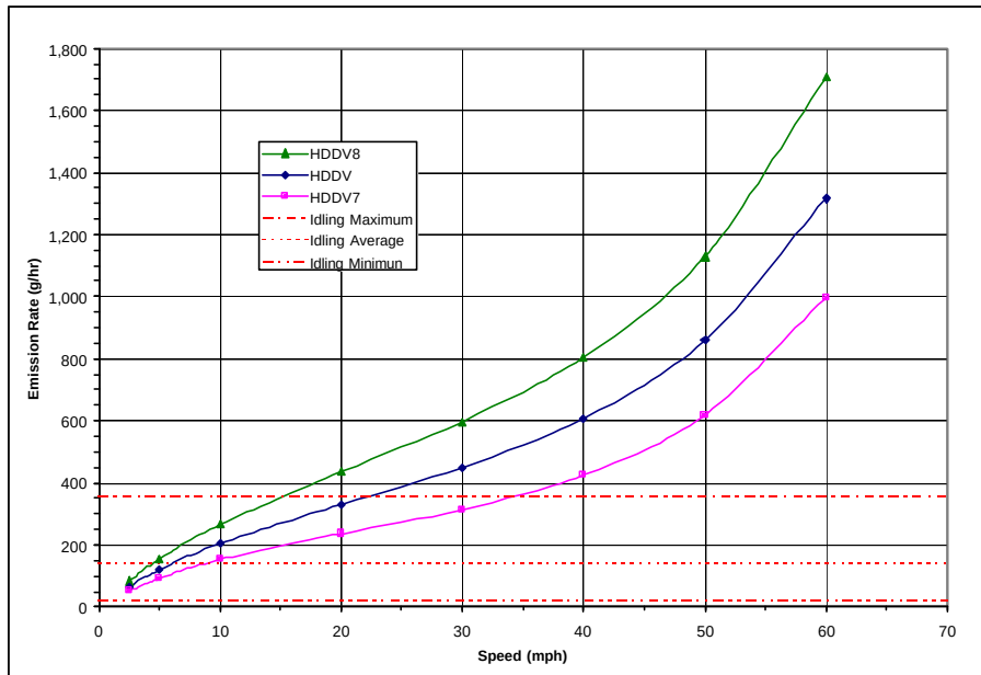
Figure 2.2. MOBILE6 - NOx emission rates as a function of vehicle speed.
