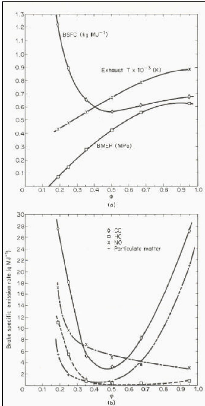
Figure 1.1. Influence of the equivalence ratio ( f ) on light-duty diesel engine performance and emissions.
