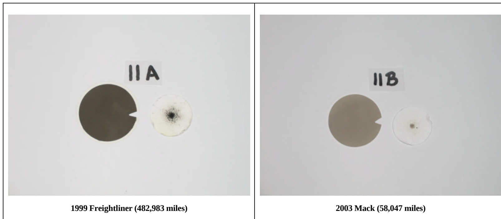
Figure 4.12. Black and gray PM collected on filter media during emission testing.
