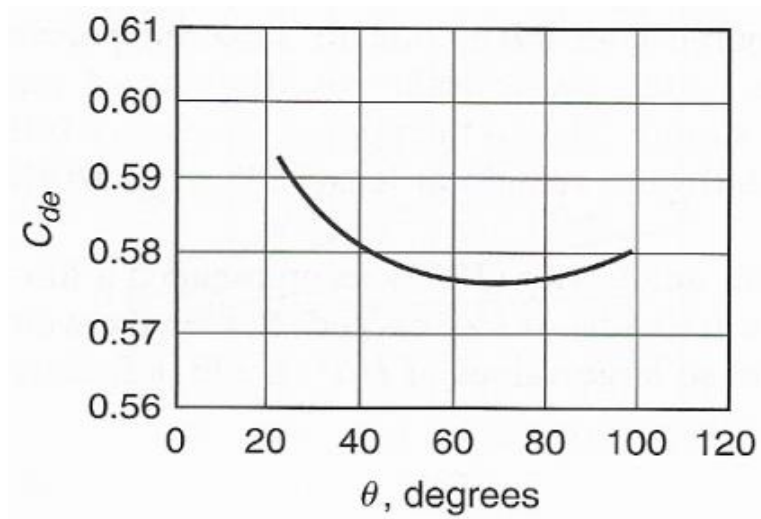
Figure 3-13. Coefficient of discharge for 90-degree V-notch weirs partially contracted flow (Sturm 2010).
