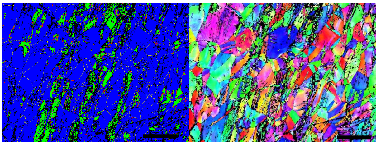
(b) Sample R#411B: center (slightly off to the side). Phase: 75% FCC, 8%hcp, 15%bcc
