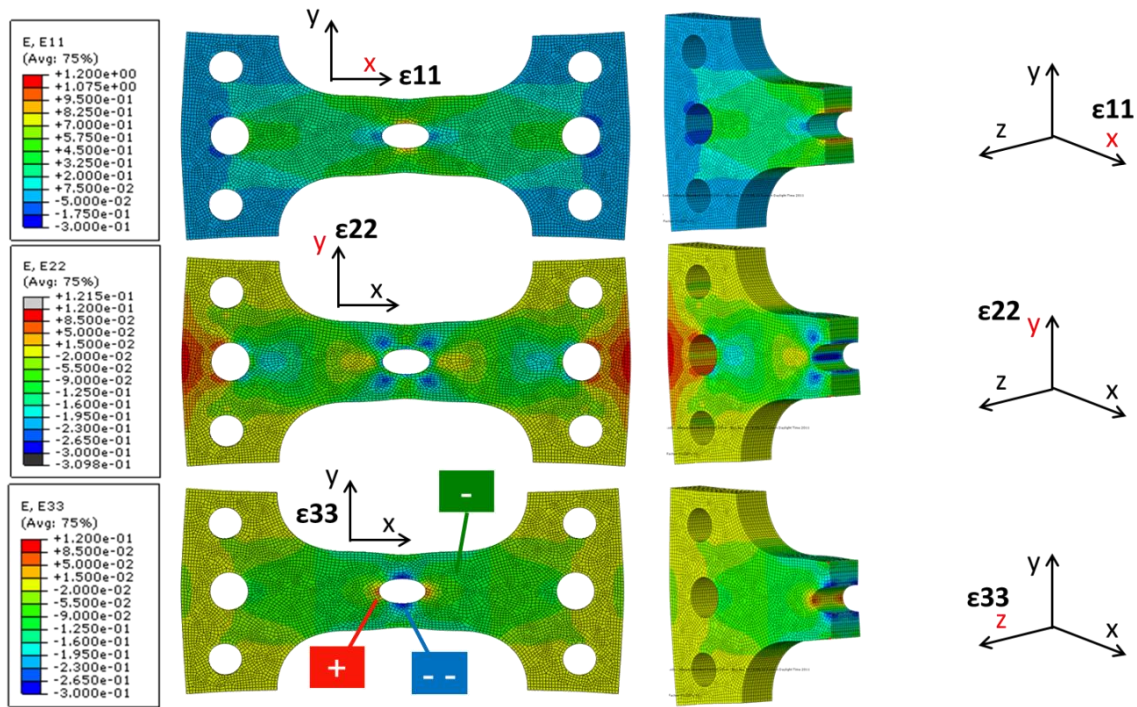
Figure 5-3. Finite Element Model (FEM) and strain state for of the a proposed (thick (9.5 mm)) steel sample geometry. The strain component \epsilon_{33} will be probed during the transmission measurement and varies in the z-direction (along thickness direction) as can be seen.
