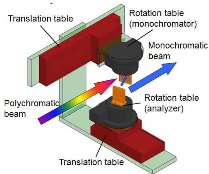
Figure 2-20. Double Crystal Monochromator for CONRAD at HZB.
