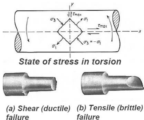
Figure 2-6. Modes of failure in torsion. From ( Dieter 1986 , 6 )
