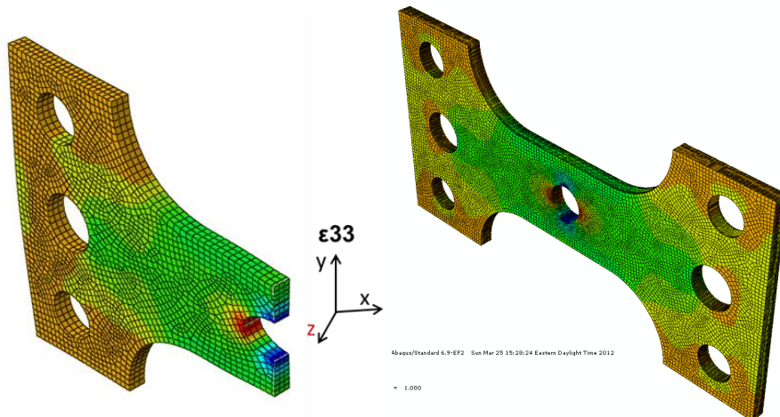
Figure 5-4. Finite Element Model (FEM) and strain state of a thin (3 mm) steel sample. The strain component \epsilon_{33} is relatively uniform in the z-direction.
