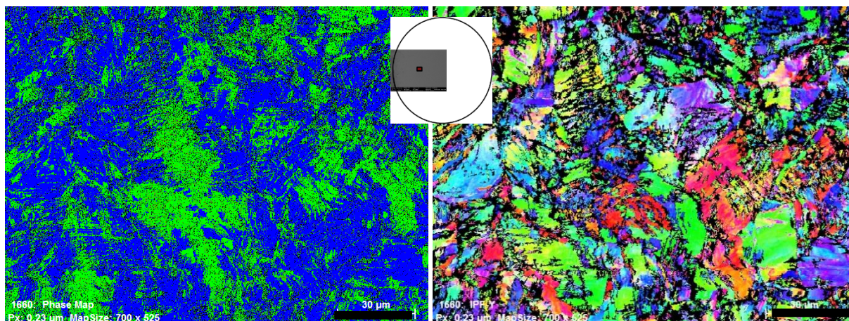
(a) Sample R#410A. Measured towards side of the sample (not precisely defined).
