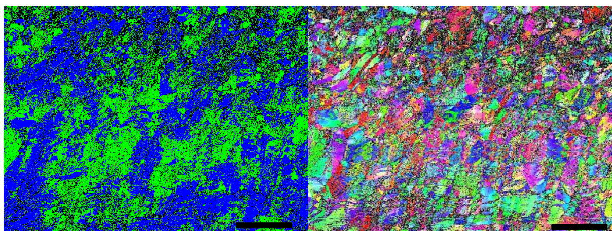
(c) Sample R#411B: 2mm from the center. Phase: 45% FCC, 15%hcp, 39%bcc
