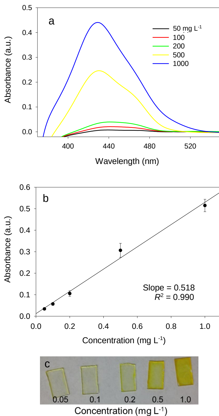
Figure 3.2. (a) Visible spectra of probe exposed to aniline. (b) Calibration plot for aniline concentrations. (c) Probe response to different aniline concentrations.
