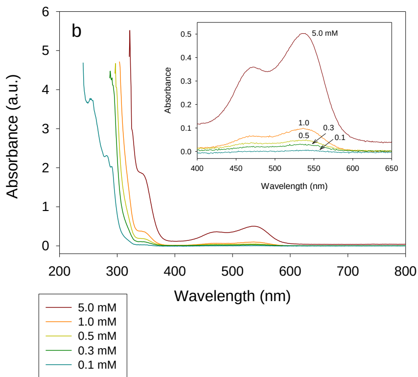
Figure 4.1. (a) Calibration plot of \beta -bis(indolyl)methane. (b) UV-visible spectra of \beta -bis(indolyl)methane in 95% ethanol.
