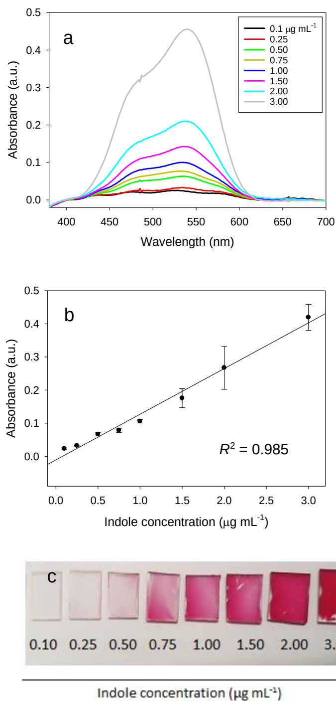
Figure 2.2. (a) Visible spectra of the probe showing response to increasing indole concentrations. (b) Calibration plot using the absorbance at 540 nm. (c) Photos of the probe to 0.1-3.0 \mu\text{g mL}^{-1} indole solutions.
